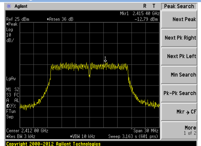
802.11g CHANNEL 1
