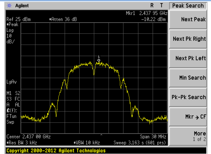
802.11b CHANNEL 6
