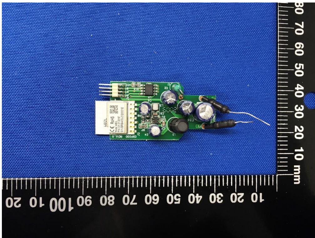
MAIN BOARD REAR VIEW (EBE-QPW70 &amp; EBE-QPW70-B)
