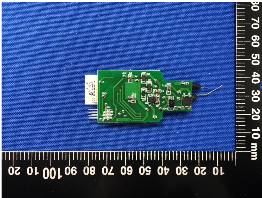
MAIN BOARD TOP VIEW (EBE-QPW70 &amp; EBE-QPW70-B)
