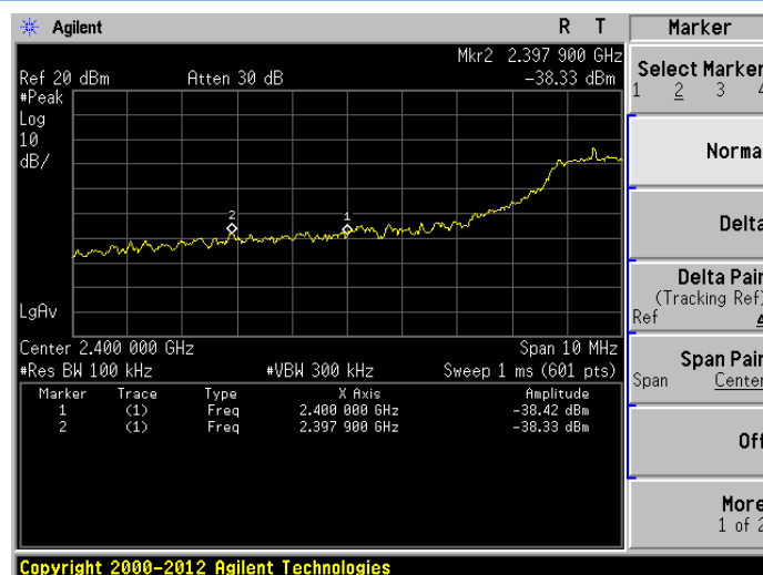
802.11g LOW CHANNEL 1, Reference level
