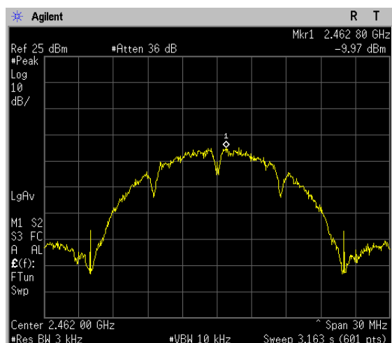
802.11b CHANNEL 11
