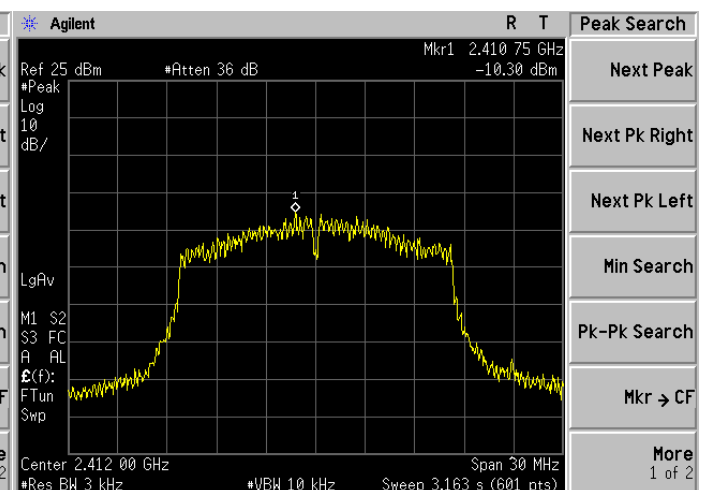
802.11g CHANNEL 1
