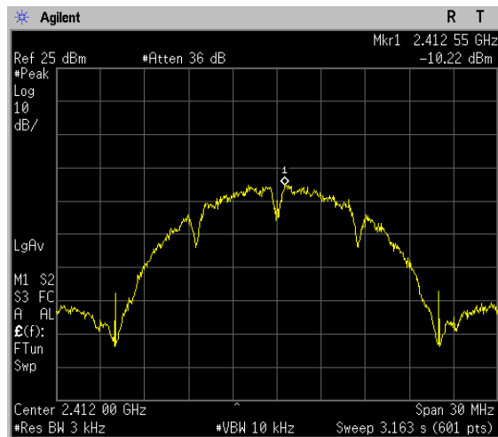
802.11b CHANNEL 1
