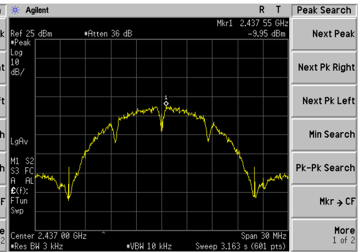
802.11b CHANNEL 6
