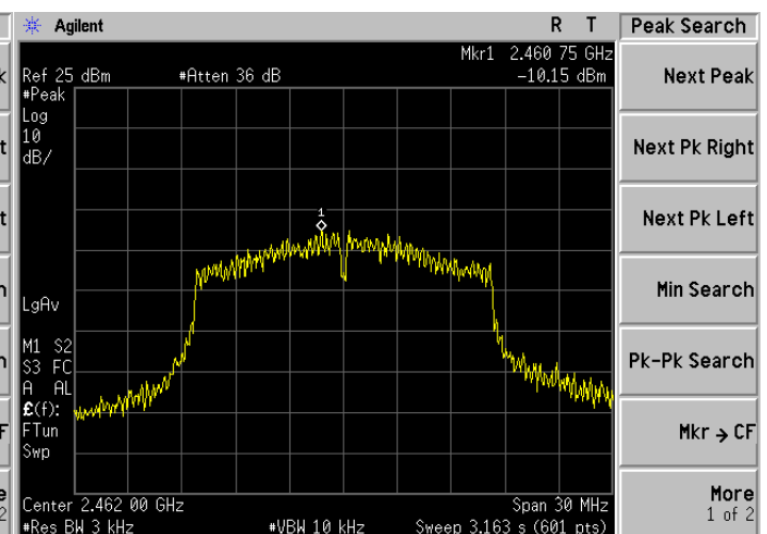
802.11g CHANNEL 11
