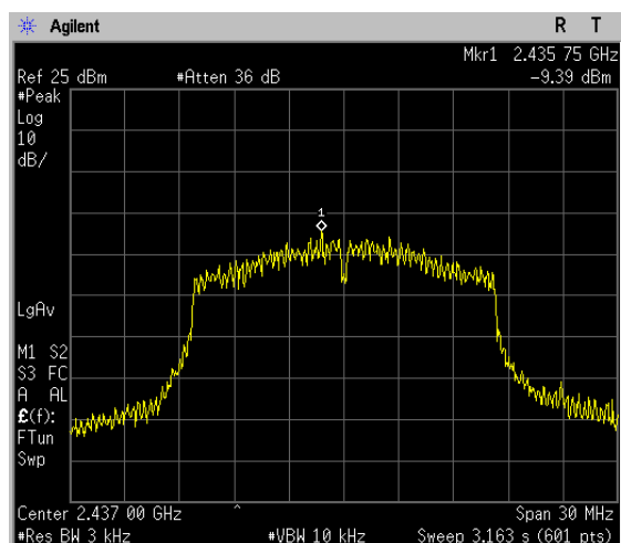
802.11g CHANNEL 6
