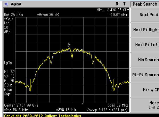
802.11b CHANNEL 6
