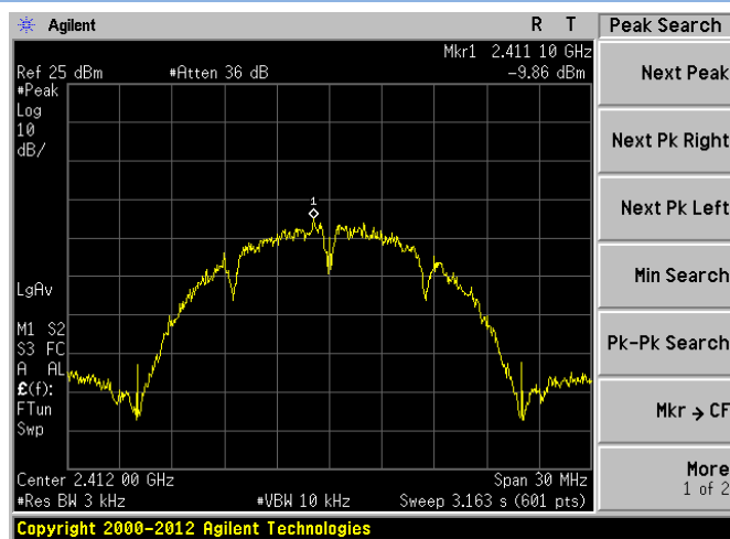
802.11b CHANNEL 1
