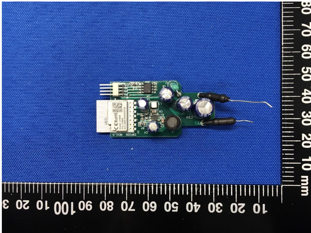
MAIN BOARD REAR VIEW (EBE-QPW113)
