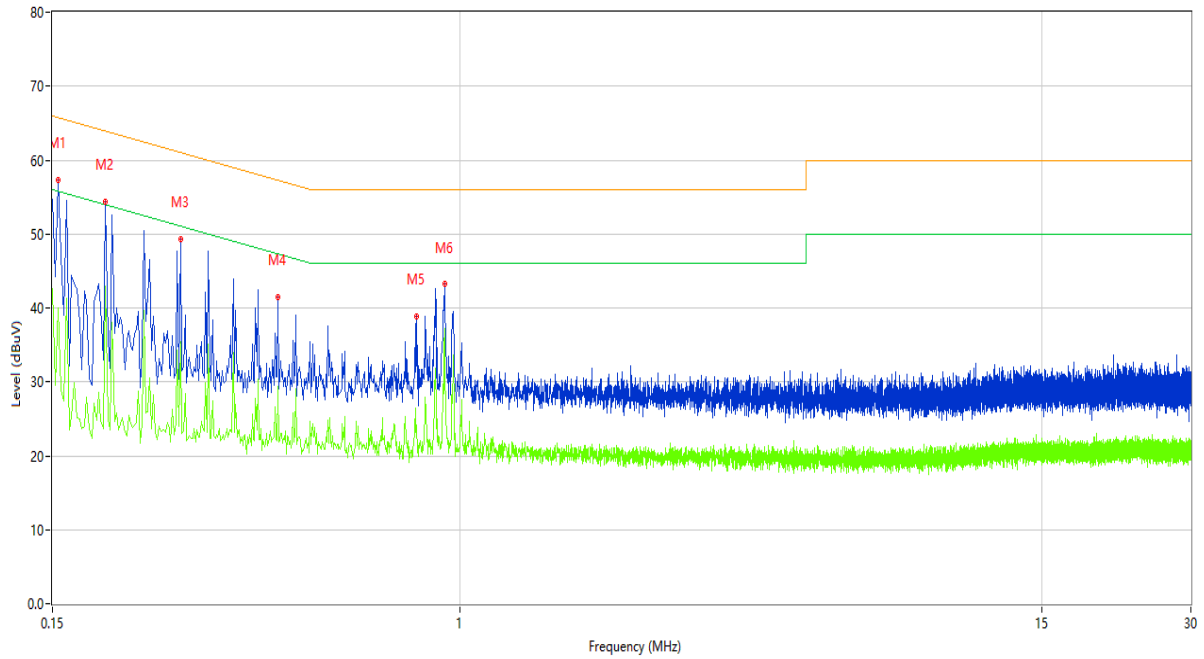
PHASE L
