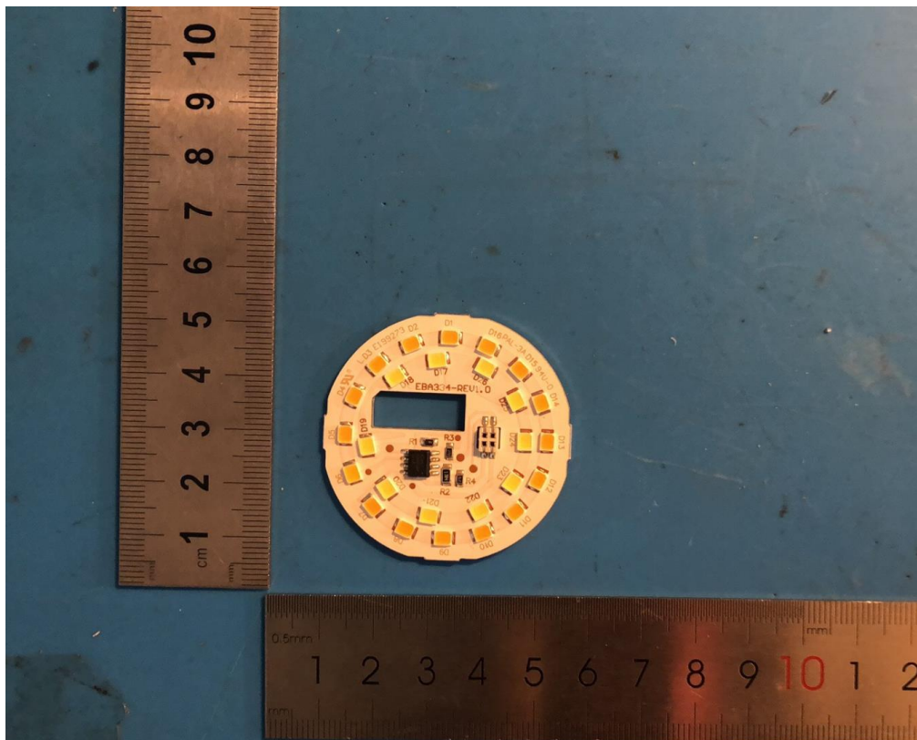
MAIN BOARD TOP VIEW (EBE-QPW112)
