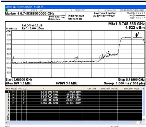
802.11n20-5745MHz-Lower(Peak)
