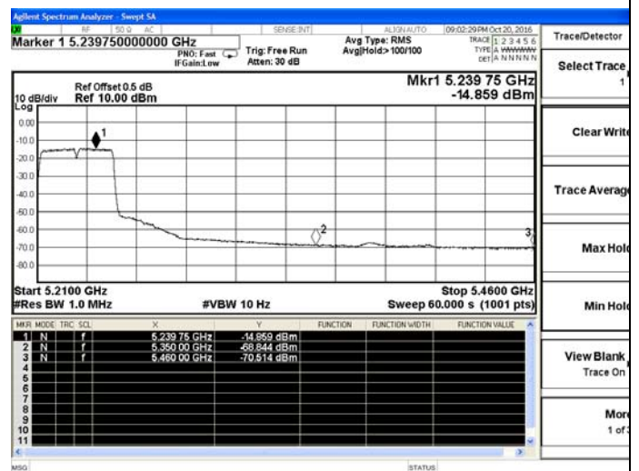
802.11n20-5240MHz-Upper(Average)
