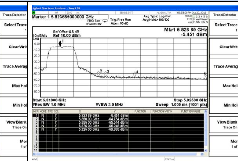
802.11a-5825MHz-Upper(Peak)
