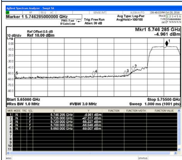
802.11a-5745MHz-Lower(Peak)
