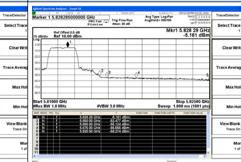
802.11n20-5825MHz-Upper(Peak)
