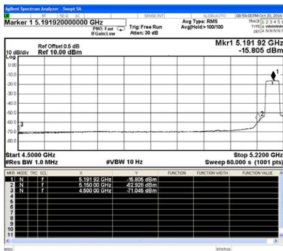
802.11n20-5180MHz-Lower(Average)
