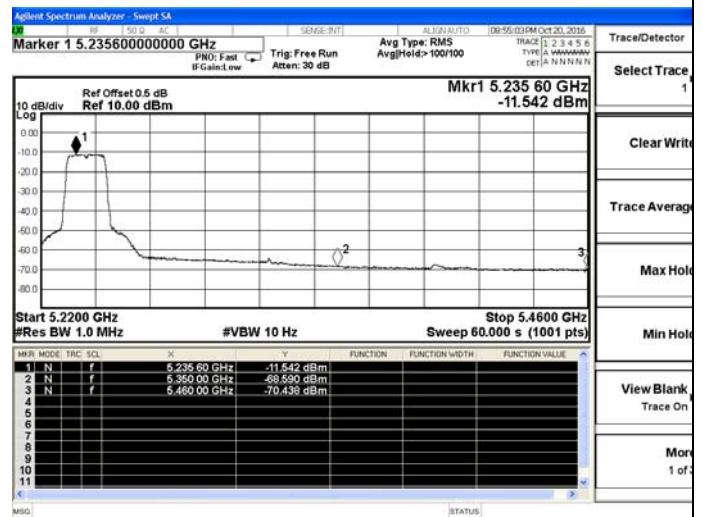
802.11a-5240MHz-Upper(Average)
