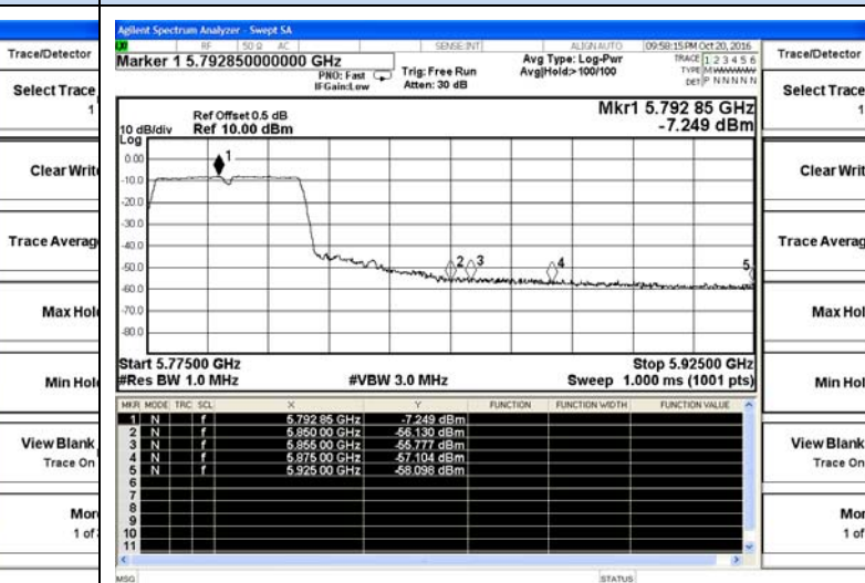
802.11n40-5795MHz-Upper(Peak)
