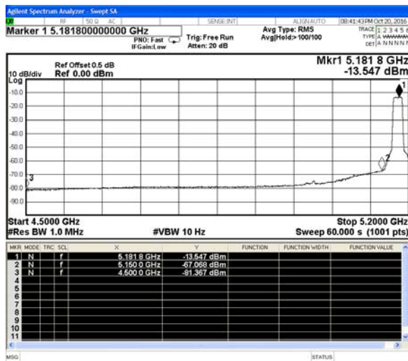
802.11a-5180MHz-Lower(Average)
