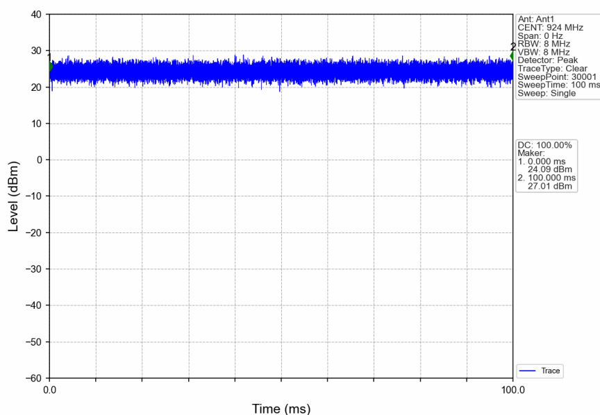
8M_HCH_924MHz_Ant1_NTNV
