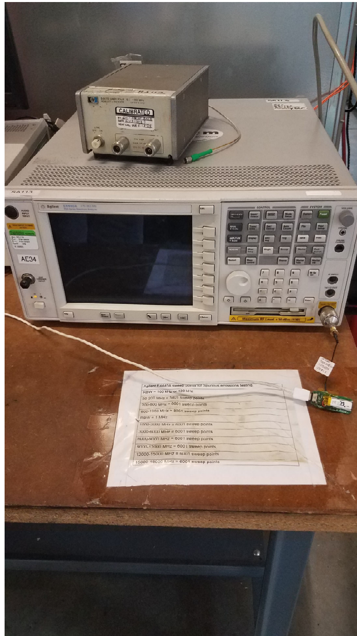
Figure 5. Radio Bench testing, FCC/ISED
