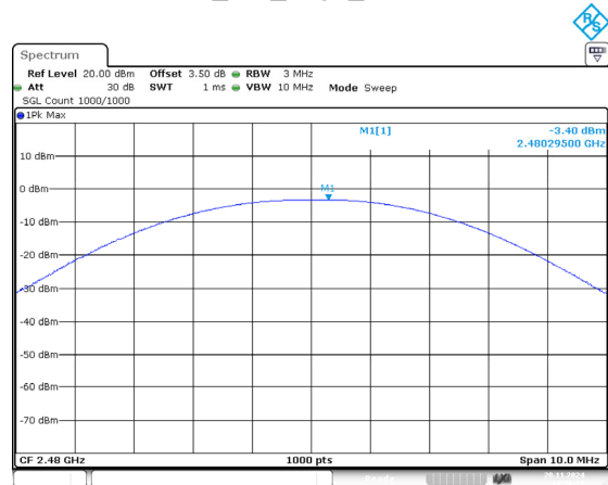
BLE_1M_High_Channel
