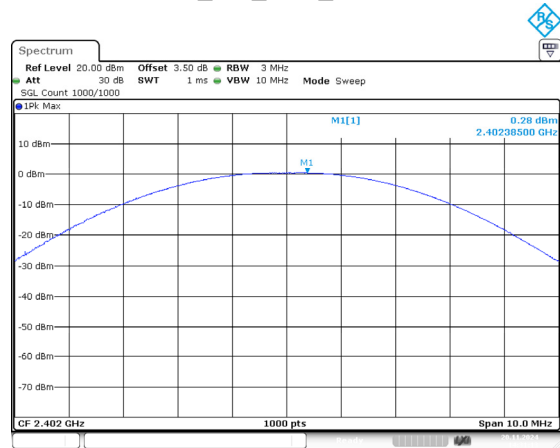
BLE_1M_Low_Channel
