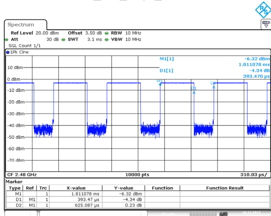
BLE_1M_High_Channel
