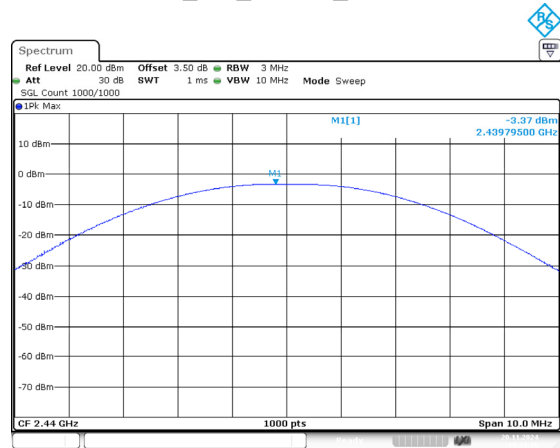
BLE_1M_Middle_Channel
