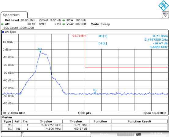
BLE_1M_High_Channel
