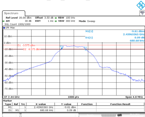
BLE_1M_Middle_Channel
