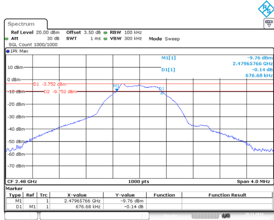
BLE_1M_High_Channel
