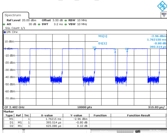
BLE_1M_Low_Channel
