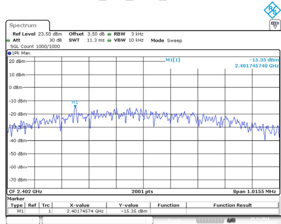
BLE_1M_Low_Channel
