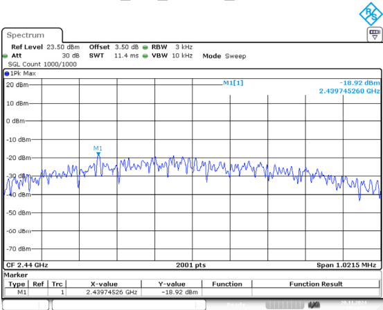
BLE_1M_Middle_Channel
