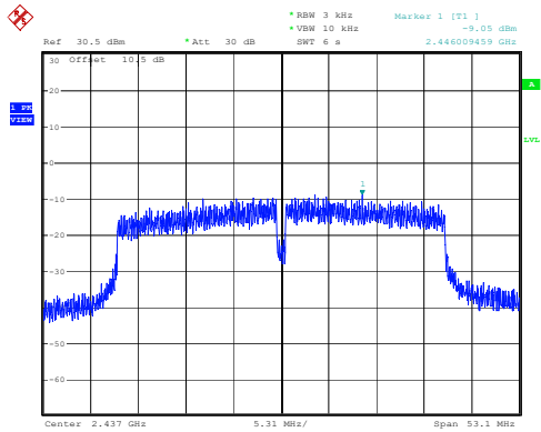
802.11n40_2437MHz
