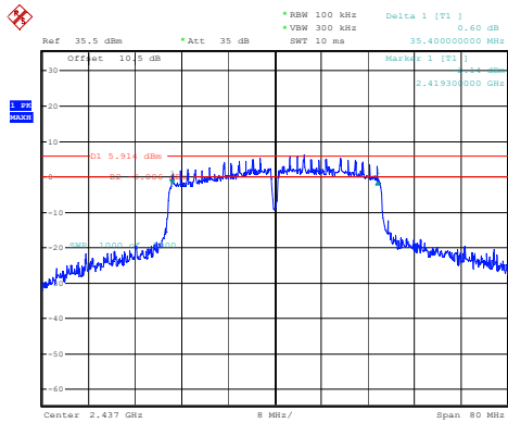
802.11n40_2437MHz
