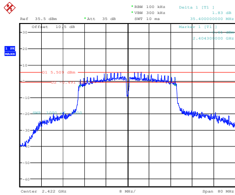
802.11n40_2422MHz
