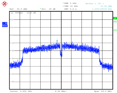
802.11n40_2452MHz
