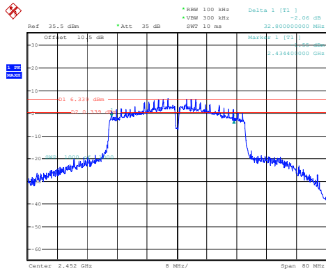
802.11n40_2452MHz
