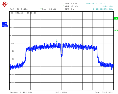
802.11n40_2422MHz
