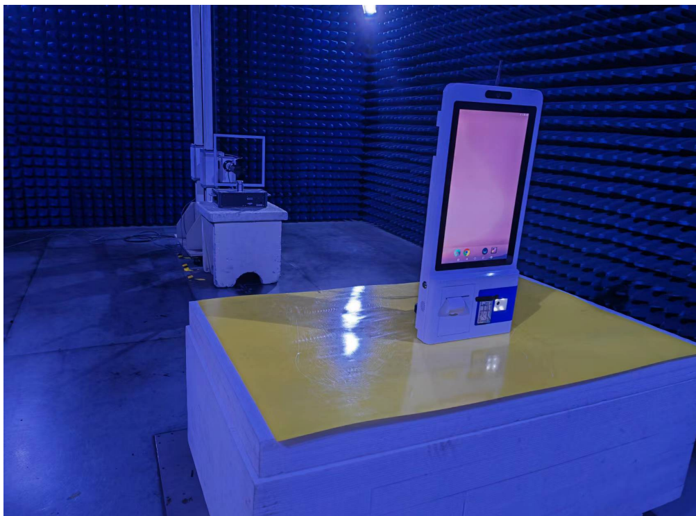
Photo of Radiated Emission Measurement (9kHz-30MHz)
