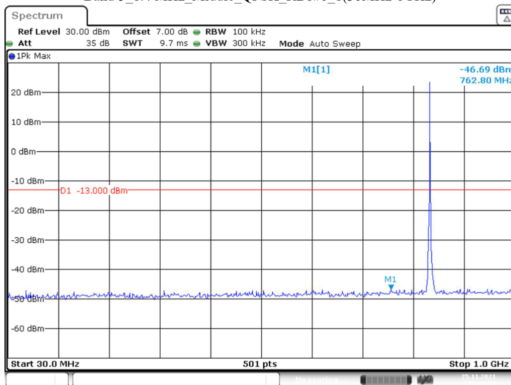
Band 5 1.4 MHz Middle QPSK RB6#0 1(30MHz-1GHz)
