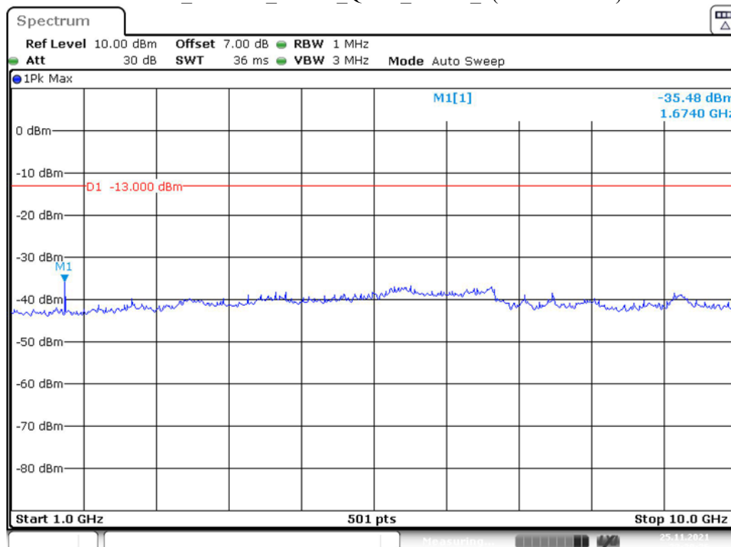
Band 5 1.4 MHz Middle QPSK RB6#0 2(1GHz-10GHz)
