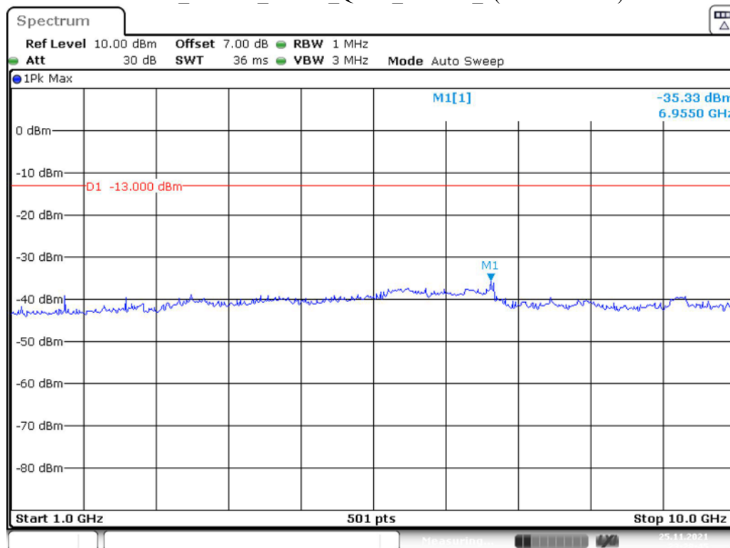
Band 5_10 MHz_Middle_QPSK_RB50#0_2(1GHz-10GHz)
