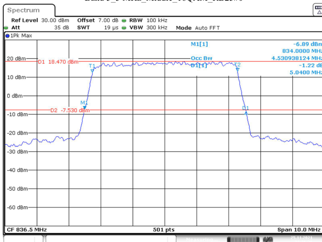
Band 5 5 MHz Middle 16QAM RB25#0
