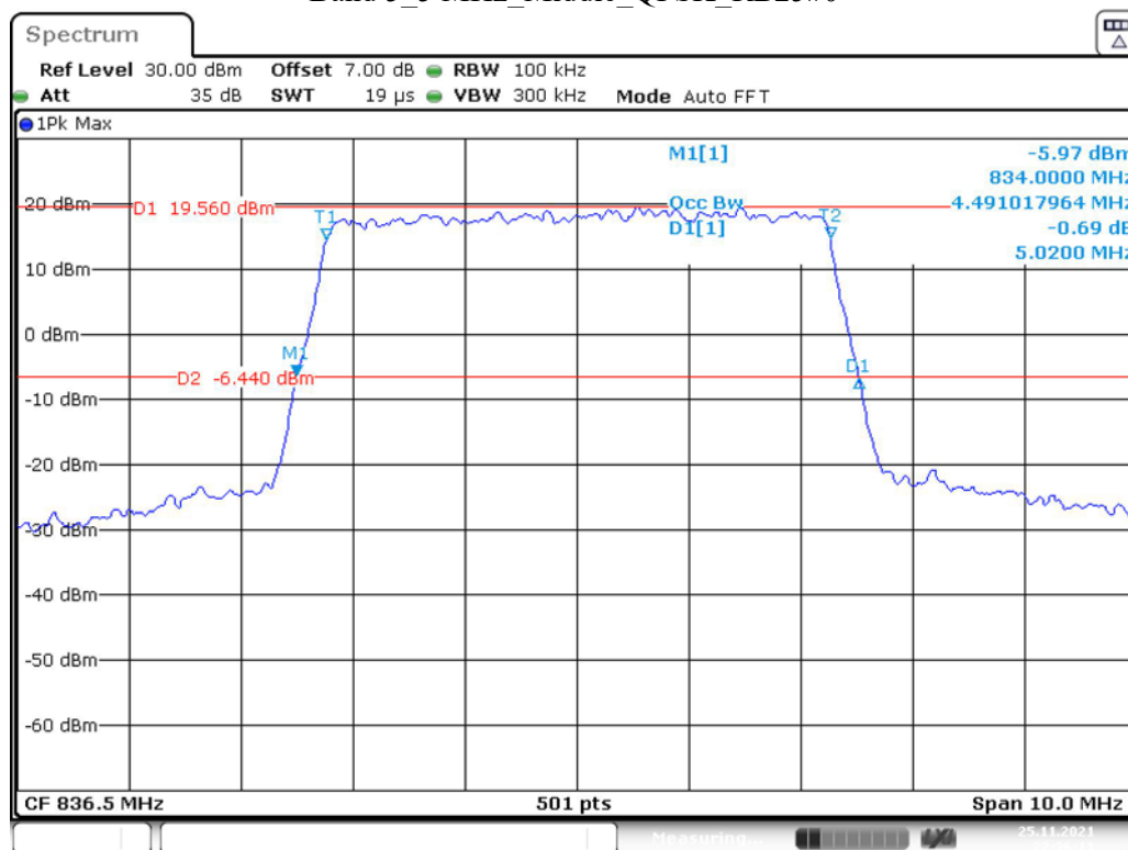
Band 5 5 MHz Middle QPSK RB25#0
