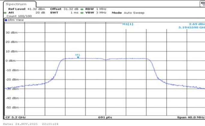
11AC20SISO Ant1 5200
