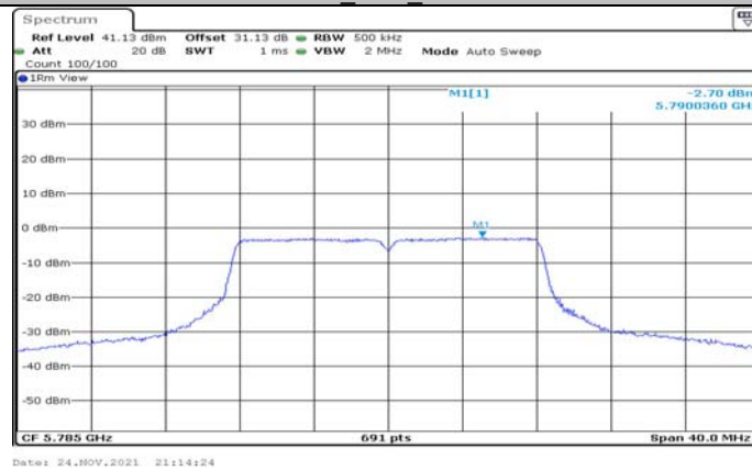
11A_Ant1_5785
