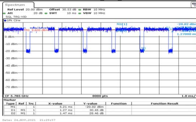
11N20SISO Ant1 5785
