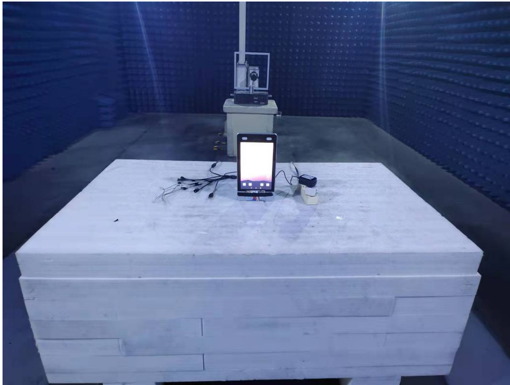
Photo of Radiated Emission Measurement (9kHz-30MHz) Coaxial view
