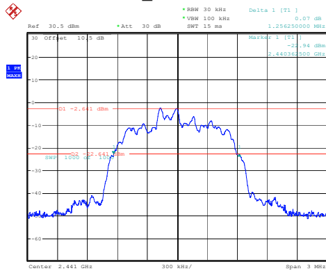
2DH1_Middle 1.256MHz
