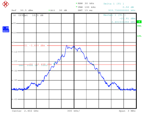
DH1_Low 0.934MHz
