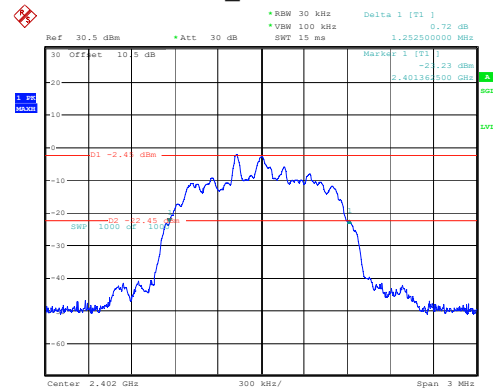
2DH1_Low 1.252MHz
