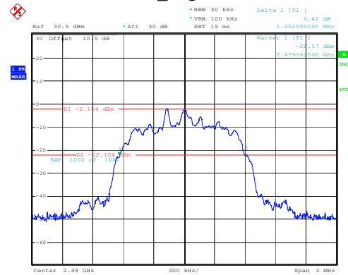
2DH1_High 1.252MHz
