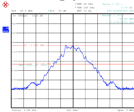
DH1_High 0.945MHz
