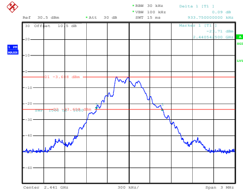
DH1_Middle 0.934MHz
