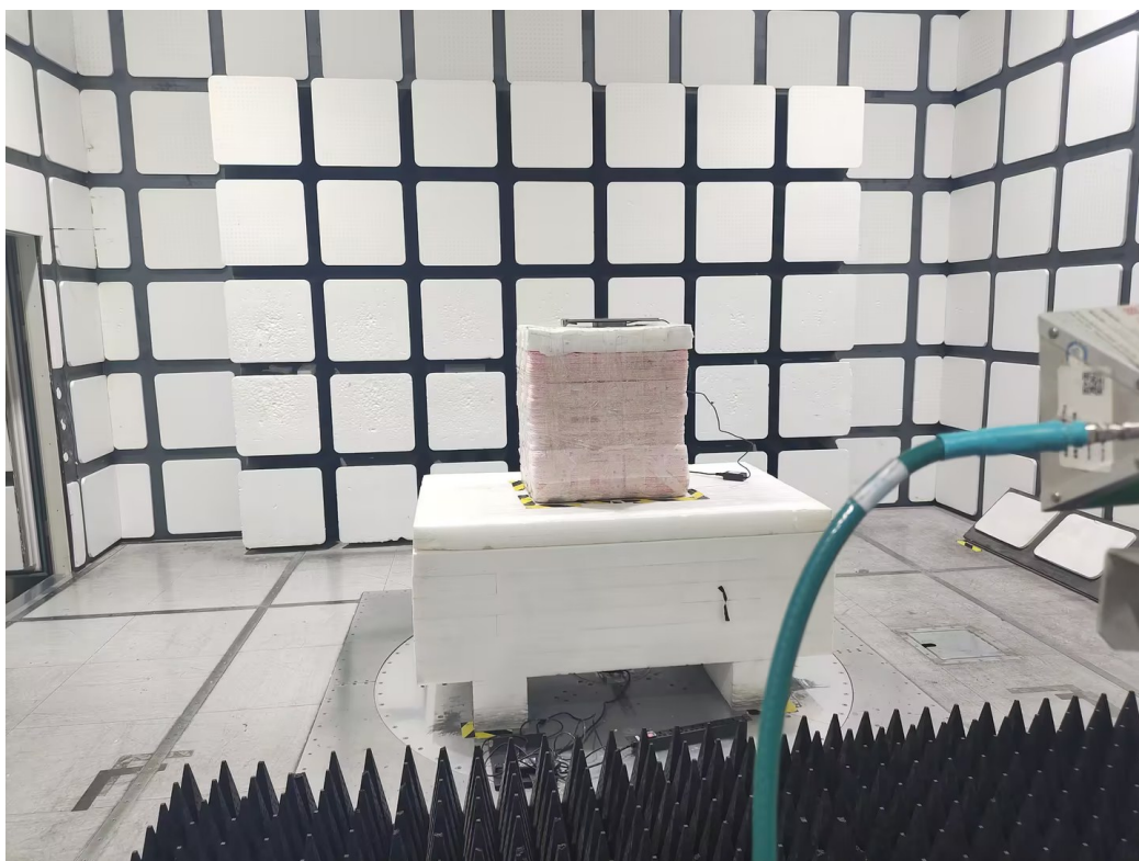
Radiated Emissions View (18-25 GHz)
