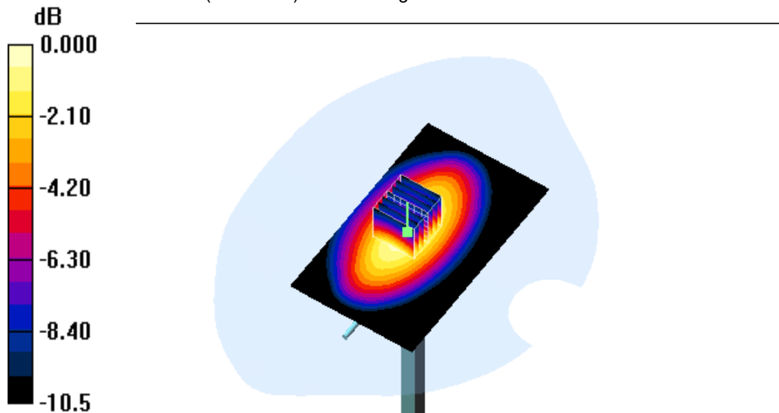
System Performance Check 835MHz Body 1000mW
