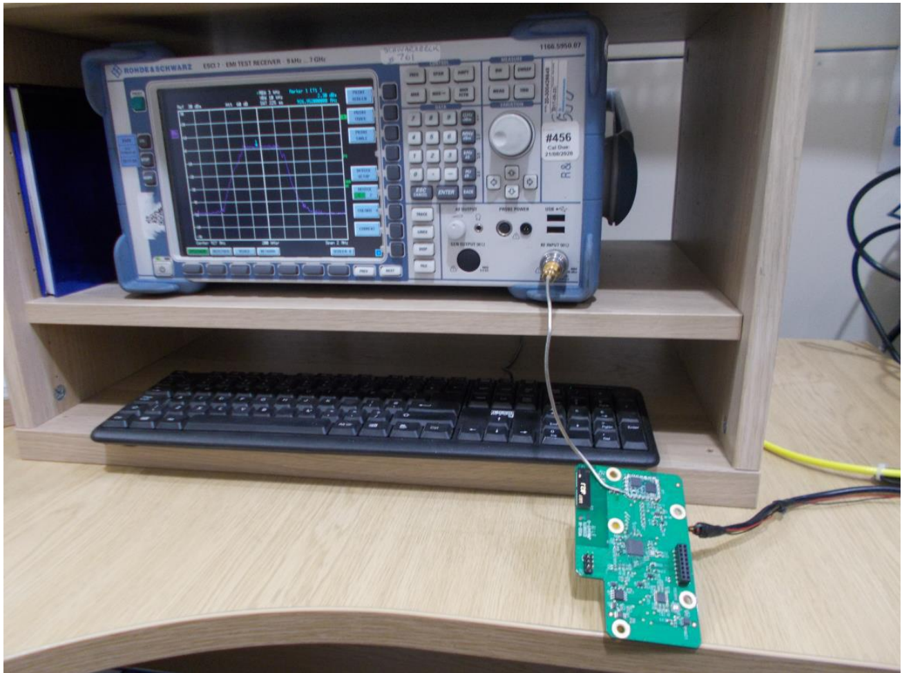
Figure 3. Conducted Measurements
