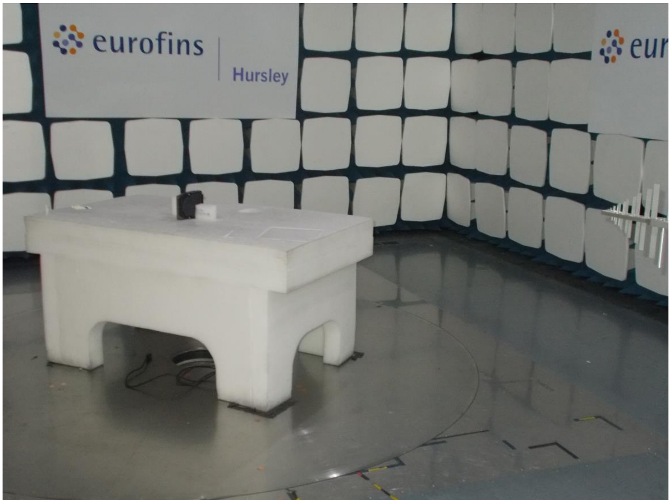
Figure 1. Radiated Emissions <1GHz
