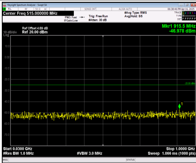
Band41-20MHz-QPSK-40620-1RB#0-Range1:30~1000MHz
