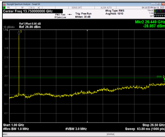
Band38-5MHz-64QAM-38225-1RB#0-Range2:1000~26500MHz
