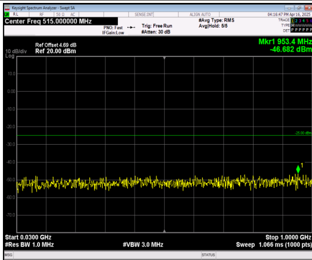
Band38-5MHz-64QAM-38225-1RB#0-Range1:30~1000MHz
