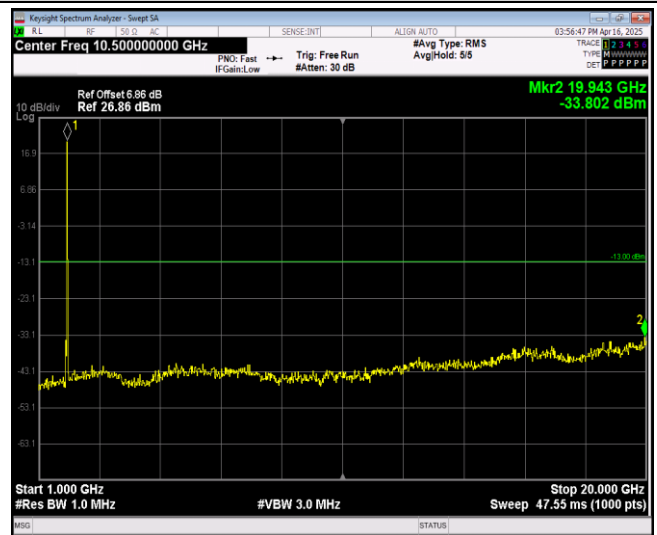
Band25-20MHz-16QAM-26140-1RB#0-Range2:1000~20000MHz
