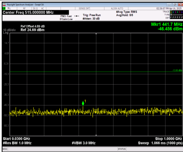
Band25-1.4MHz-QPSK-26365-1RB#0-Range1:30~1000MHz
