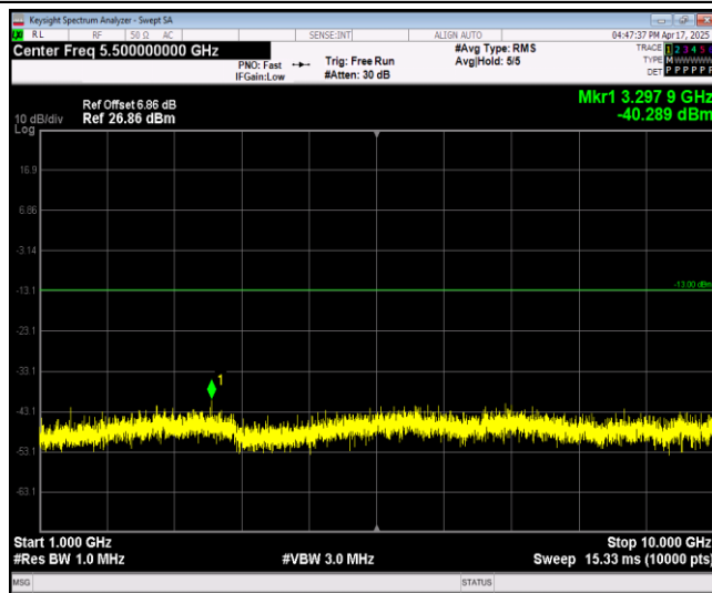
Band17-5MHz-16QAM-23825-1RB#0-Range2:1000~10000MHz
