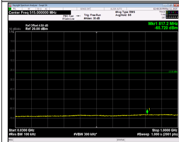
66-66-20MHz-20MHz-16QAM-16QAM-132374-132572-1 RB#99-ORB#0-30~1000MHz-PASS
