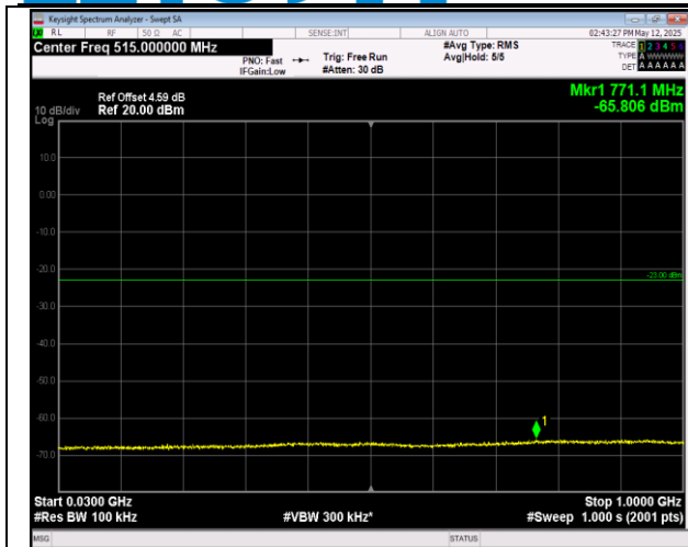
66-66-20MHz-20MHz-16QAM-16QAM-132323-132521-1 RB#99-ORB#0-30~1000MHz-PASS
