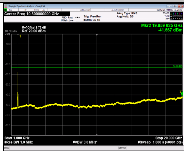
66-66-20MHz-20MHz-16QAM-16QAM-132323-132521-100 RB#0-100RB#0-1000~20000MHz-PASS
