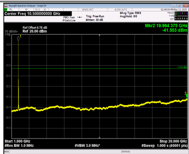
66-66-20MHz-20MHz-16QAM-16QAM-132374-132572-1RB #99-ORB#0-1000~20000MHz-PASS
