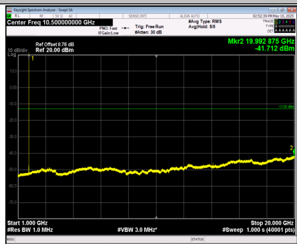
66-66-5MHz-20MHz-16QAM-16QAM-132455-132572-1RB# 0-1RB#99-1000~20000MHz-PASS
