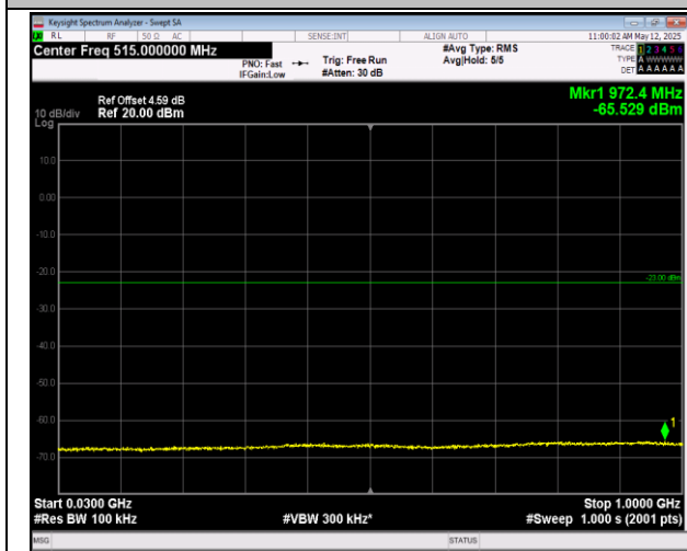
66-66-20MHz-5MHz-16QAM-16QAM-132397-132514-10 ORB#0-25RB#0-30~1000MHz-PASS
