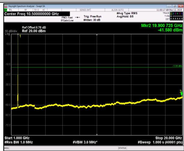
66-66-20MHz-5MHz-16QAM-16QAM-132397-132514-100R B#0-25RB#0-1000~20000MHz-PASS
