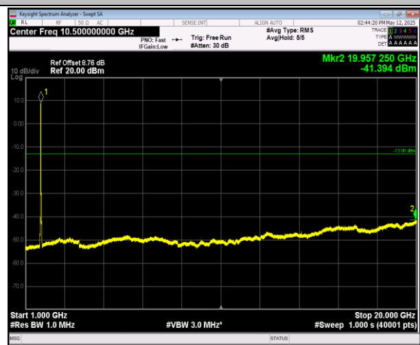
66-66-20MHz-20MHz-16QAM-16QAM-132323-132521-1RB #0-0RB#0-1000~20000MHz-PASS
