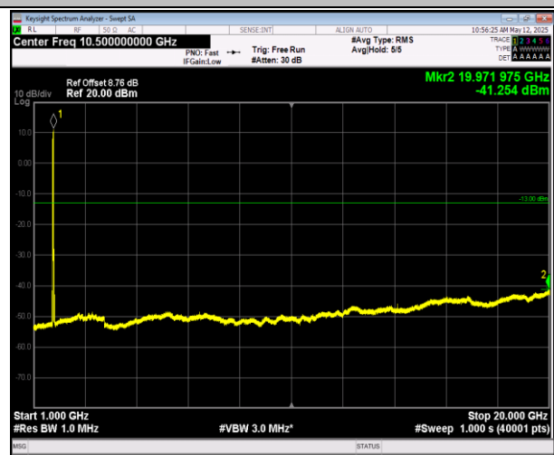
66-66-20MHz-5MHz-16QAM-16QAM-132072-132189-1RB# 99-0RB#0-1000~20000MHz-PASS
