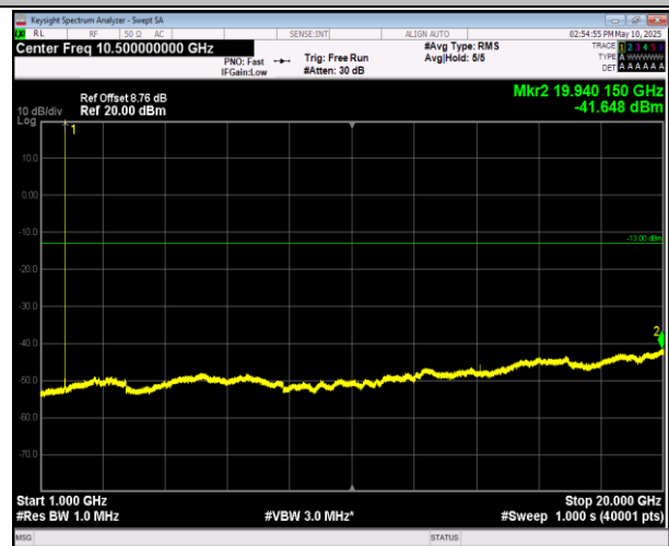
66-66-5MHz-20MHz-16QAM-16QAM-132455-132572-1RB# 24-0RB#0-1000~20000MHz-PASS
