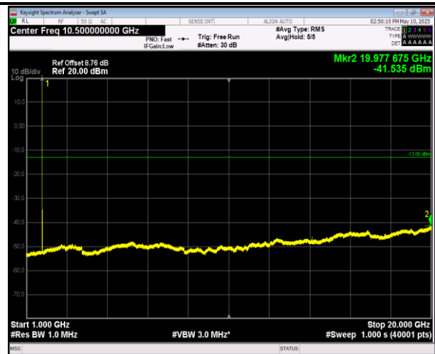
66-66-5MHz-20MHz-16QAM-16QAM-132330-132447-1RB# 24-ORB#0-1000~20000MHz-PASS
