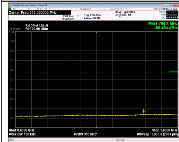
66-66-20MHz-5MHz-16QAM-16QAM-132072-132189-10 ORB#0-25RB#0-30~1000MHz-PASS
