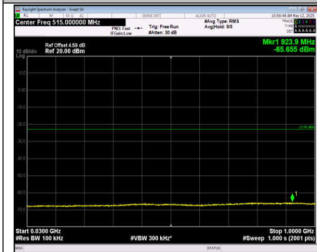
66-66-20MHz-5MHz-16QAM-16QAM-132072-132189-1RB# B#0-ORB#0-30~1000MHz-PASS
