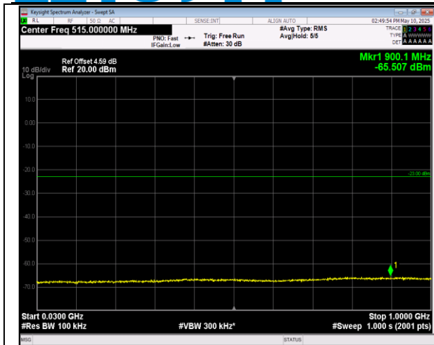
66-66-5MHz-20MHz-16QAM-16QAM-132330-132447-1R B#24-ORB#0-30~1000MHz-PASS
