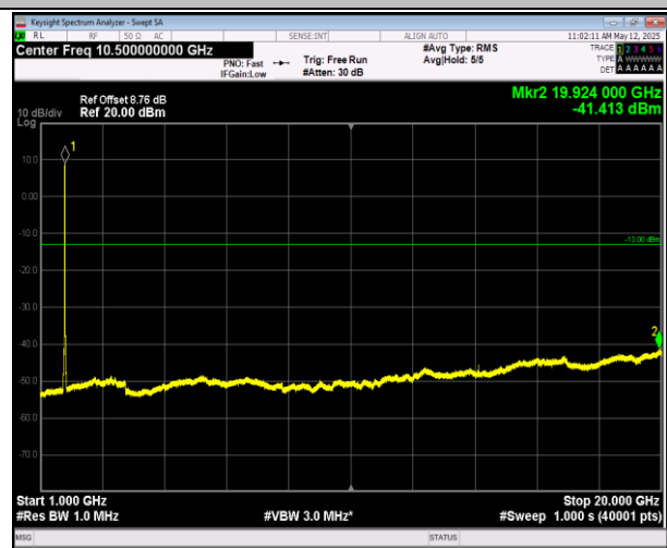
66-66-20MHz-5MHz-16QAM-16QAM-132397-132514-1RB# 0-0RB#0-1000~20000MHz-PASS
