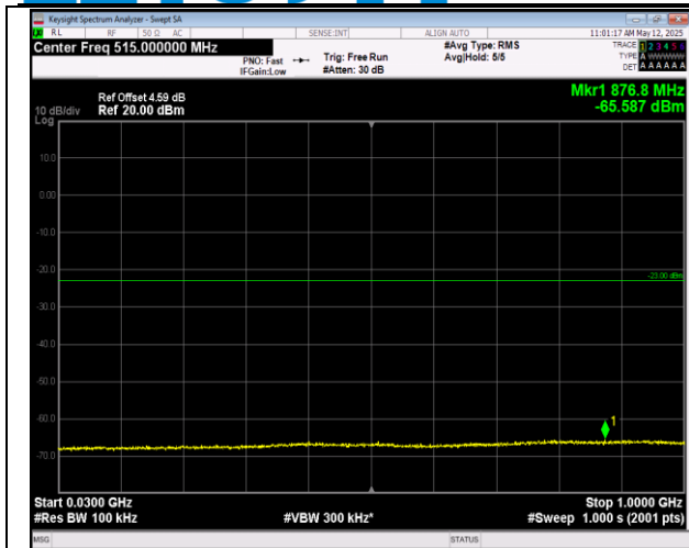
66-66-20MHz-5MHz-16QAM-16QAM-132397-132514-1R B#99-ORB#0-30~1000MHz-PASS
