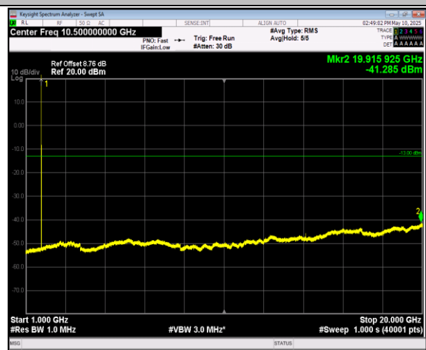
66-66-5MHz-20MHz-16QAM-16QAM-132330-132447-25RB #0-100RB#0-1000~20000MHz-PASS
