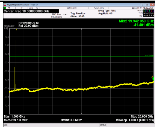
66-66-20MHz-5MHz-16QAM-16QAM-132072-132189-100R B#0-25RB#0-1000~20000MHz-PASS
