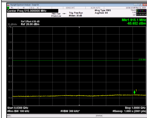
66-66-20MHz-5MHz-16QAM-16QAM-132072-132189-1R B#99-0RB#0-30~1000MHz-PASS
