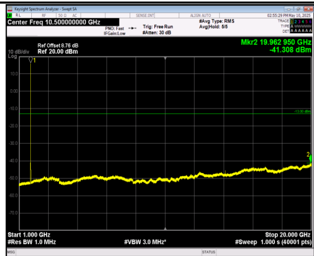
66-66-5MHz-20MHz-16QAM-16QAM-132455-132572-1RB# 0-0RB#0-1000~20000MHz-PASS
