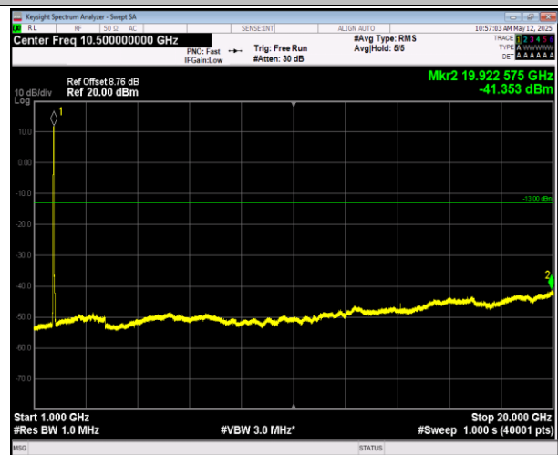
66-66-20MHz-5MHz-16QAM-16QAM-132072-132189-1RB# 0-ORB#0-1000~20000MHz-PASS
