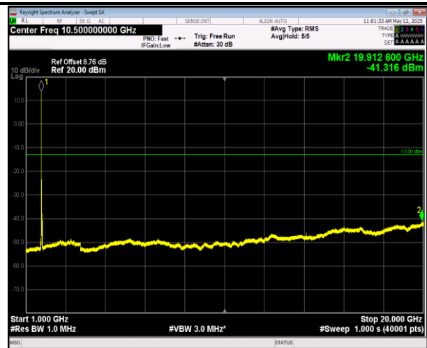
66-66-20MHz-5MHz-16QAM-16QAM-132397-132514-1RB# 99-ORB#0-1000~20000MHz-PASS
