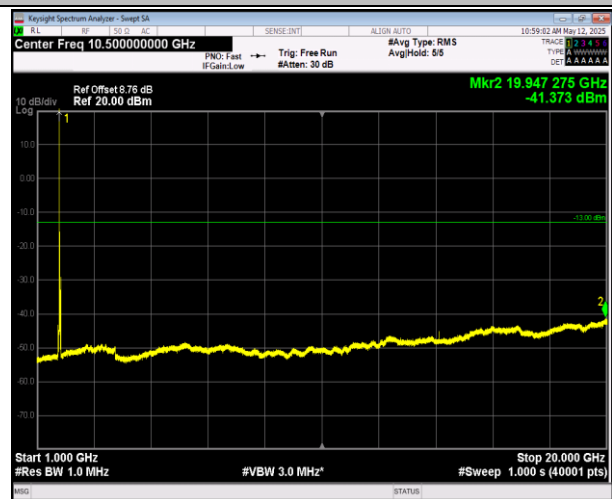
66-66-20MHz-5MHz-16QAM-16QAM-132397-132514-1RB# 0-1RB#24-1000~20000MHz-PASS
