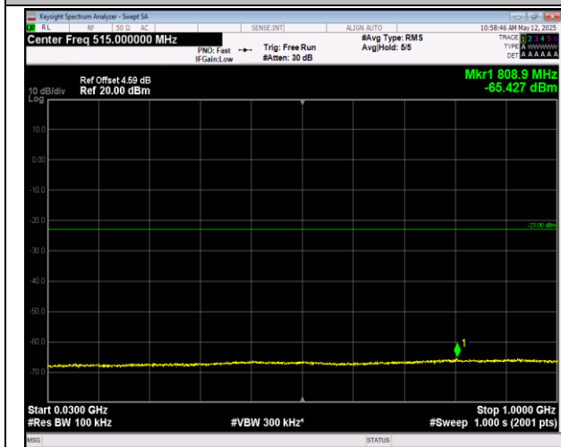
66-66-20MHz-5MHz-16QAM-16QAM-132397-132514-1R B#0-1RB#24-30~1000MHz-PASS
