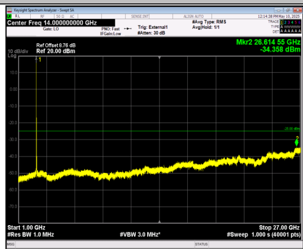
41-41-20MHz-10MHz-16QAM-16QAM-41391-41535-1RB#0 -1RB#49-1000~27000MHz-PASS
