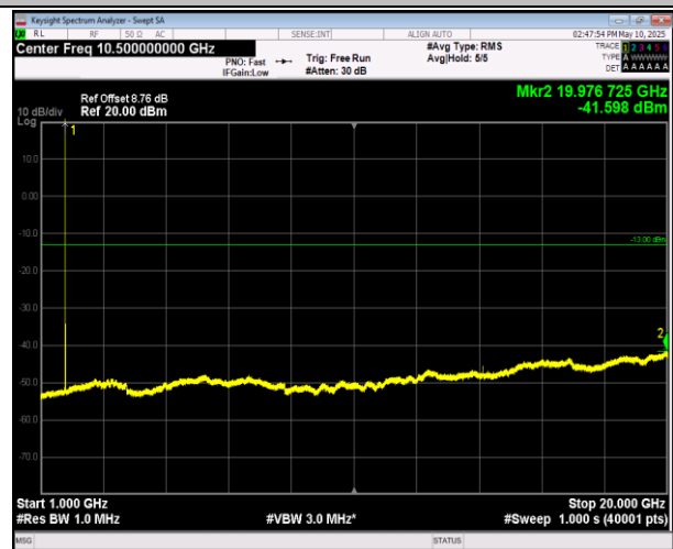
66-66-5MHz-20MHz-16QAM-16QAM-132330-132447-1RB# 0-1RB#99-1000~20000MHz-PASS
