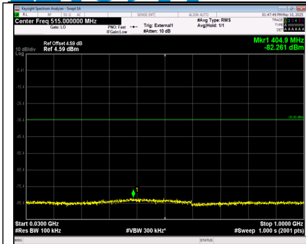
41-41-20MHz-20MHz-16QAM-16QAM-40521-40719-1RB #99-0RB#0-30~1000MHz-PASS
