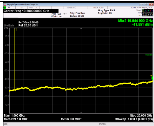
66-66-5MHz-20MHz-16QAM-16QAM-132005-132122-1RB# 0-1RB#99-1000~20000MHz-PASS
