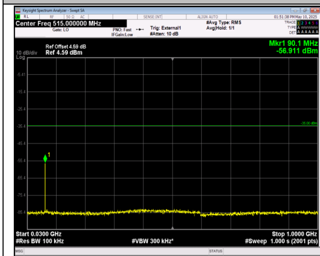
41-41-20MHz-20MHz-16QAM-16QAM-41292-41490-1RB #0-1RB#99-30~1000MHz-PASS
