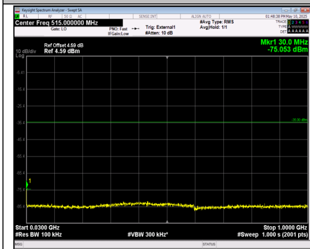
41-41-20MHz-20MHz-16QAM-16QAM-40521-40719-1RB #0-0RB#0-30~1000MHz-PASS
