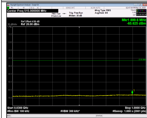
66-66-5MHz-20MHz-QPSK-QPSK-132330-132447-1RB# 0-1RB#99-30~1000MHz-PASS
