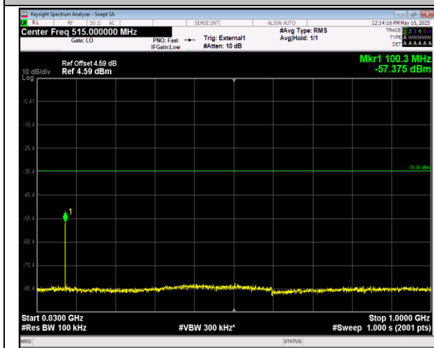
41-41-20MHz-10MHz-16QAM-16QAM-41391-41535-1RB #0-1RB#49-30~1000MHz-PASS
