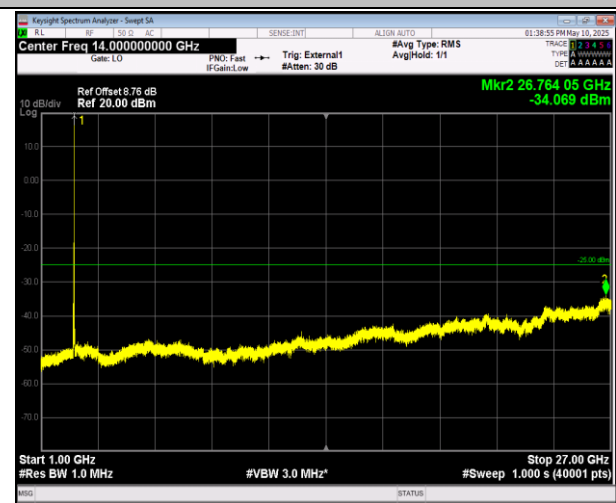
41-41-20MHz-20MHz-QPSK-QPSK-39750-39948-100RB#0 -100RB#0-1000~27000MHz-PASS
