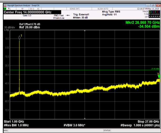
41-41-20MHz-20MHz-QPSK-QPSK-39750-39948-1RB#0-0 RB#0-1000~27000MHz-PASS
