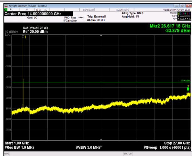
41-41-20MHz-20MHz-16QAM-16QAM-41292-41490-1RB#9 9-ORB#0-1000~27000MHz-PASS
