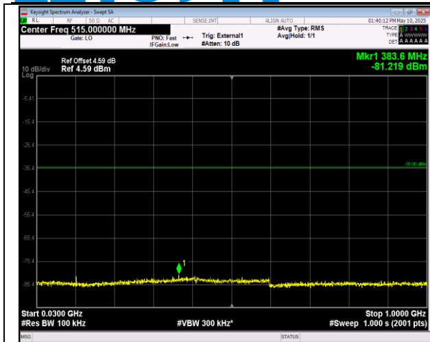
41-41-20MHz-20MHz-QPSK-QPSK-39750-39948-1RB#9 9-ORB#0-30~1000MHz-PASS
