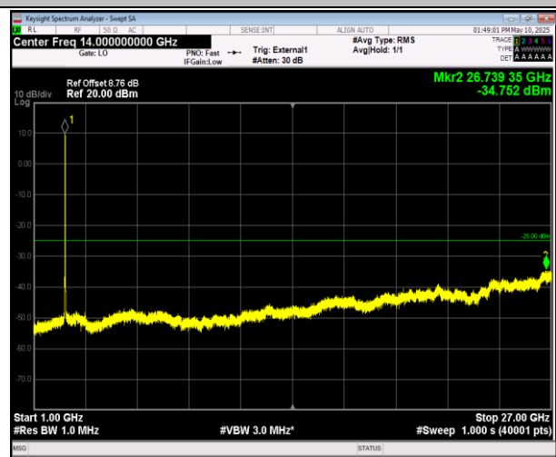
41-41-20MHz-20MHz-16QAM-16QAM-40521-40719-1RB#0 -0RB#0-1000~27000MHz-PASS
