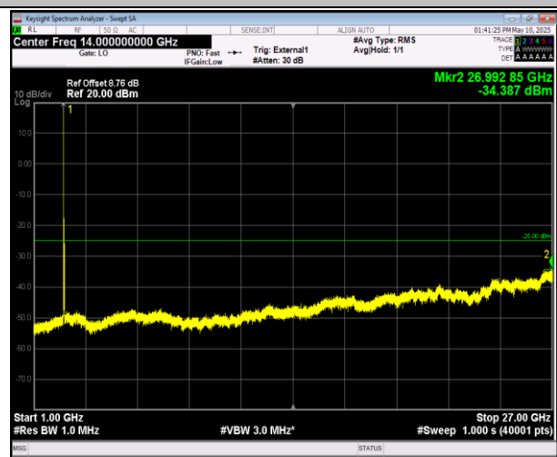
41-41-20MHz-20MHz-16QAM-16QAM-39750-39948-1RB#9 9-0RB#0-1000~27000MHz-PASS
