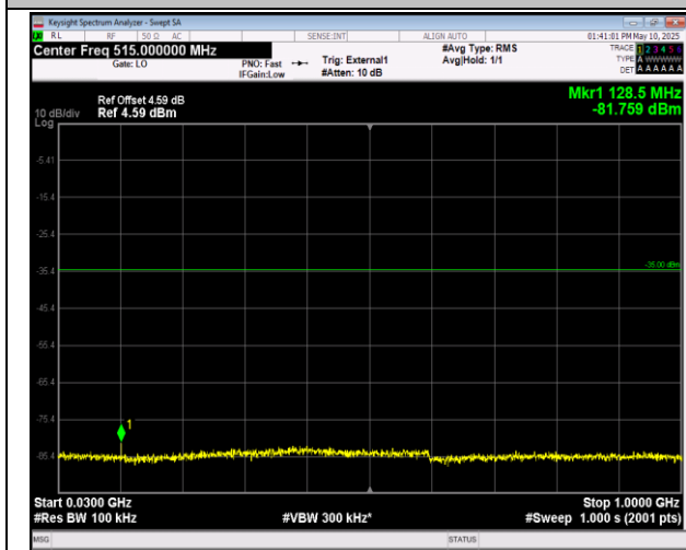
41-41-20MHz-20MHz-16QAM-16QAM-39750-39948-1RB #99-0RB#0-30~1000MHz-PASS
