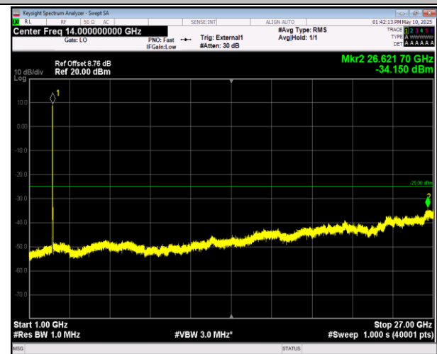
41-41-20MHz-20MHz-16QAM-16QAM-39750-39948-1RB#0 -ORB#0-1000~27000MHz-PASS
