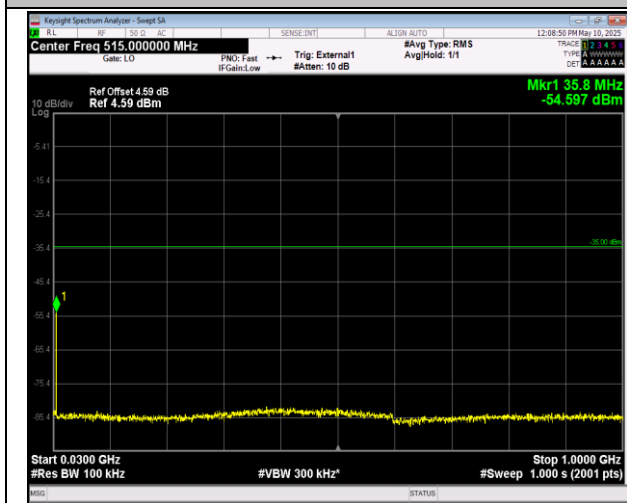
41-41-20MHz-10MHz-16QAM-16QAM-40571-40715-100 RB#0-50RB#0-30~1000MHz-PASS
