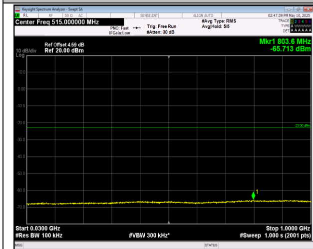
66-66-5MHz-20MHz-16QAM-16QAM-132330-132447-1RB B#0-1RB#99-30~1000MHz-PASS
