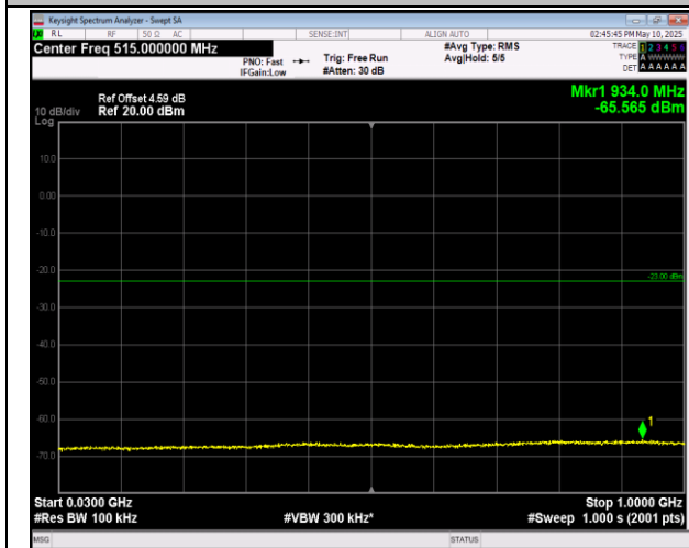
66-66-5MHz-20MHz-16QAM-16QAM-132005-132122-1R B#0-ORB#0-30~1000MHz-PASS
