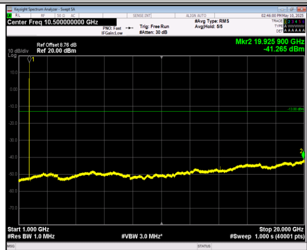
66-66-5MHz-20MHz-16QAM-16QAM-132005-132122-1RB# 0-ORB#0-1000~20000MHz-PASS
