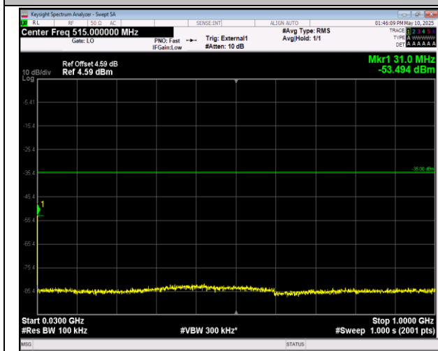
41-41-20MHz-20MHz-16QAM-16QAM-40521-40719-100 RB#0-100RB#0-30~1000MHz-PASS
