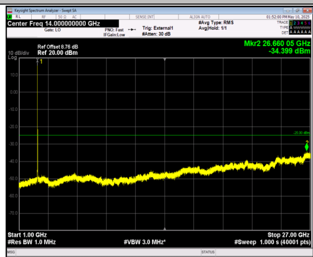
41-41-20MHz-20MHz-16QAM-16QAM-41292-41490-1RB#0 -1RB#99-1000~27000MHz-PASS
