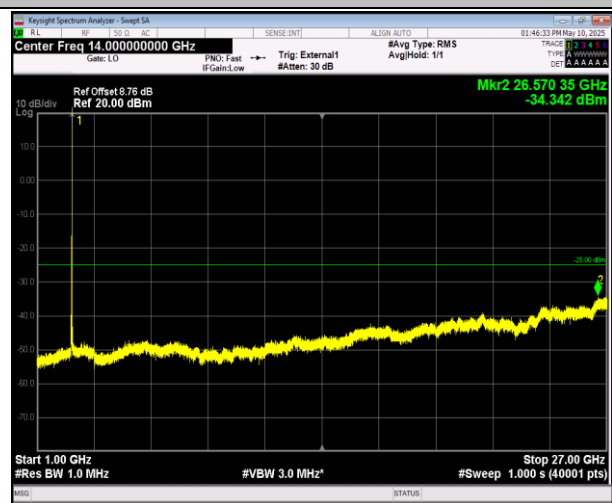
41-41-20MHz-20MHz-16QAM-16QAM-40521-40719-100RB #0-100RB#0-1000~27000MHz-PASS
