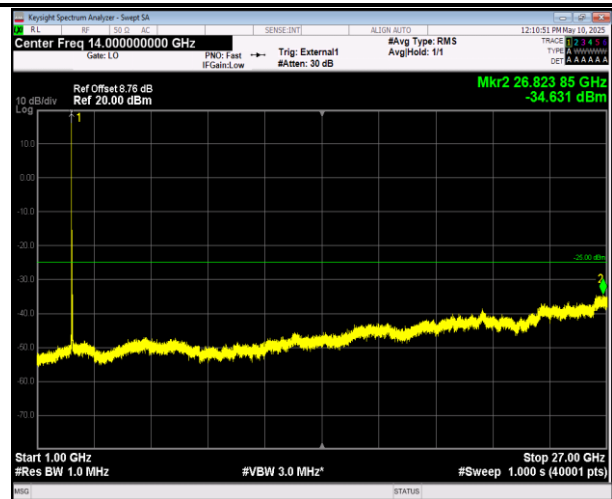
41-41-20MHz-10MHz-16QAM-16QAM-40571-40715-1RB#9 9-0RB#0-1000~27000MHz-PASS
