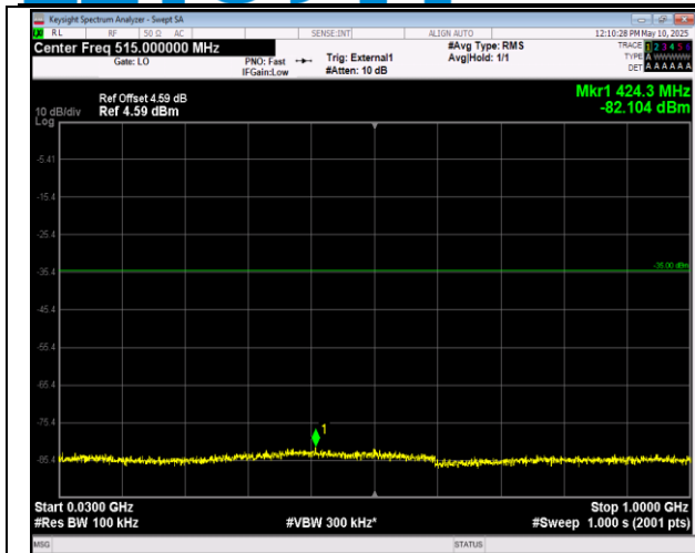
41-41-20MHz-10MHz-16QAM-16QAM-40571-40715-1RB #99-0RB#0-30~1000MHz-PASS
