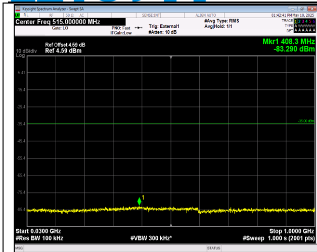
41-41-20MHz-20MHz-QPSK-QPSK-40521-40719-1RB#0 -ORB#0-30~1000MHz-PASS
