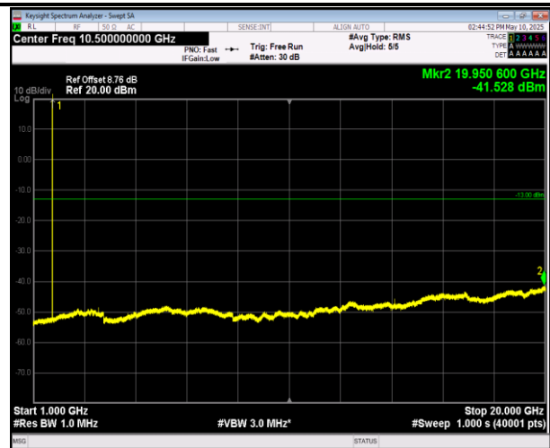
66-66-5MHz-20MHz-QPSK-QPSK-132005-132122-1RB#24 -ORB#0-1000~20000MHz-PASS
