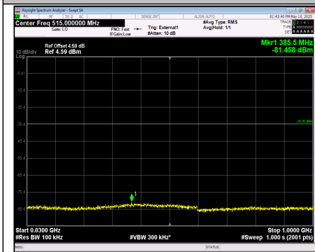
41-41-20MHz-20MHz-QPSK-QPSK-40521-40719-1RB#0 -1RB#99-30~1000MHz-PASS
