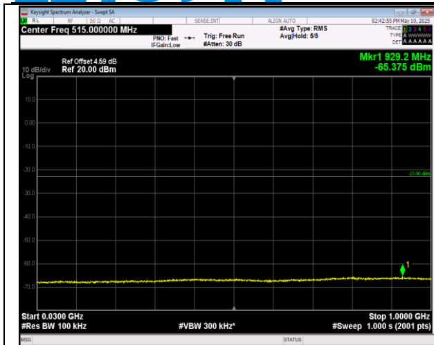
66-66-5MHz-20MHz-16QAM-16QAM-132005-132122-1R B#0-1RB#99-30~1000MHz-PASS
