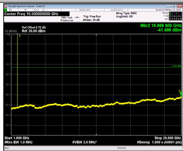
66-66-5MHz-20MHz-16QAM-16QAM-132005-132122-1RB# 24-0RB#0-1000~20000MHz-PASS
