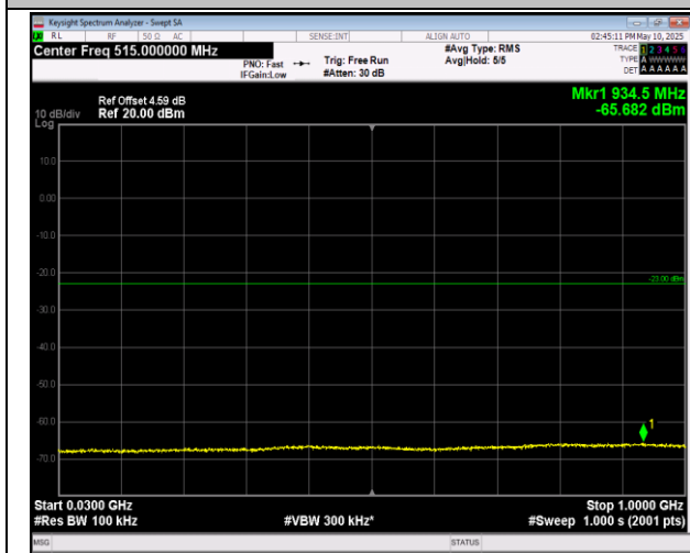
66-66-5MHz-20MHz-16QAM-16QAM-132005-132122-1R B#24-0RB#0-30~1000MHz-PASS
