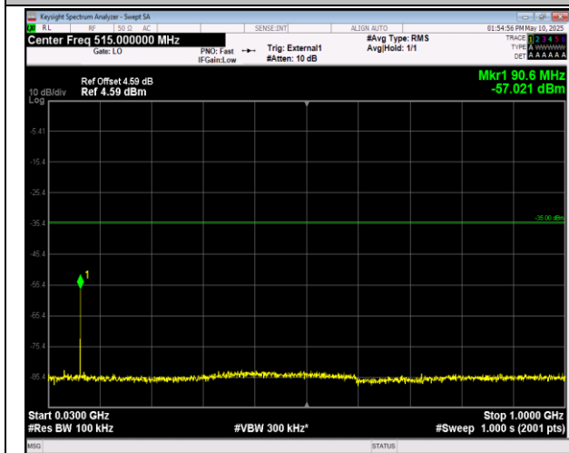
41-41-20MHz-20MHz-16QAM-16QAM-41292-41490-1RB #99-ORB#0-30~1000MHz-PASS
