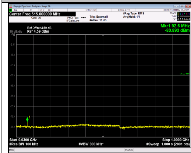
41-41-20MHz-20MHz-QPSK-QPSK-39750-39948-100RB #0-100RB#0-30~1000MHz-PASS
