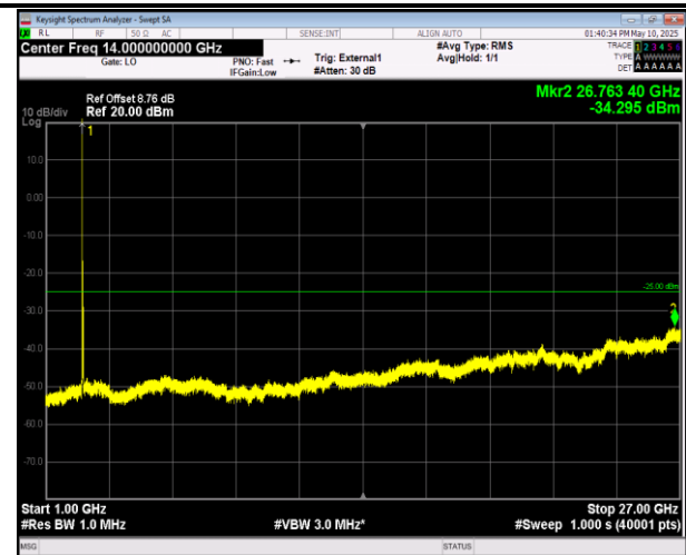
41-41-20MHz-20MHz-QPSK-QPSK-39750-39948-1RB#99- ORB#0-1000~27000MHz-PASS
