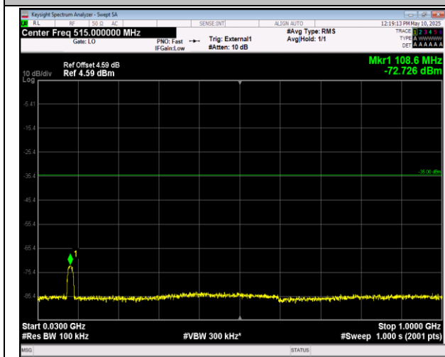
41-41-20MHz-20MHz-QPSK-QPSK-39750-39948-1RB#0 -0RB#0-30~1000MHz-PASS
