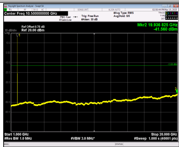
66-66-5MHz-20MHz-16QAM-16QAM-132330-132447-1RB# 0-0RB#0-1000~20000MHz-PASS
