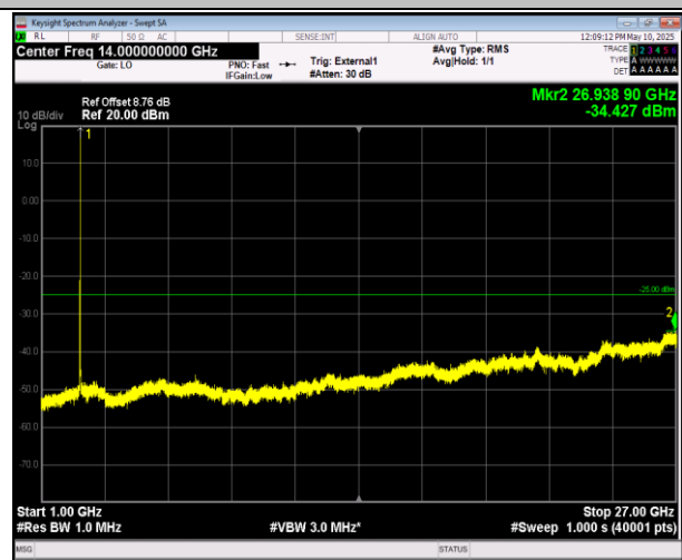
41-41-20MHz-10MHz-16QAM-16QAM-40571-40715-100RB #0-50RB#0-1000~27000MHz-PASS
