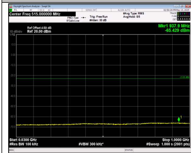
66-66-5MHz-20MHz-16QAM-16QAM-132330-132447-1RB B#0-0RB#0-30~1000MHz-PASS
