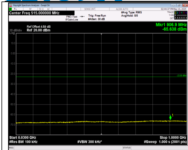
66-66-5MHz-20MHz-QPSK-QPSK-132005-132122-1RB# 24-ORB#0-30~1000MHz-PASS
