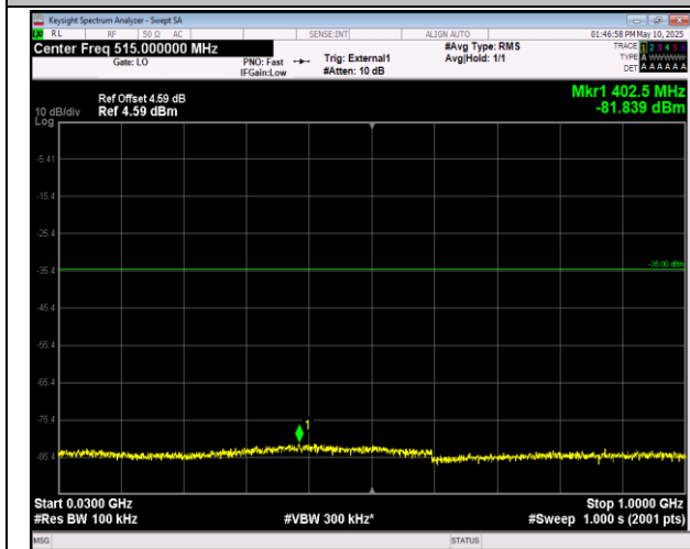
41-41-20MHz-20MHz-QPSK-QPSK-40521-40719-1RB#9 9-ORB#0-30~1000MHz-PASS
