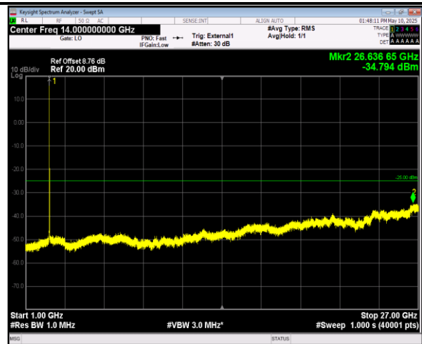
41-41-20MHz-20MHz-16QAM-16QAM-40521-40719-1RB#9 9-0RB#0-1000~27000MHz-PASS
