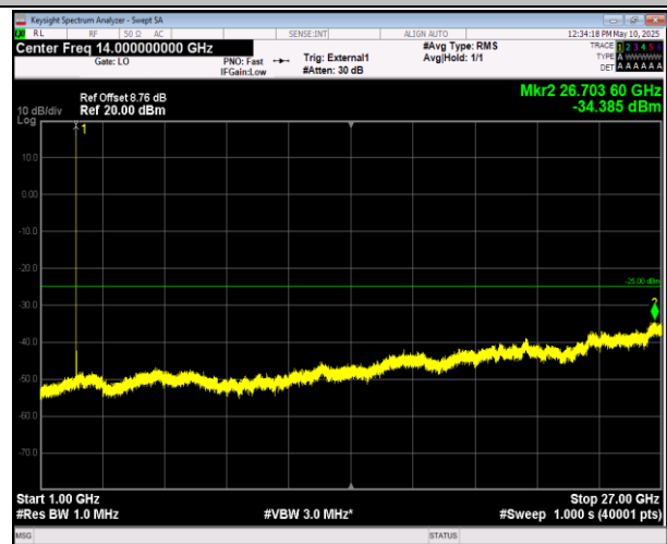
41-41-5MHz-20MHz-16QAM-16QAM-39683-39800-25RB#0 -100RB#0-1000~27000MHz-PASS
