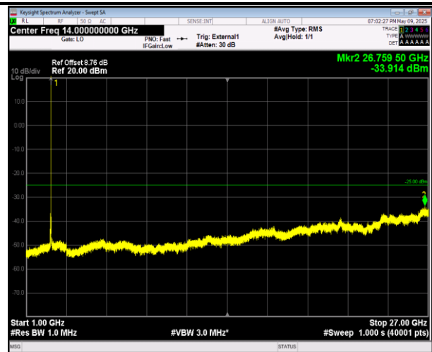
38-38-15MHz-15MHz-16QAM-16QAM-38025-38175-75RB# 0-75RB#0-1000~27000MHz-PASS
