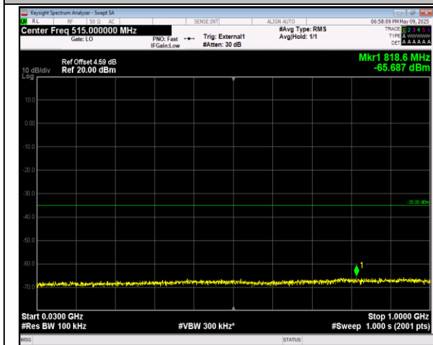
38-38-15MHz-15MHz-QPSK-QPSK-38025-38175-1RB#0 -0RB#0-30~1000MHz-PASS
