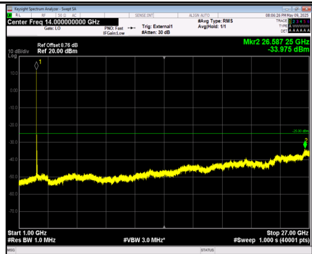
38-38-20MHz-20MHz-16QAM-16QAM-37901-38099-1RB#9 9-0RB#0-1000~27000MHz-PASS
