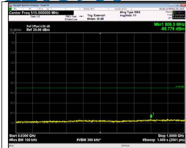
38-38-15MHz-15MHz-16QAM-16QAM-37925-38075-1RB #74-0RB#0-30~1000MHz-PASS
