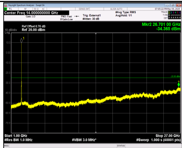
38-38-15MHz-15MHz-16QAM-16QAM-38025-38175-1RB#0 -ORB#0-1000~27000MHz-PASS
