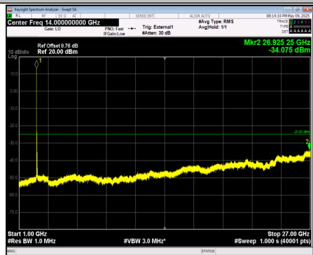
38-38-20MHz-20MHz-16QAM-16QAM-37952-38150-1RB#9 9-ORB#0-1000~27000MHz-PASS
