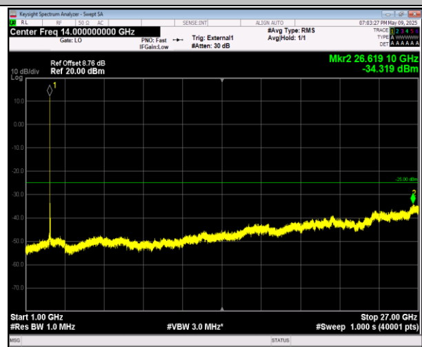
38-38-15MHz-15MHz-QPSK-QPSK-38025-38175-1RB#74- 0RB#0-1000~27000MHz-PASS
