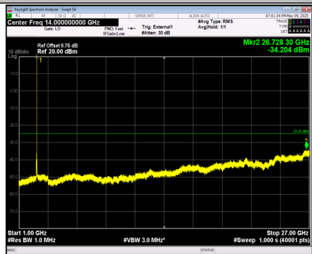
38-38-15MHz-15MHz-QPSK-QPSK-38025-38175-75RB#0- 75RB#0-1000~27000MHz-PASS
