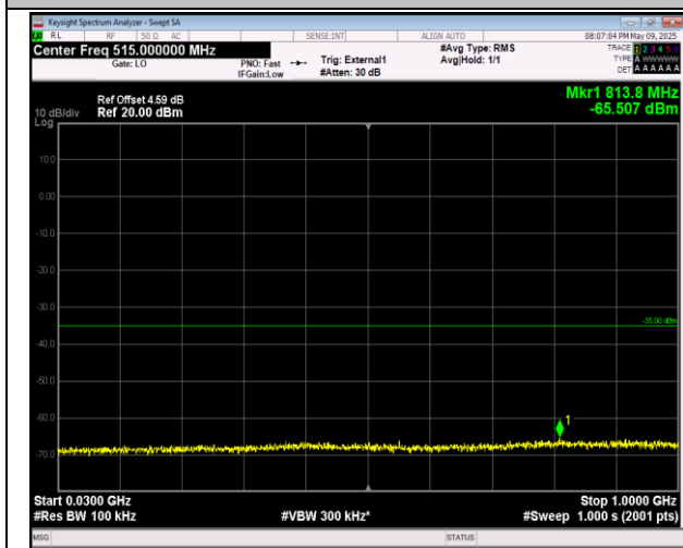
38-38-20MHz-20MHz-16QAM-16QAM-37901-38099-1RB #0-0RB#0-30~1000MHz-PASS
