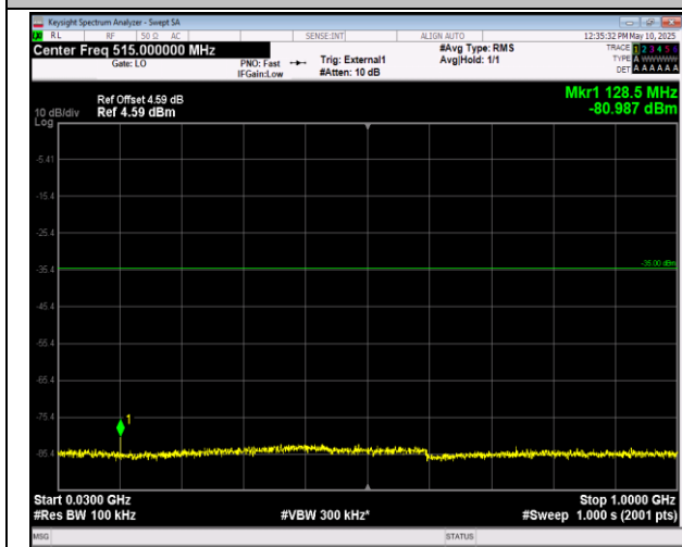
41-41-5MHz-20MHz-16QAM-16QAM-39683-39800-1RB# 24-0RB#0-30~1000MHz-PASS
