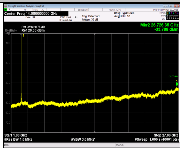
38-38-15MHz-15MHz-16QAM-16QAM-37925-38075-75RB# 0-75RB#0-1000~27000MHz-PASS
