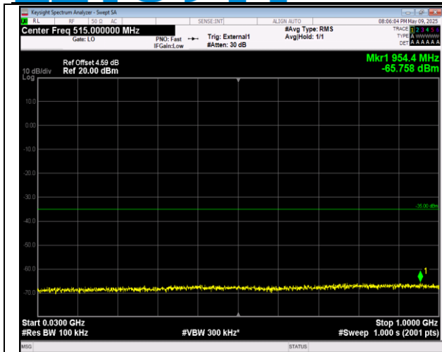
38-38-20MHz-20MHz-16QAM-16QAM-37901-38099-1RB #99-0RB#0-30~1000MHz-PASS
