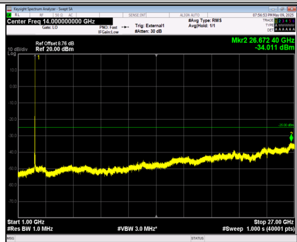
38-38-20MHz-20MHz-16QAM-16QAM-37850-38048-100RB #0-100RB#0-1000~27000MHz-PASS
