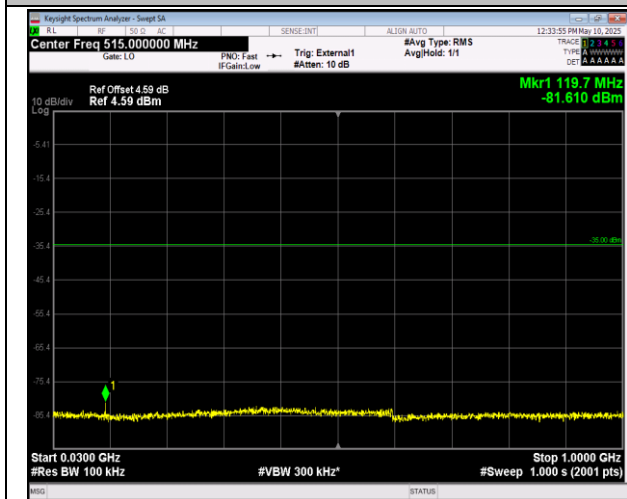
41-41-5MHz-20MHz-16QAM-16QAM-39683-39800-25RB #0-100RB#0-30~1000MHz-PASS
