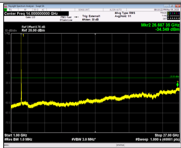
38-38-20MHz-20MHz-16QAM-16QAM-37952-38150-1RB#0 -1RB#99-1000~27000MHz-PASS
