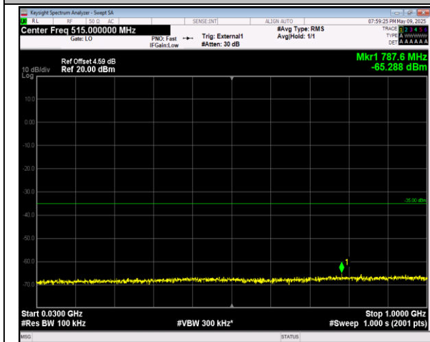
38-38-20MHz-20MHz-16QAM-16QAM-37850-38048-1RB #0-ORB#0-30~1000MHz-PASS
