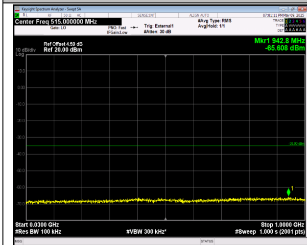
38-38-15MHz-15MHz-QPSK-QPSK-38025-38175-75RB# 0-75RB#0-30~1000MHz-PASS
