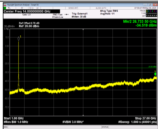
38-38-20MHz-20MHz-16QAM-16QAM-37850-38048-1RB#0 -ORB#0-1000~27000MHz-PASS
