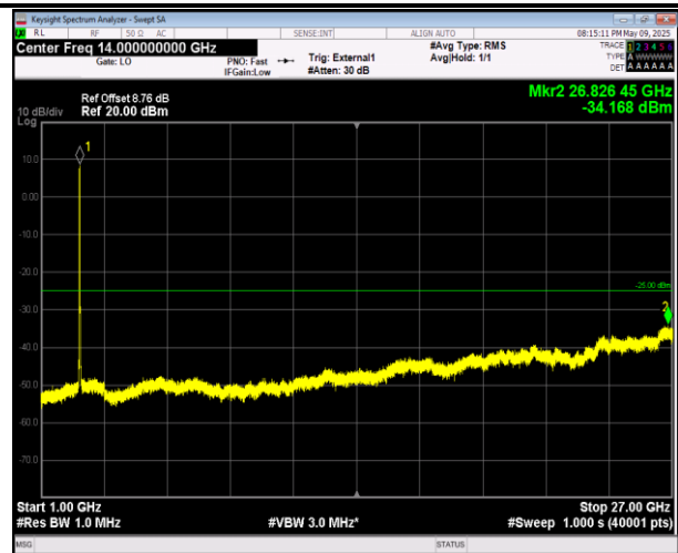
38-38-20MHz-20MHz-16QAM-16QAM-37952-38150-1RB#0 -ORB#0-1000~27000MHz-PASS
