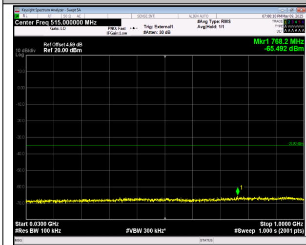
38-38-15MHz-15MHz-16QAM-16QAM-38025-38175-1RB #0-1RB#74-30~1000MHz-PASS
