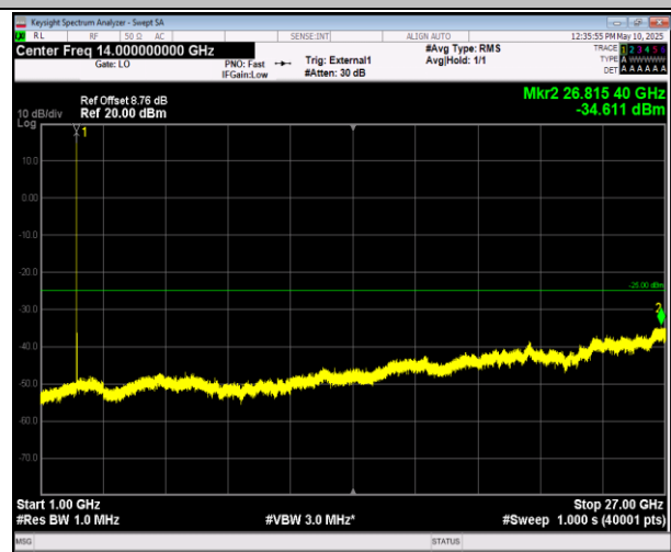
41-41-5MHz-20MHz-16QAM-16QAM-39683-39800-1RB#24 -0RB#0-1000~27000MHz-PASS
