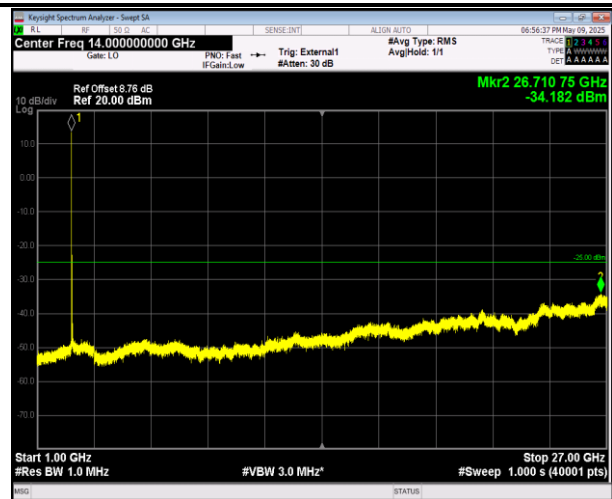
38-38-15MHz-15MHz-16QAM-16QAM-37925-38075-1RB#7 4-0RB#0-1000~27000MHz-PASS
