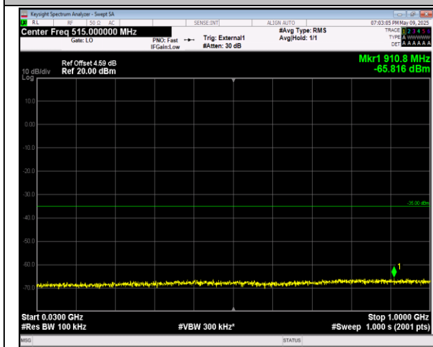
38-38-15MHz-15MHz-QPSK-QPSK-38025-38175-1RB#7 4-0RB#0-30~1000MHz-PASS
