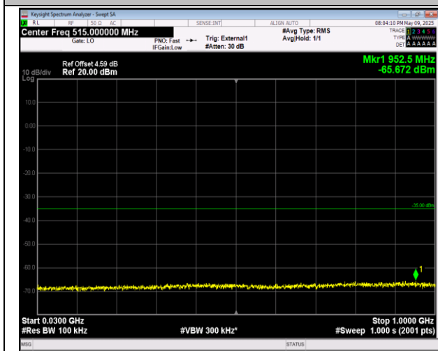
38-38-20MHz-20MHz-16QAM-16QAM-37901-38099-100RB RB#0-100RB#0-30~1000MHz-PASS
