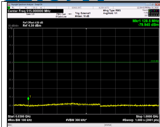
41-41-5MHz-20MHz-QPSK-QPSK-39683-39800-1RB#24 -ORB#0-30~1000MHz-PASS
