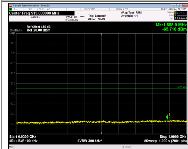
38-38-20MHz-20MHz-16QAM-16QAM-37901-38099-1RB #0-1RB#99-30~1000MHz-PASS
