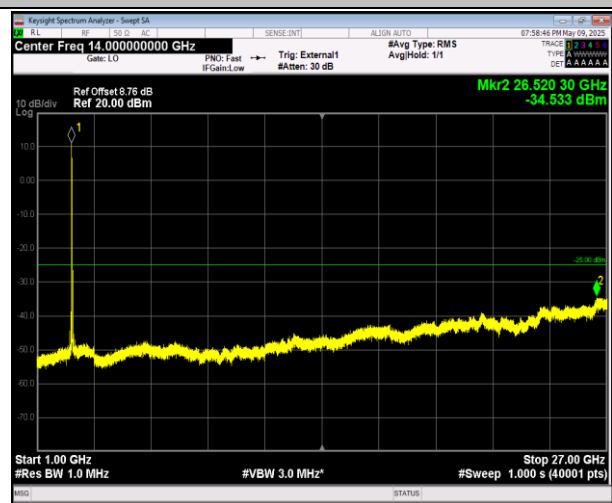
38-38-20MHz-20MHz-16QAM-16QAM-37850-38048-1RB#9 9-0RB#0-1000~27000MHz-PASS
