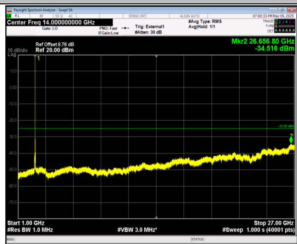
38-38-15MHz-15MHz-16QAM-16QAM-38025-38175-1RB#0 -1RB#74-1000~27000MHz-PASS
