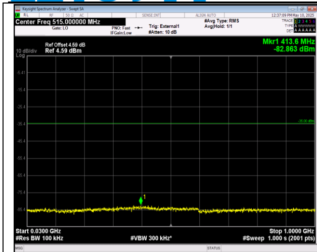
41-41-5MHz-20MHz-QPSK-QPSK-40528-40645-1RB#0-0RB#0-30~1000MHz-PASS
