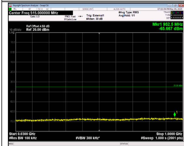
38-38-15MHz-15MHz-16QAM-16QAM-38025-38175-1RB #74-ORB#0-30~1000MHz-PASS
