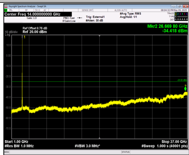
38-38-20MHz-20MHz-16QAM-16QAM-37901-38099-100RB #0-100RB#0-1000~27000MHz-PASS
