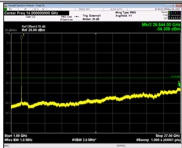
38-38-15MHz-15MHz-16QAM-16QAM-38025-38175-1RB#7 4-ORB#0-1000~27000MHz-PASS
