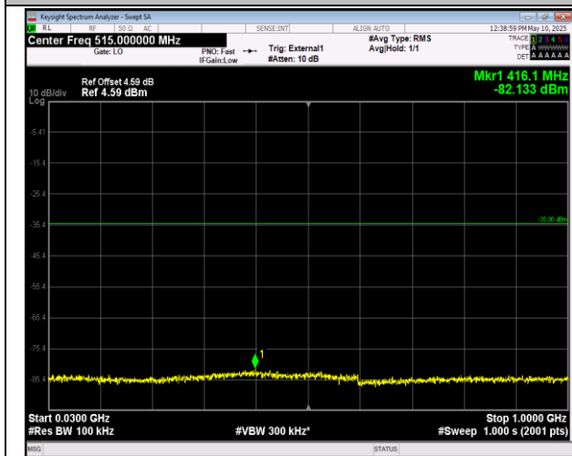
41-41-5MHz-20MHz-16QAM-16QAM-40528-40645-1RB# 0-1RB#99-30~1000MHz-PASS
