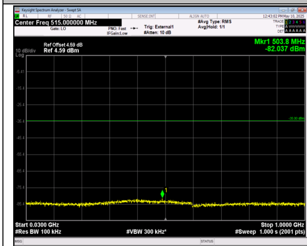
41-41-5MHz-20MHz-16QAM-16QAM-40528-40645-1RB# 0-0RB#0-30~1000MHz-PASS
