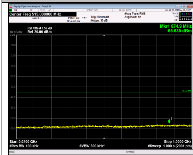
38-38-15MHz-15MHz-16QAM-16QAM-37925-38075-75R B#0-75RB#0-30~1000MHz-PASS
