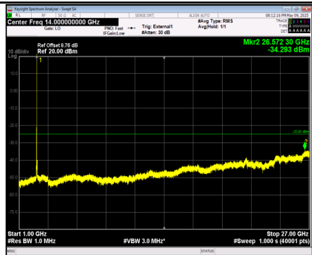
38-38-20MHz-20MHz-16QAM-16QAM-37952-38150-100RB #0-100RB#0-1000~27000MHz-PASS
