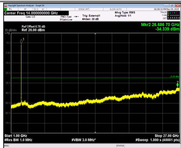
38-38-15MHz-15MHz-QPSK-QPSK-38025-38175-1RB#0-0 RB#0-1000~27000MHz-PASS
