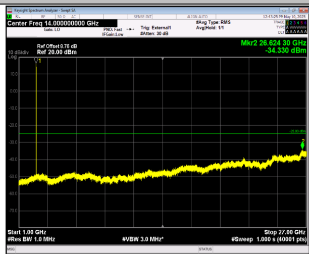
41-41-5MHz-20MHz-16QAM-16QAM-40528-40645-1RB#0- 0RB#0-1000~27000MHz-PASS
