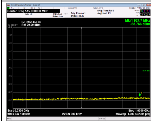
38-38-20MHz-20MHz-16QAM-16QAM-37850-38048-1RB #99-0RB#0-30~1000MHz-PASS
