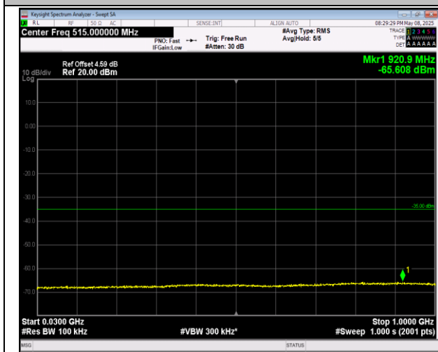
7-7-20MHz-10MHz-QPSK-QPSK-21251-21395-1RB#99-0 ORB#0-30~1000MHz-PASS
