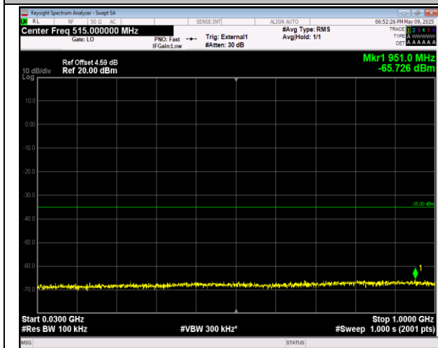
38-38-15MHz-15MHz-16QAM-16QAM-37925-38075-1RB #0-1RB#74-30~1000MHz-PASS
