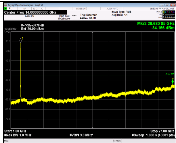
38-38-15MHz-15MHz-QPSK-QPSK-37925-38075-1RB#0-0 RB#0-1000~27000MHz-PASS
