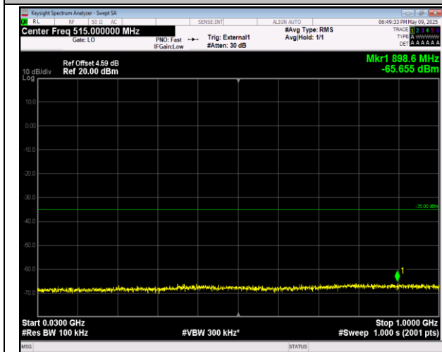
38-38-15MHz-15MHz-16QAM-16QAM-37825-37975-1RB #0-ORB#0-30~1000MHz-PASS
