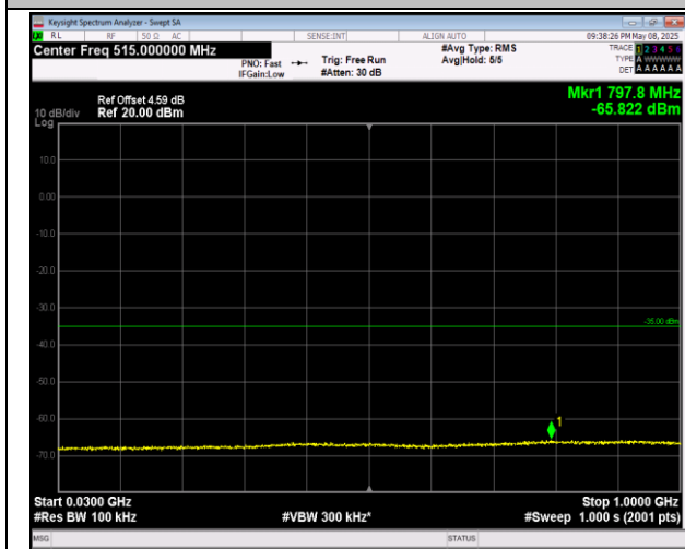
7-7-20MHz-20MHz-16QAM-16QAM-20850-21048-1RB#9 9-0RB#0-30~1000MHz-PASS
