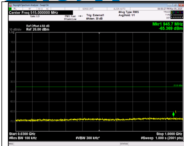
38-38-15MHz-15MHz-QPSK-QPSK-37925-38075-1RB#0 -ORB#0-30~1000MHz-PASS
