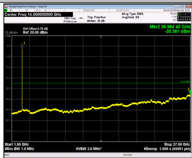
7-7-20MHz-20MHz-16QAM-16QAM-21001-21199-1RB#0-0RB#0-1000~27000MHz-PASS
