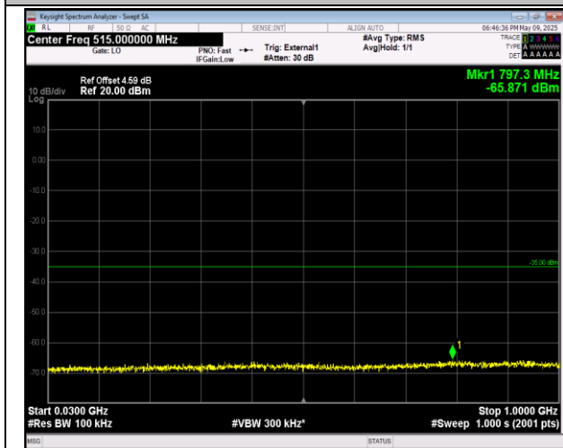
38-38-15MHz-15MHz-16QAM-16QAM-37825-37975-75R B#0-75RB#0-30~1000MHz-PASS
