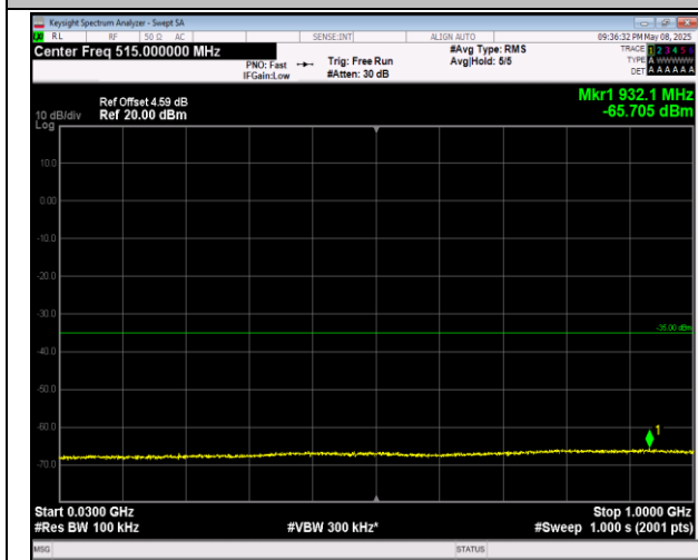
7-7-20MHz-20MHz-QPSK-QPSK-20850-21048-100RB#0-100RB#0-30~1000MHz-PASS
