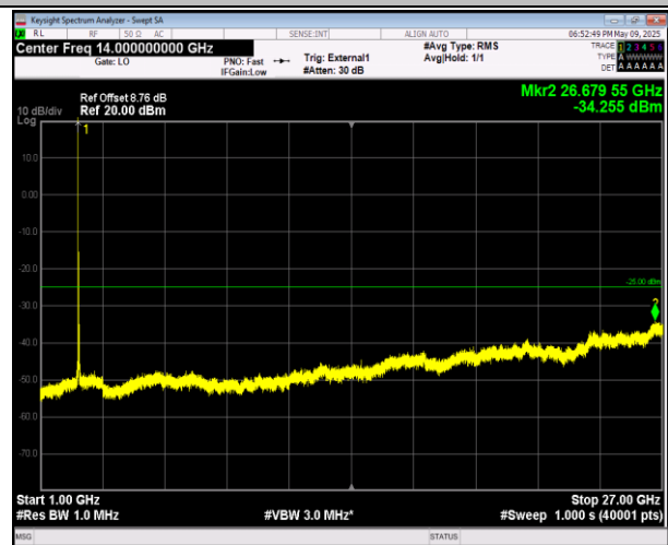
38-38-15MHz-15MHz-16QAM-16QAM-37925-38075-1RB#0 -1RB#74-1000~27000MHz-PASS
