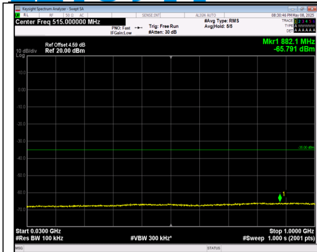
7-7-20MHz-10MHz-16QAM-16QAM-21251-21395-1RB#0 -ORB#0-30~1000MHz-PASS
