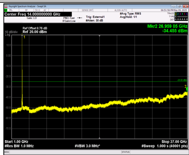
38-38-15MHz-15MHz-QPSK-QPSK-37925-38075-1RB#0-1 RB#74-1000~27000MHz-PASS
