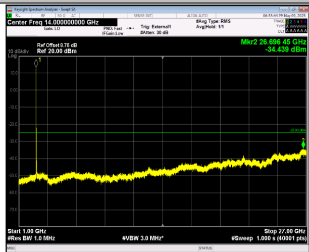
38-38-15MHz-15MHz-QPSK-QPSK-37925-38075-1RB#74- ORB#0-1000~27000MHz-PASS
