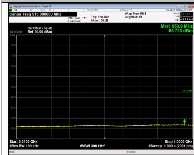
7-7-20MHz-20MHz-16QAM-16QAM-21001-21199-1RB#0-0RB#0-30~1000MHz-PASS
