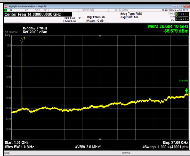
7-7-20MHz-20MHz-QPSK-QPSK-21152-21350-1RB#99-0R B#0-1000~27000MHz-PASS
