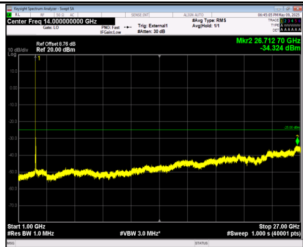
38-38-15MHz-15MHz-16QAM-16QAM-37825-37975-1RB#0 -1RB#74-1000~27000MHz-PASS
