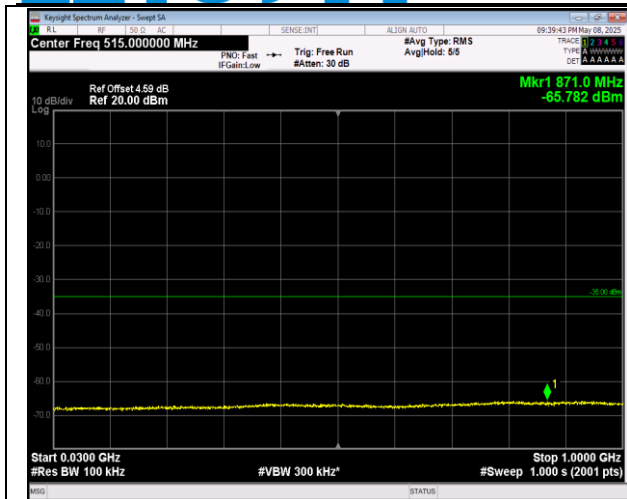
7-7-20MHz-20MHz-QPSK-QPSK-21001-21199-1RB#0-0 RB#0-30~1000MHz-PASS
