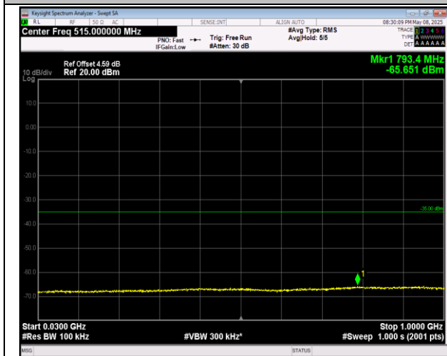
7-7-20MHz-10MHz-16QAM-16QAM-21251-21395-1RB#9 9-ORB#0-30~1000MHz-PASS
