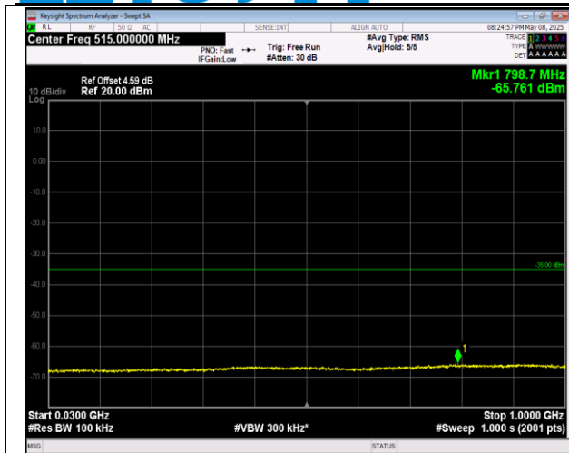
7-7-20MHz-10MHz-16QAM-16QAM-21051-21195-1RB#9 9-0RB#0-30~1000MHz-PASS
