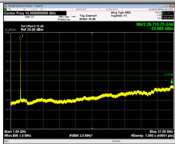
38-38-15MHz-15MHz-16QAM-16QAM-37825-37975-1RB#7 4-0RB#0-1000~27000MHz-PASS
