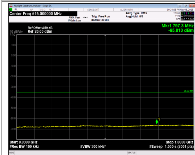
7-7-20MHz-20MHz-16QAM-16QAM-20850-21048-1RB#0-0RB#0-30~1000MHz-PASS
