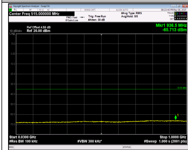
7-7-20MHz-10MHz-16QAM-16QAM-21051-21195-100RB #0-50RB#0-30~1000MHz-PASS
