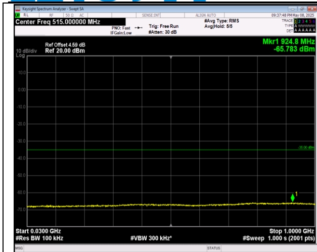
7-7-20MHz-20MHz-QPSK-QPSK-20850-21048-1RB#99-0RB#0-30~1000MHz-PASS
