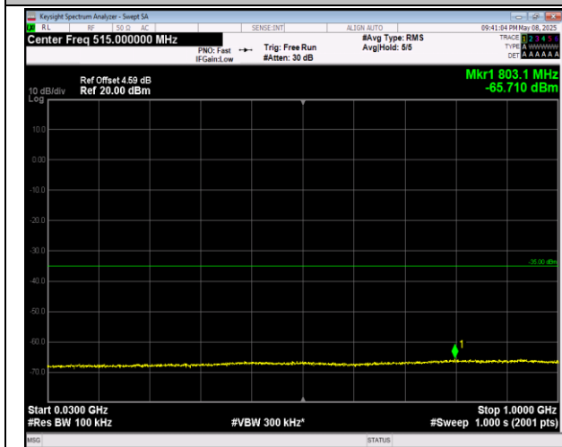
7-7-20MHz-20MHz-16QAM-16QAM-21001-21199-1RB#0-1RB#99-30~1000MHz-PASS
