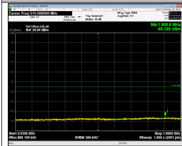
38-38-15MHz-15MHz-16QAM-16QAM-37925-38075-1RB #0-0RB#0-30~1000MHz-PASS
