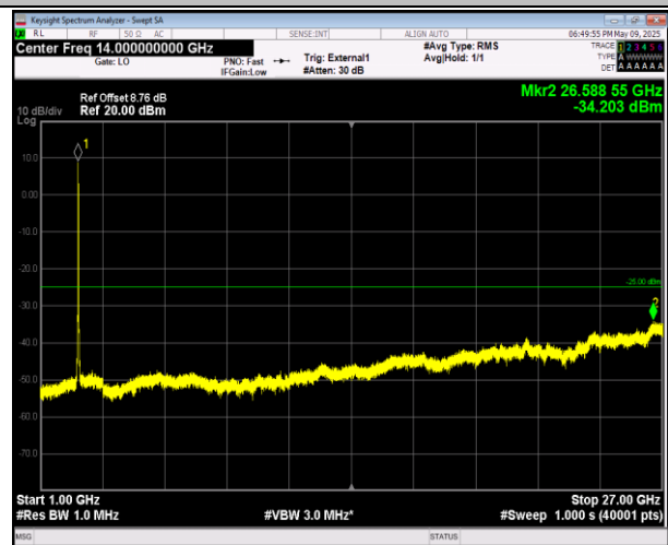
38-38-15MHz-15MHz-16QAM-16QAM-37825-37975-1RB#0 -ORB#0-1000~27000MHz-PASS
