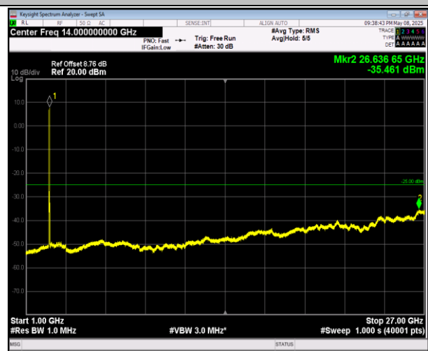
7-7-20MHz-20MHz-16QAM-16QAM-20850-21048-1RB#99- 0RB#0-1000~27000MHz-PASS
