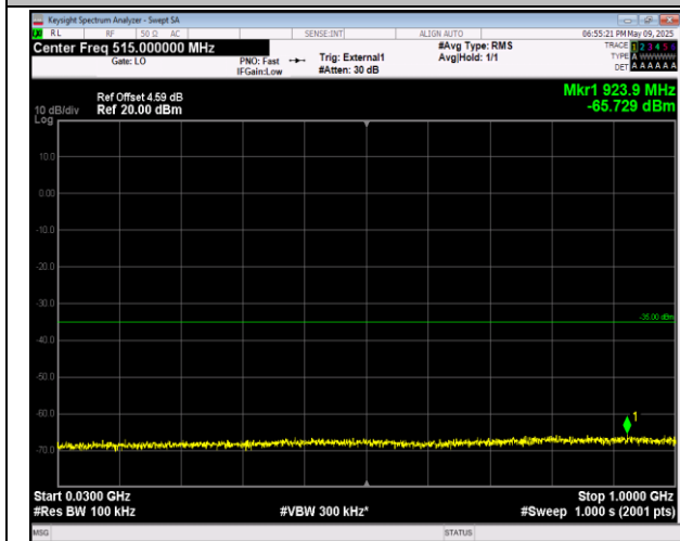
38-38-15MHz-15MHz-QPSK-QPSK-37925-38075-1RB#7 4-ORB#0-30~1000MHz-PASS
