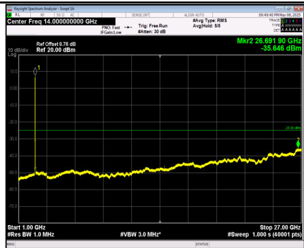
7-7-20MHz-20MHz-16QAM-16QAM-21152-21350-1RB#0-0 RB#0-1000~27000MHz-PASS
