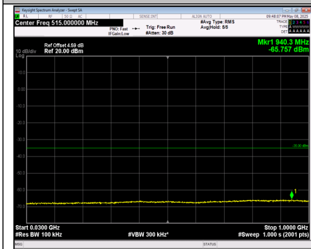
7-7-20MHz-20MHz-QPSK-QPSK-21152-21350-1RB#99-0 RB#0-30~1000MHz-PASS
