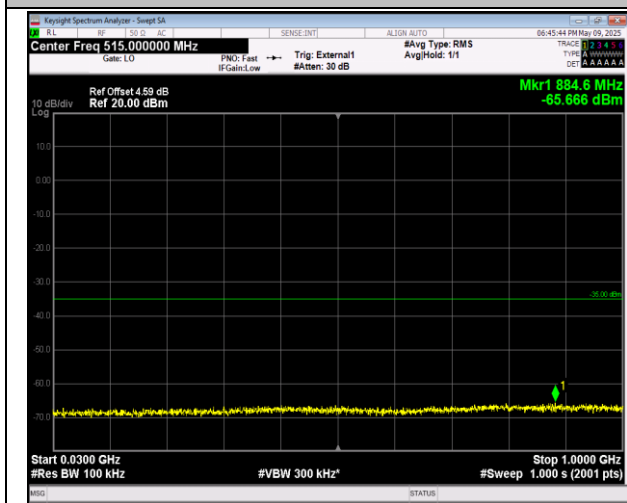
38-38-15MHz-15MHz-QPSK-QPSK-37825-37975-75RB# 0-75RB#0-30~1000MHz-PASS
