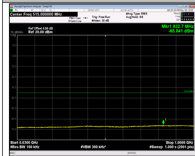
7-7-20MHz-10MHz-16QAM-16QAM-21051-21195-1RB#0-0-ORB#0-30~1000MHz-PASS
