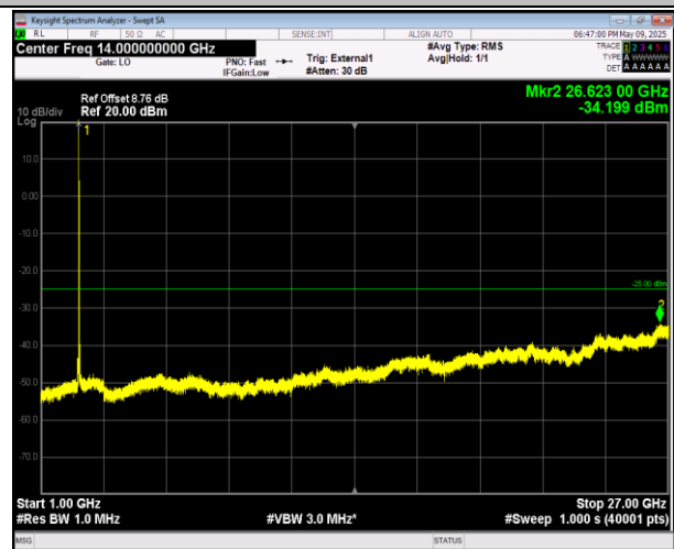
38-38-15MHz-15MHz-16QAM-16QAM-37825-37975-75RB# 0-75RB#0-1000~27000MHz-PASS
