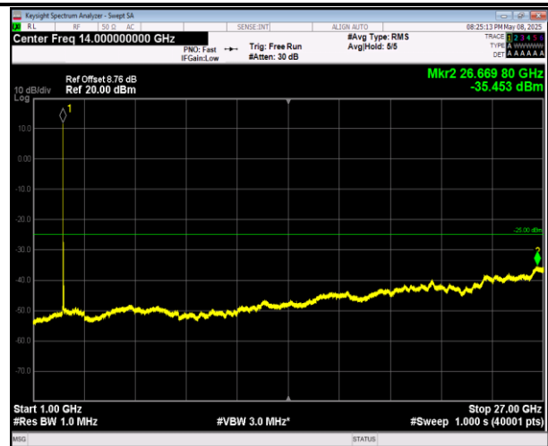
7-7-20MHz-10MHz-16QAM-16QAM-21051-21195-1RB#99- 0RB#0-1000~27000MHz-PASS
