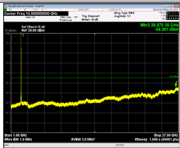
38-38-15MHz-15MHz-QPSK-QPSK-37825-37975-75RB#0- 75RB#0-1000~27000MHz-PASS
