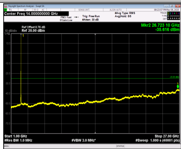
7-7-20MHz-10MHz-16QAM-16QAM-21051-21195-100RB#0 -50RB#0-1000~27000MHz-PASS
