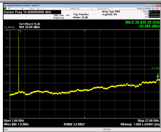
7-7-20MHz-20MHz-16QAM-16QAM-21152-21350-1RB#0-1 RB#99-1000~27000MHz-PASS
