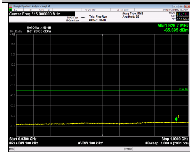
7-7-20MHz-20MHz-16QAM-16QAM-21152-21350-1RB#0 -1RB#99-30~1000MHz-PASS
