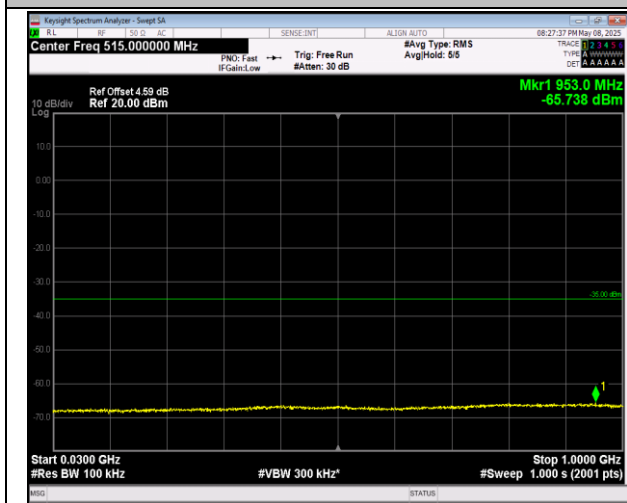
7-7-20MHz-10MHz-16QAM-16QAM-21251-21395-1RB#0 -1RB#49-30~1000MHz-PASS
