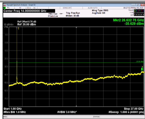
7-7-20MHz-10MHz-16QAM-16QAM-21251-21395-1RB#0-1 RB#49-1000~27000MHz-PASS
