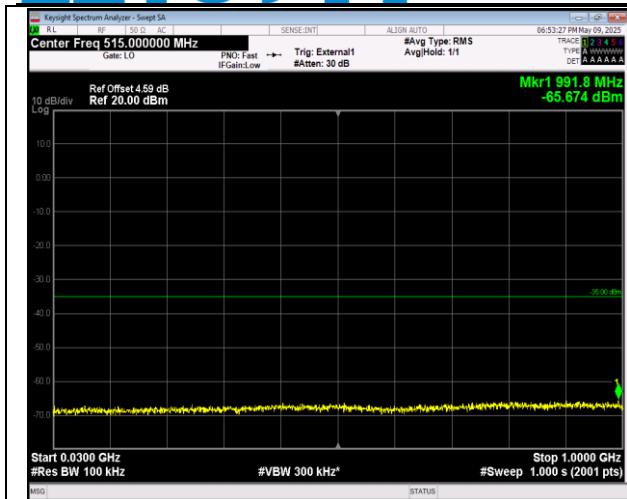
38-38-15MHz-15MHz-QPSK-QPSK-37925-38075-75RB# 0-75RB#0-30~1000MHz-PASS
