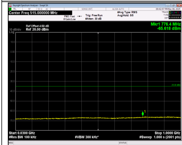
7-7-20MHz-20MHz-QPSK-QPSK-21001-21199-1RB#99-0 RB#0-30~1000MHz-PASS
