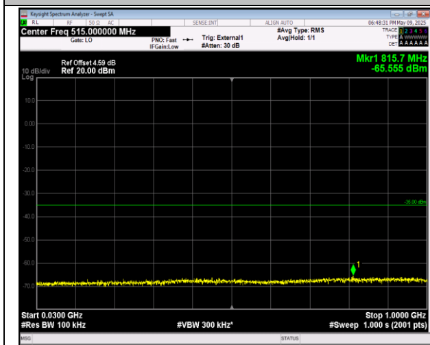
38-38-15MHz-15MHz-16QAM-16QAM-37825-37975-1RB #74-0RB#0-30~1000MHz-PASS
