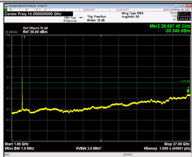
7-7-20MHz-20MHz-16QAM-16QAM-21001-21199-1RB#0-1RB#99-1000~27000MHz-PASS
