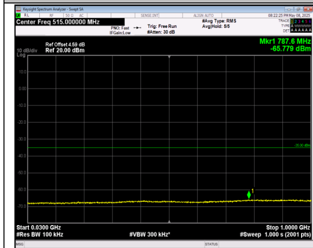
7-7-20MHz-10MHz-16QAM-16QAM-21051-21195-1RB#0-0-ORB#0-30~1000MHz-PASS
