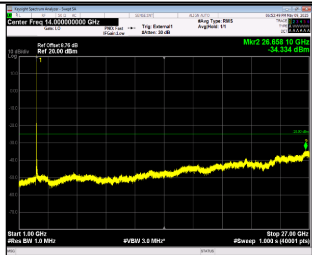
38-38-15MHz-15MHz-QPSK-QPSK-37925-38075-75RB#0- 75RB#0-1000~27000MHz-PASS
