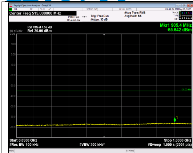
7-7-20MHz-20MHz-16QAM-16QAM-21152-21350-1RB#0 -ORB#0-30~1000MHz-PASS
