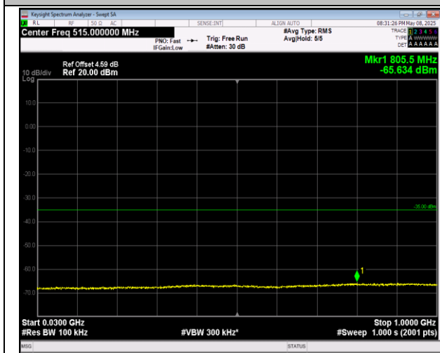
7-7-20MHz-20MHz-QPSK-QPSK-20850-21048-1RB#0-0 RB#0-30~1000MHz-PASS
