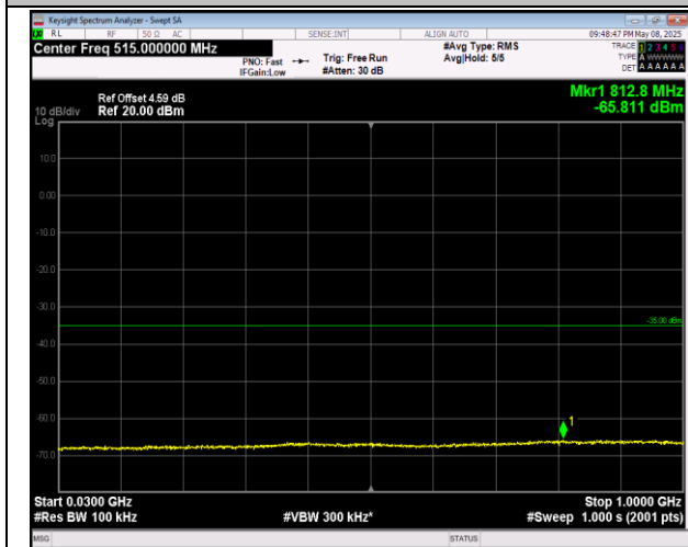
7-7-20MHz-20MHz-16QAM-16QAM-21152-21350-1RB#9 9-ORB#0-30~1000MHz-PASS
