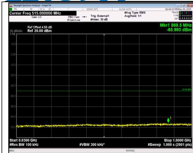
38-38-15MHz-15MHz-16QAM-16QAM-37825-37975-1RB #0-1RB#74-30~1000MHz-PASS
