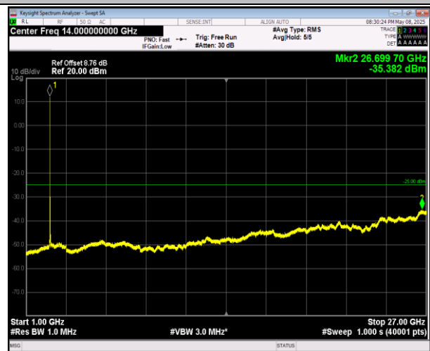
7-7-20MHz-10MHz-16QAM-16QAM-21251-21395-1RB#99- ORB#0-1000~27000MHz-PASS
