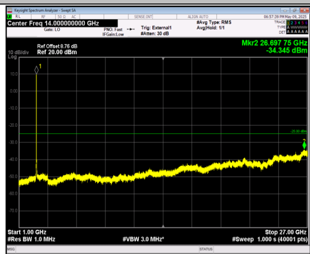
38-38-15MHz-15MHz-16QAM-16QAM-37925-38075-1RB#0 -0RB#0-1000~27000MHz-PASS
