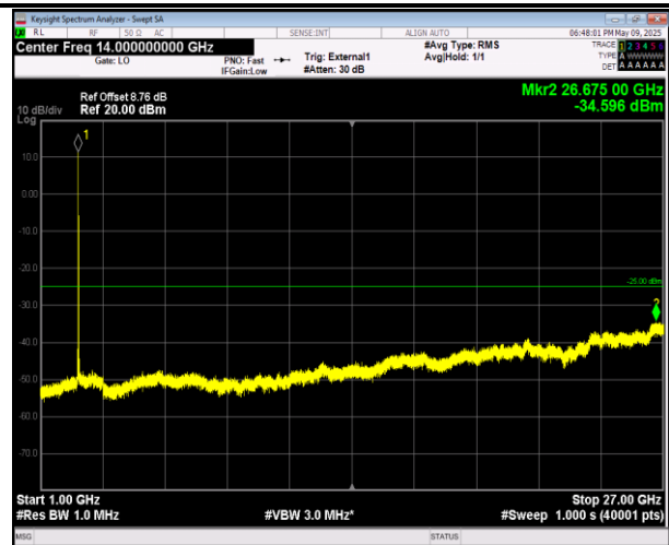
38-38-15MHz-15MHz-QPSK-QPSK-37825-37975-1RB#74- ORB#0-1000~27000MHz-PASS
