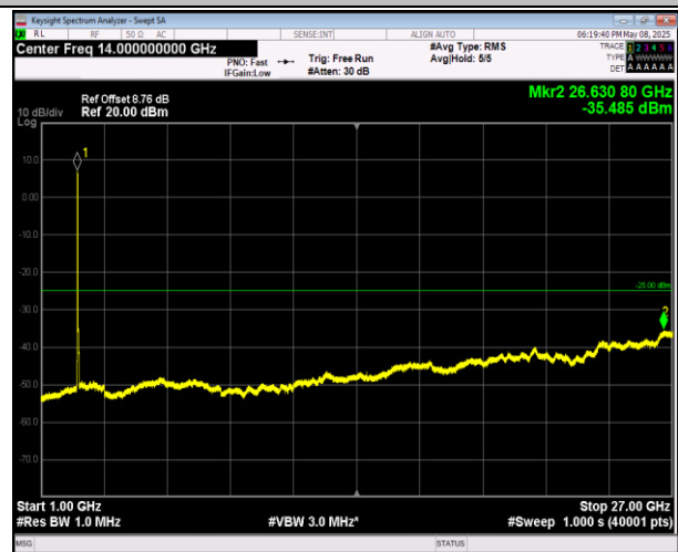
7-7-10MHz-20MHz-16QAM-16QAM-20805-20949-1RB#0-0RB#0-1000~27000MHz-PASS
