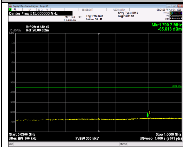
7-7-10MHz-20MHz-16QAM-16QAM-21006-21150-1RB#0 -ORB#0-30~1000MHz-PASS
