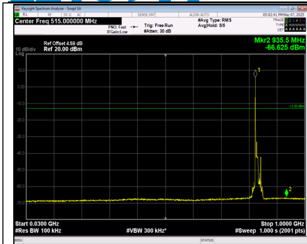
5-5-10MHz-10MHz-16QAM-16QAM-20476-20575-1RB#4 9-0RB#0-30~1000MHz-PASS
