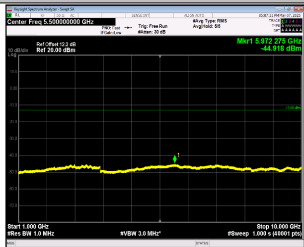
5-5-10MHz-10MHz-16QAM-16QAM-20501-20600-1RB#49- ORB#0-1000~10000MHz-PASS
