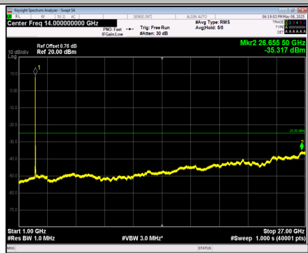
7-7-10MHz-20MHz-16QAM-16QAM-20805-20949-1RB#49- 0RB#0-1000~27000MHz-PASS
