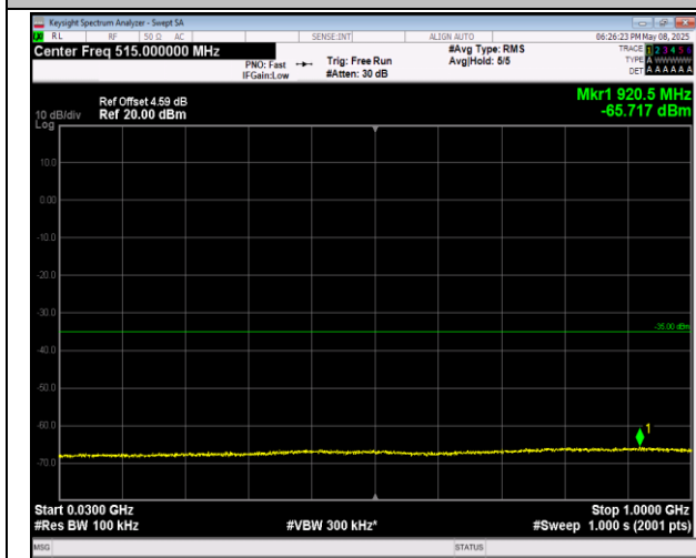
7-7-10MHz-20MHz-16QAM-16QAM-21206-21350-1RB#0 -1RB#99-30~1000MHz-PASS
