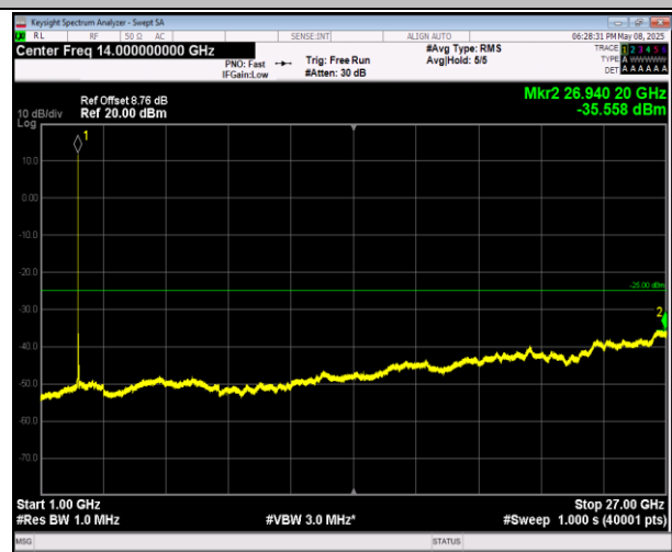
7-7-10MHz-20MHz-QPSK-QPSK-21206-21350-1RB#49-0R B#0-1000~27000MHz-PASS
