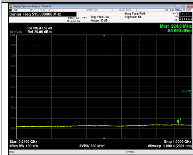
7-7-20MHz-10MHz-16QAM-16QAM-20850-20994-1RB#9 9-0RB#0-30~1000MHz-PASS
