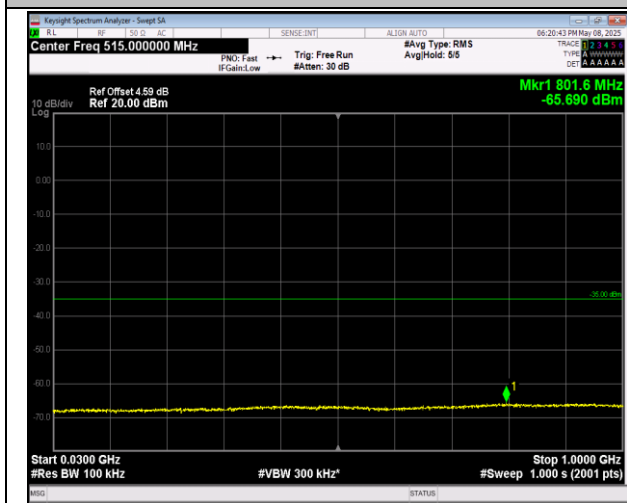
7-7-10MHz-20MHz-QPSK-QPSK-21006-21150-1RB#0-1 RB#99-30~1000MHz-PASS
