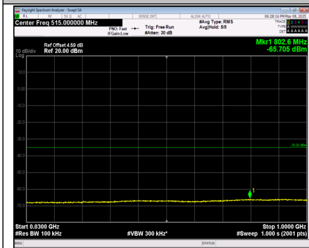
7-7-10MHz-20MHz-QPSK-QPSK-21206-21350-1RB#49- 0RB#0-30~1000MHz-PASS
