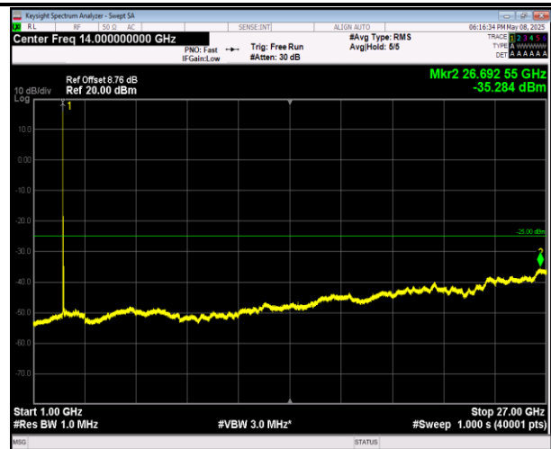
7-7-10MHz-20MHz-16QAM-16QAM-20805-20949-1RB#0-1 RB#99-1000~27000MHz-PASS
