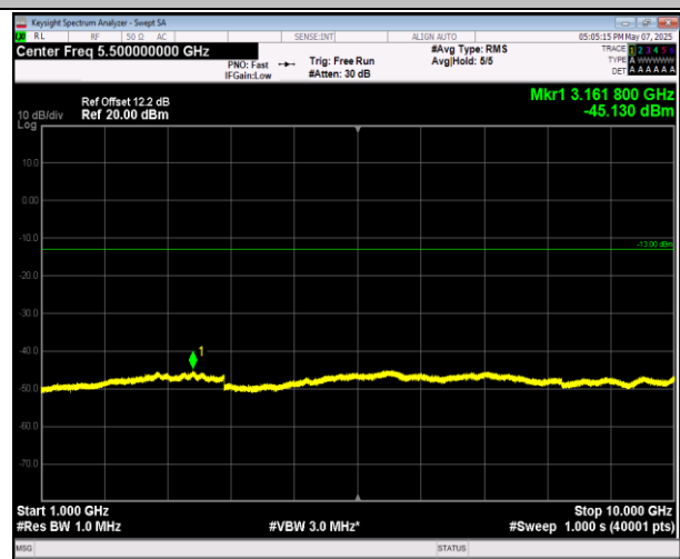
5-5-10MHz-10MHz-16QAM-16QAM-20501-20600-1RB#0-1 RB#49-1000~10000MHz-PASS
