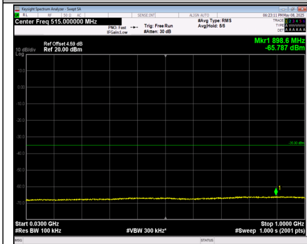
7-7-10MHz-20MHz-QPSK-QPSK-21006-21150-1RB#49-0 RB#0-30~1000MHz-PASS
