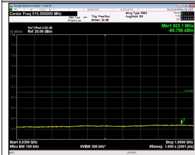
7-7-10MHz-20MHz-16QAM-16QAM-20805-20949-1RB#0-0RB#0-30~1000MHz-PASS
