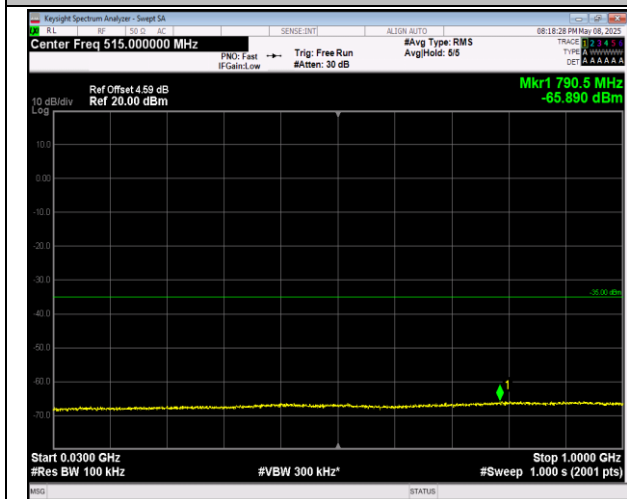
7-7-20MHz-10MHz-16QAM-16QAM-20850-20994-100RB #0-50RB#0-30~1000MHz-PASS
