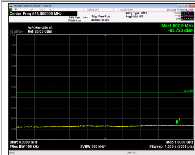
7-7-20MHz-10MHz-16QAM-16QAM-20850-20994-1RB#0-0RB#0-30~1000MHz-PASS
