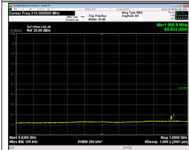
7-7-10MHz-20MHz-16QAM-16QAM-21006-21150-1RB#0 -1RB#99-30~1000MHz-PASS
