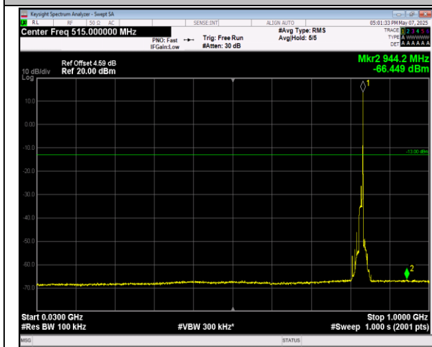
5-5-10MHz-10MHz-16QAM-16QAM-20476-20575-50RB#- 0-50RB#0-30~1000MHz-PASS
