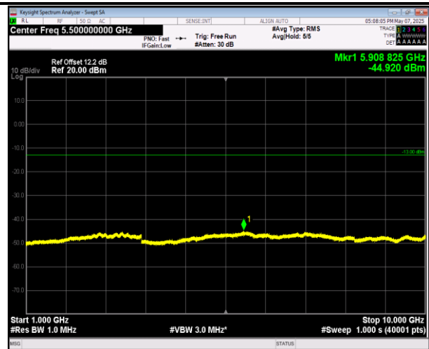
5-5-10MHz-10MHz-16QAM-16QAM-20501-20600-1RB#0-0 RB#0-1000~10000MHz-PASS
