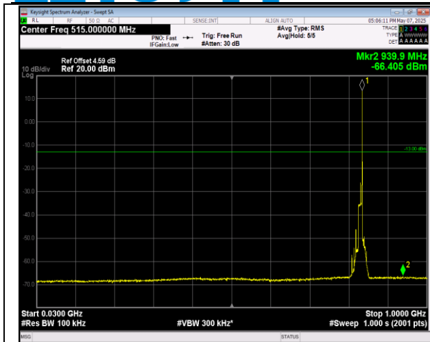
5-5-10MHz-10MHz-16QAM-16QAM-20501-20600-50RB# 0-50RB#0-30~1000MHz-PASS
