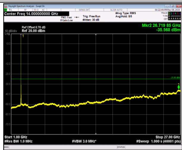
7-7-10MHz-20MHz-16QAM-16QAM-21006-21150-50RB#0- 100RB#0-1000~27000MHz-PASS
