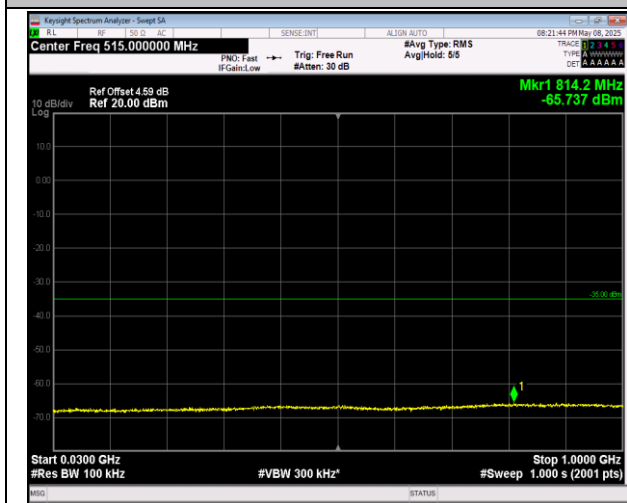
7-7-20MHz-10MHz-QPSK-QPSK-21051-21195-1RB#0-1 RB#49-30~1000MHz-PASS
