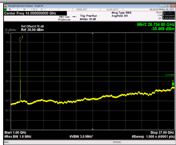
7-7-10MHz-20MHz-16QAM-16QAM-21006-21150-1RB#0-0 RB#0-1000~27000MHz-PASS
