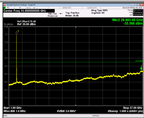
7-7-20MHz-10MHz-16QAM-16QAM-20850-20994-1RB#99- 0RB#0-1000~27000MHz-PASS
