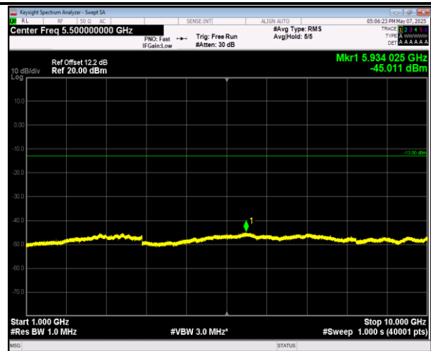
5-5-10MHz-10MHz-16QAM-16QAM-20501-20600-50RB#0- 50RB#0-1000~10000MHz-PASS
