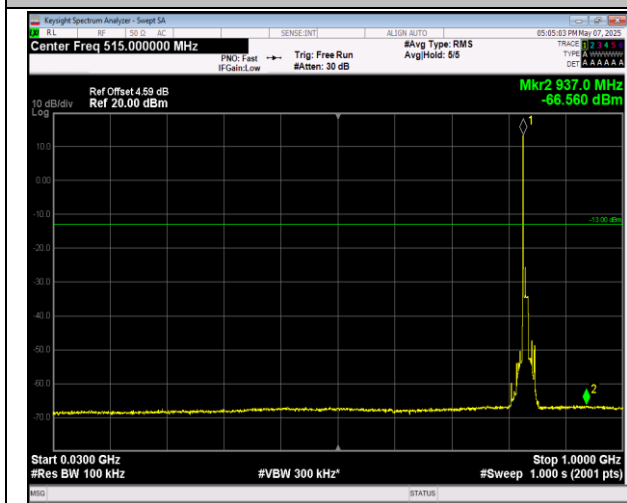
5-5-10MHz-10MHz-16QAM-16QAM-20501-20600-1RB#0 -1RB#49-30~1000MHz-PASS
