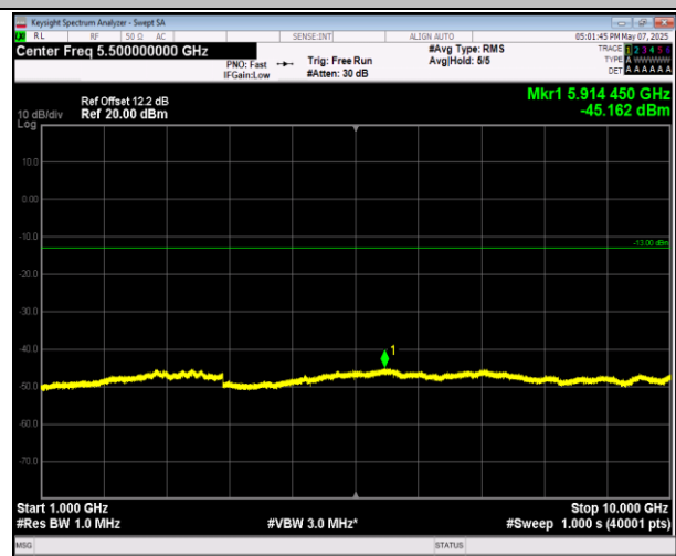
5-5-10MHz-10MHz-16QAM-16QAM-20476-20575-50RB#0- 50RB#0-1000~10000MHz-PASS
