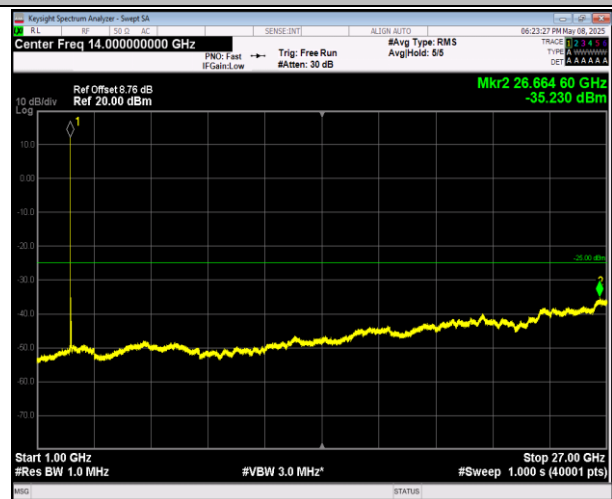
7-7-10MHz-20MHz-QPSK-QPSK-21006-21150-1RB#49-0R B#0-1000~27000MHz-PASS
