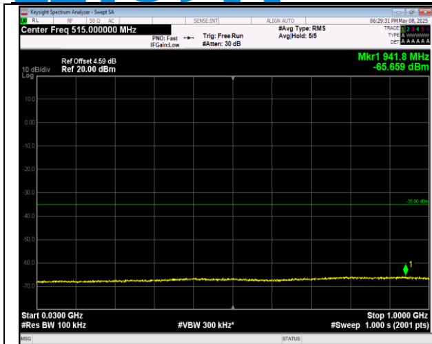
7-7-10MHz-20MHz-16QAM-16QAM-21206-21350-1RB#0 -ORB#0-30~1000MHz-PASS
