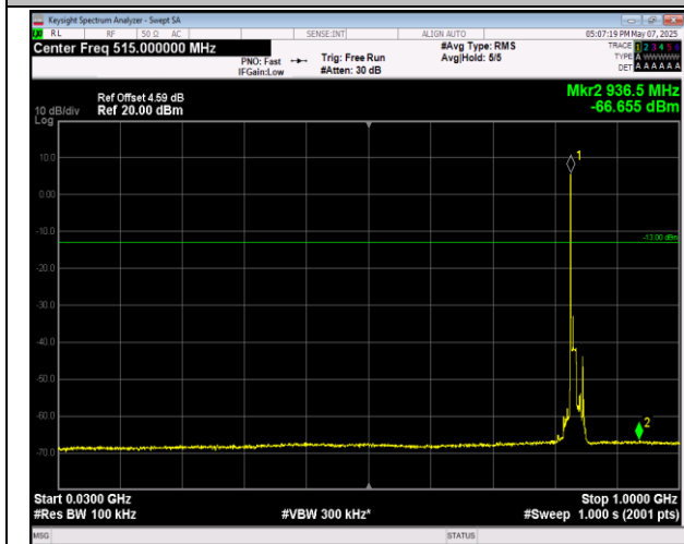
5-5-10MHz-10MHz-16QAM-16QAM-20501-20600-1RB#4 9-ORB#0-30~1000MHz-PASS
