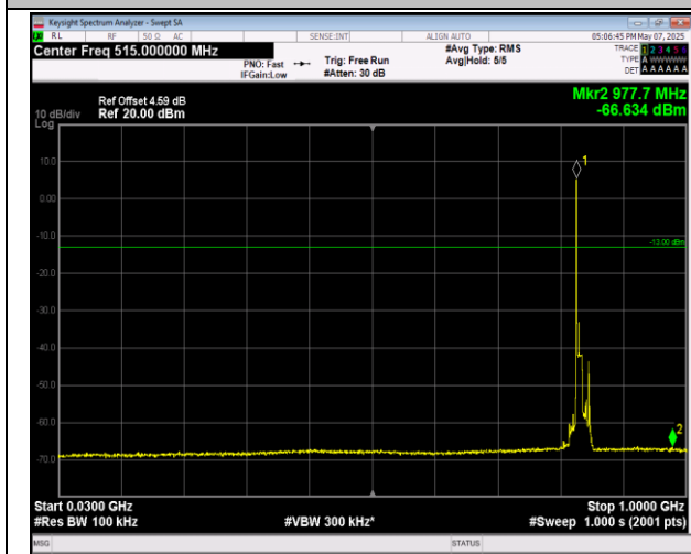
5-5-10MHz-10MHz-QPSK-QPSK-20501-20600-1RB#49-0RB#0-30~1000MHz-PASS
