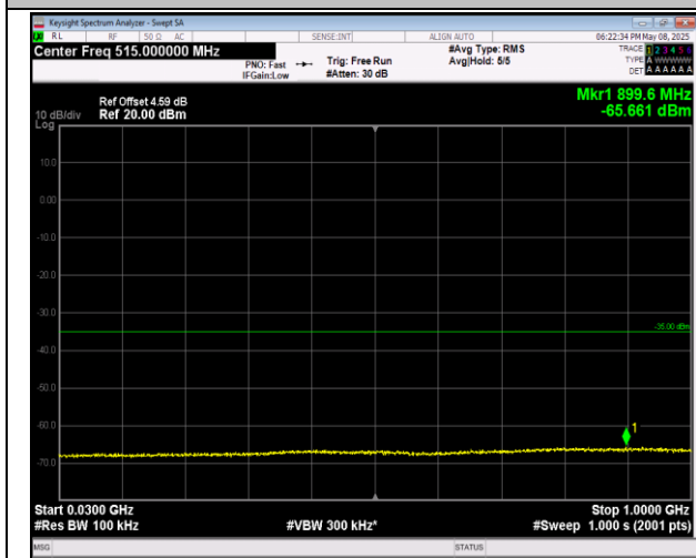
7-7-10MHz-20MHz-16QAM-16QAM-21006-21150-50RB#- 0-100RB#0-30~1000MHz-PASS
