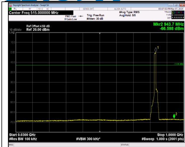
5-5-10MHz-10MHz-16QAM-16QAM-20501-20600-1RB#0 -ORB#0-30~1000MHz-PASS
