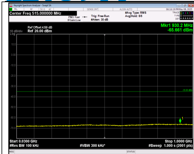
7-7-10MHz-20MHz-16QAM-16QAM-20805-20949-1RB#0 -1RB#99-30~1000MHz-PASS
