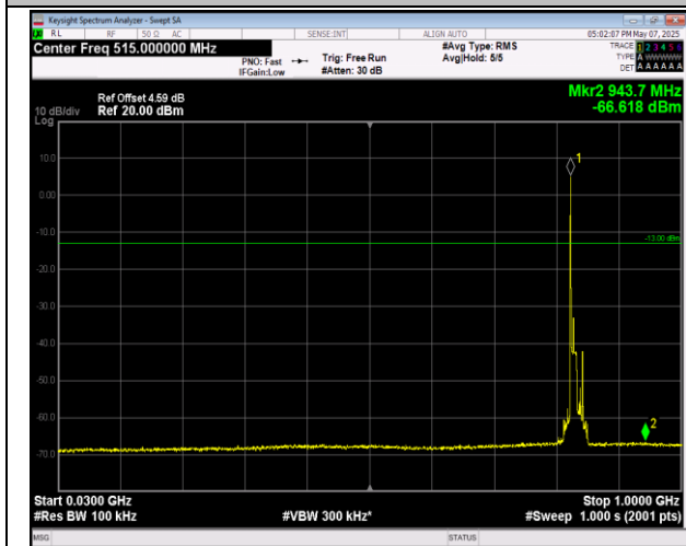
5-5-10MHz-10MHz-QPSK-QPSK-20476-20575-1RB#49-4 ORB#0-30~1000MHz-PASS
