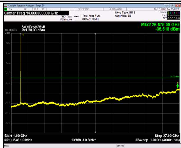
7-7-10MHz-20MHz-16QAM-16QAM-20805-20949-50RB#0- 100RB#0-1000~27000MHz-PASS
