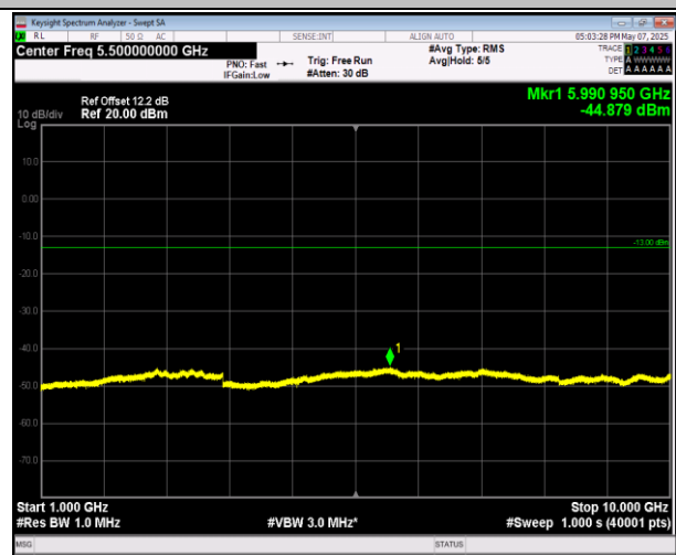
5-5-10MHz-10MHz-16QAM-16QAM-20476-20575-1RB#0-0RB#0-1000~10000MHz-PASS
