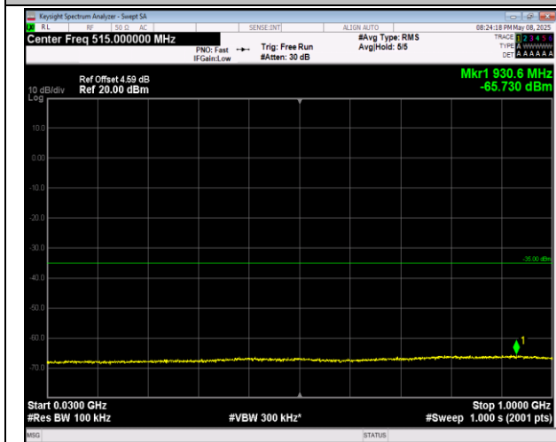
7-7-20MHz-10MHz-QPSK-QPSK-21051-21195-1RB#99-0 RB#0-30~1000MHz-PASS
