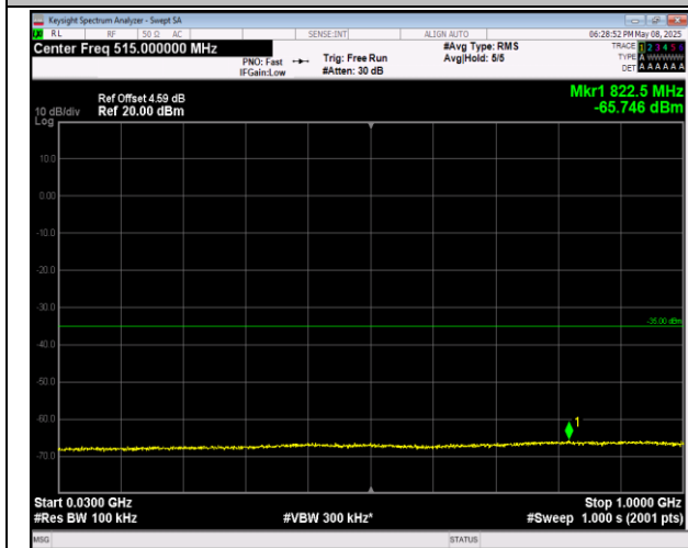
7-7-10MHz-20MHz-16QAM-16QAM-21206-21350-1RB#4 9-ORB#0-30~1000MHz-PASS
