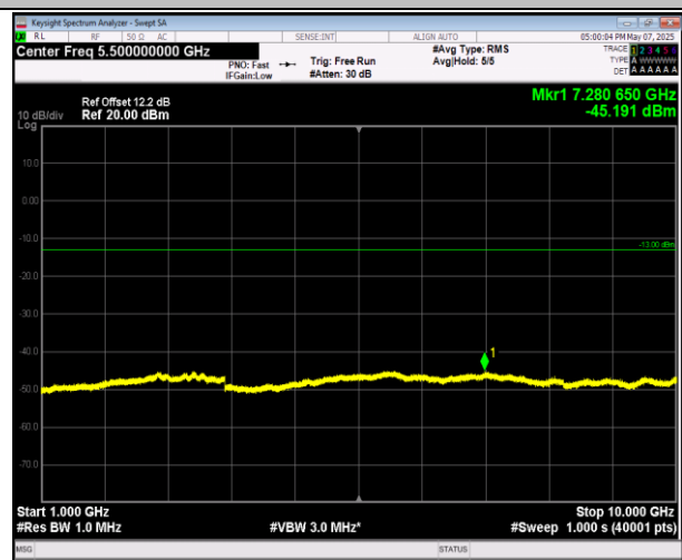
5-5-10MHz-10MHz-QPSK-QPSK-20476-20575-1RB#0-1RB #49-1000~10000MHz-PASS
