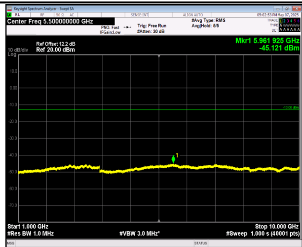
5-5-10MHz-10MHz-16QAM-16QAM-20476-20575-1RB#49- 0RB#0-1000~10000MHz-PASS
