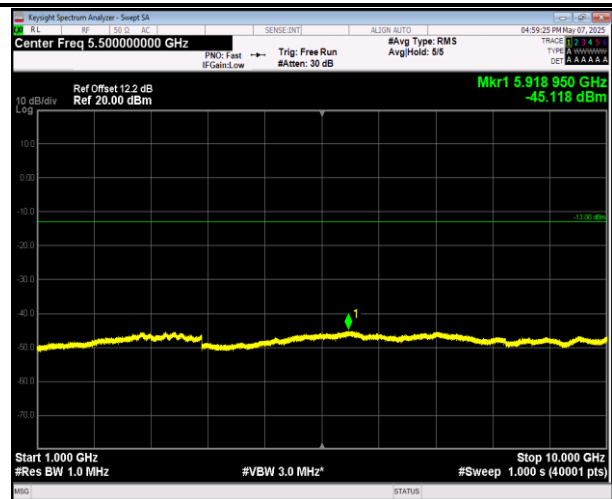
5-5-10MHz-10MHz-QPSK-QPSK-20476-20575-1RB#0-0RB #0-1000~10000MHz-PASS
