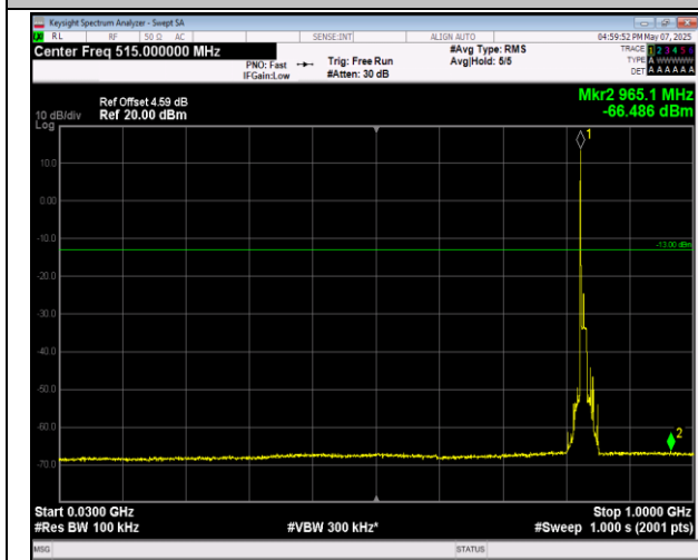
5-5-10MHz-10MHz-QPSK-QPSK-20476-20575-1RB#0-1 RB#49-30~1000MHz-PASS
