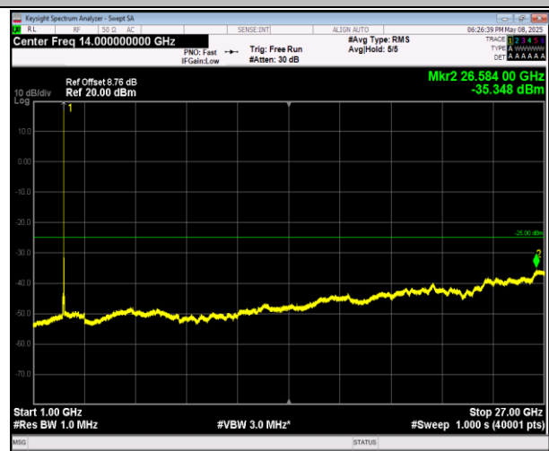
7-7-10MHz-20MHz-16QAM-16QAM-21206-21350-1RB#0-1 RB#99-1000~27000MHz-PASS
