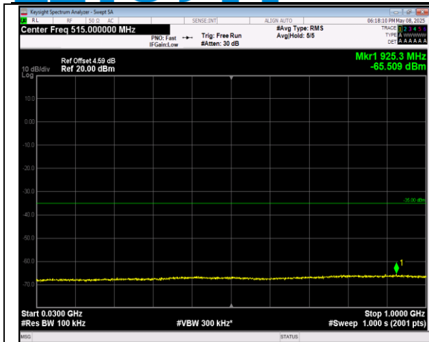
7-7-10MHz-20MHz-QPSK-QPSK-20805-20949-1RB#49-0RB#0-30~1000MHz-PASS
