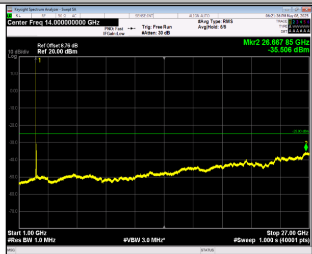
7-7-10MHz-20MHz-16QAM-16QAM-21006-21150-1RB#0-1 RB#99-1000~27000MHz-PASS
