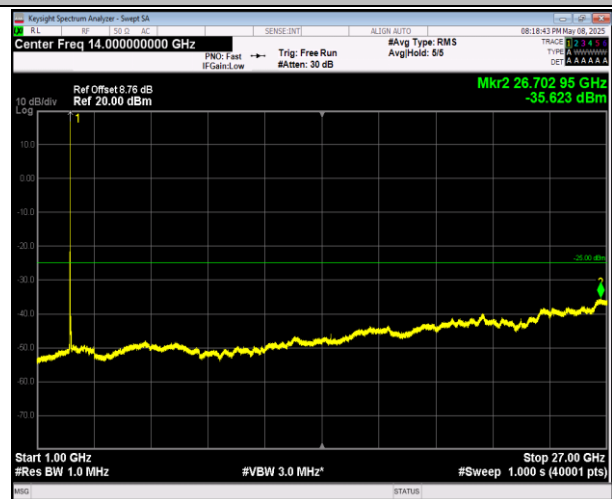
7-7-20MHz-10MHz-16QAM-16QAM-20850-20994-100RB#0 -50RB#0-1000~27000MHz-PASS
