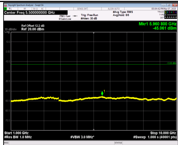
5-5-10MHz-10MHz-QPSK-QPSK-20501-20600-1RB#0-1RB #49-1000~10000MHz-PASS
