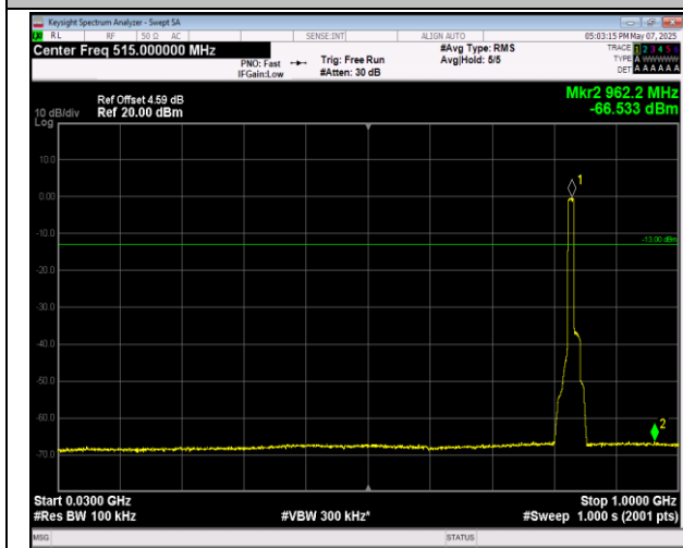
5-5-10MHz-10MHz-16QAM-16QAM-20476-20575-1RB#0-0RB#0-30~1000MHz-PASS
