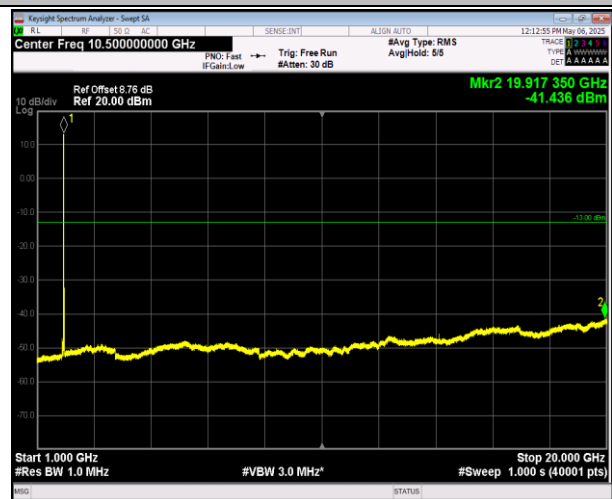
2-2-5MHz-20MHz-16QAM-16QAM-18983-19100-1RB#24-0RB#0-1000~20000MHz-PASS
