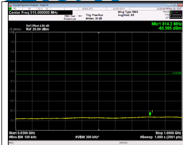
2-2-5MHz-20MHz-QPSK-QPSK-18633-18750-1RB#24-0 RB#0-30~1000MHz-PASS
