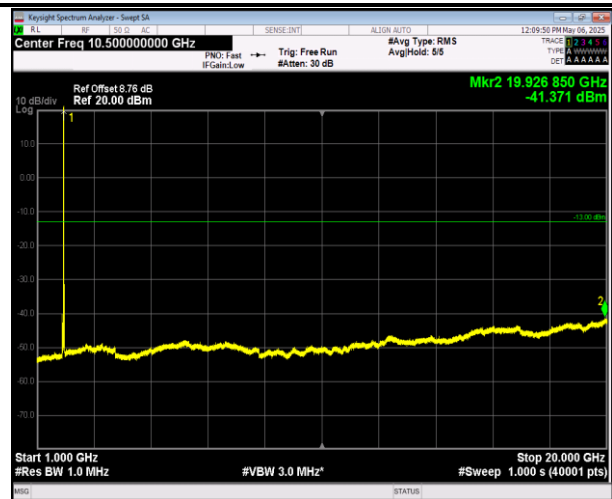
2-2-5MHz-20MHz-QPSK-QPSK-18983-19100-1RB#0-1RB# 99-1000~20000MHz-PASS
