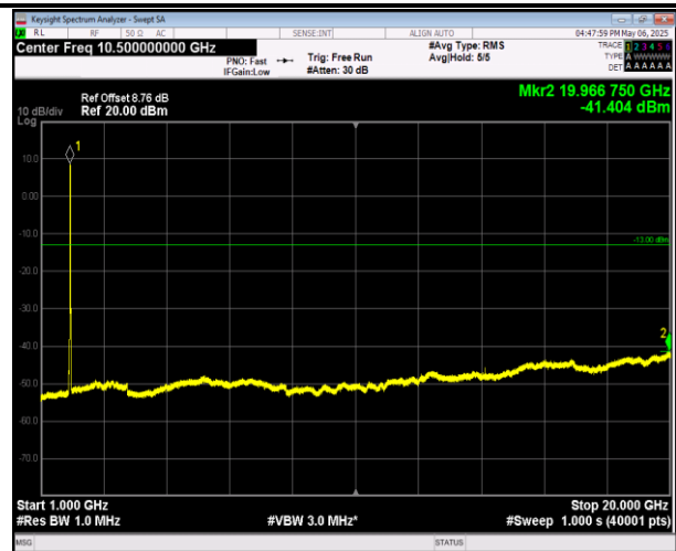
2-2-20MHz-20MHz-16QAM-16QAM-18902-19100-1RB#0-0 RB#0-1000~20000MHz-PASS
