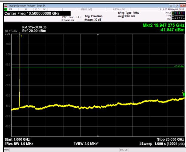
2-2-5MHz-20MHz-QPSK-QPSK-18983-19100-25RB#0-100 RB#0-1000~20000MHz-PASS
