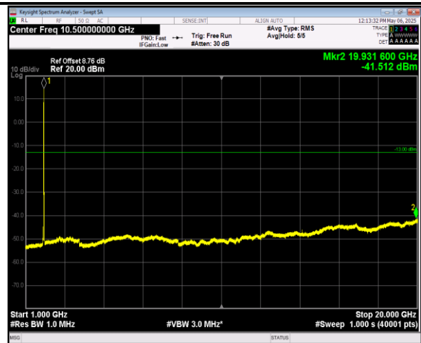
2-2-5MHz-20MHz-16QAM-16QAM-18983-19100-1RB#0-0RB#0-1000~20000MHz-PASS
