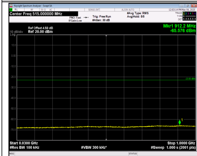
2-2-5MHz-20MHz-16QAM-16QAM-18633-18750-1RB#0-0 ORB#0-30~1000MHz-PASS
