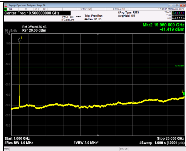
2-2-5MHz-20MHz-QPSK-QPSK-18633-18750-1RB#24-0RB #0-1000~20000MHz-PASS
