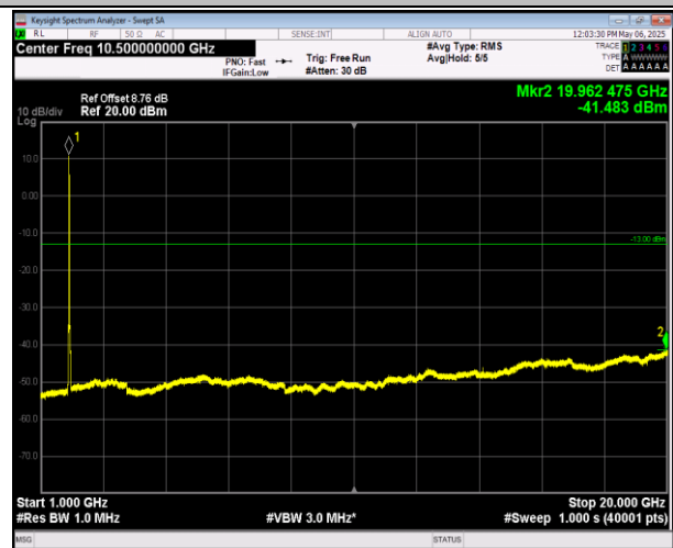
2-2-5MHz-20MHz-16QAM-16QAM-18633-18750-1RB#0-0RB B#0-1000~20000MHz-PASS
