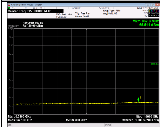
2-2-5MHz-20MHz-16QAM-16QAM-18983-19100-1RB#24-0RB#0-30~1000MHz-PASS
