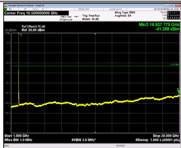
2-2-20MHz-20MHz-16QAM-16QAM-18700-18898-100RB#0 -100RB#0-1000~20000MHz-PASS
