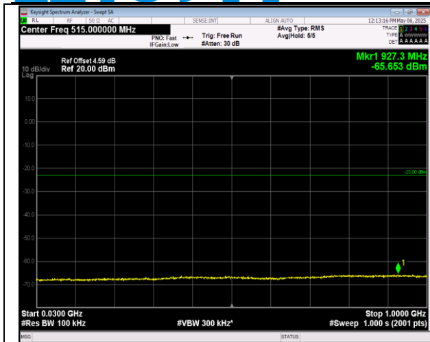
2-2-5MHz-20MHz-16QAM-16QAM-18983-19100-1RB#0-0RB#0-30~1000MHz-PASS
