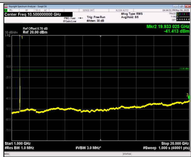
2-2-20MHz-20MHz-16QAM-16QAM-18902-19100-1RB#0-1 RB#99-1000~20000MHz-PASS
