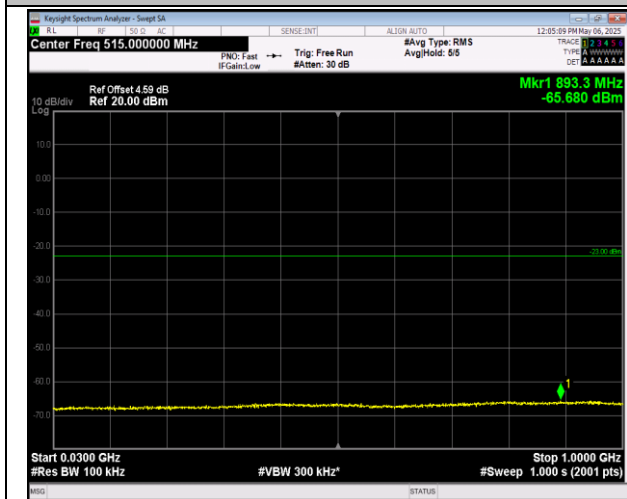
2-2-5MHz-20MHz-16QAM-16QAM-18808-18925-1RB#0-0 1RB#99-30~1000MHz-PASS
