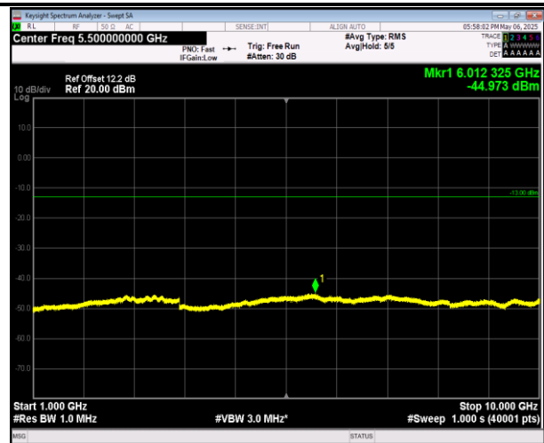
5-5-3MHz-5MHz-QPSK-QPSK-20416-20455-1RB#14-0RB# 0-1000~10000MHz-PASS
