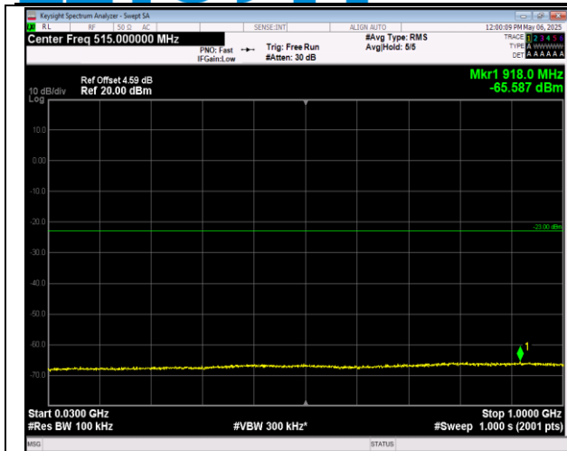
2-2-5MHz-20MHz-16QAM-16QAM-18633-18750-1RB#0-1RB#99-30~1000MHz-PASS
