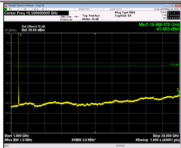
2-2-5MHz-20MHz-16QAM-16QAM-18633-18750-25RB#0-100RB#0-1000~20000MHz-PASS
