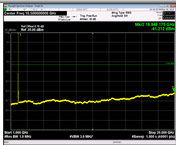
2-2-20MHz-20MHz-16QAM-16QAM-18801-18999-100RB#0 -100RB#0-1000~20000MHz-PASS
