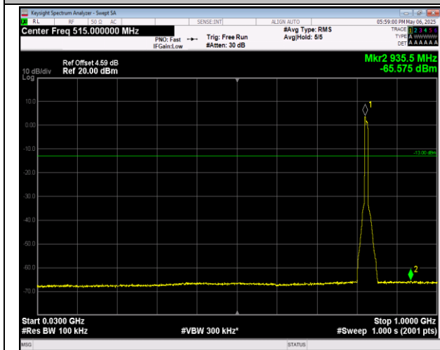
5-5-3MHz-5MHz-16QAM-16QAM-20416-20455-1RB#0-0 RB#0-30~1000MHz-PASS
