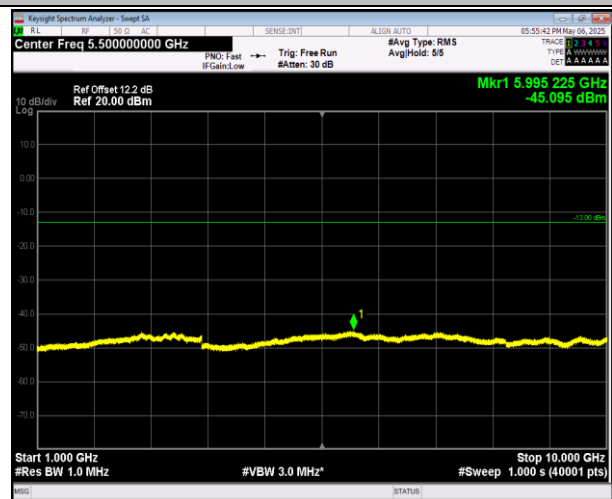
5-5-3MHz-5MHz-QPSK-QPSK-20416-20455-1RB#0-1RB#2 4-1000~10000MHz-PASS
