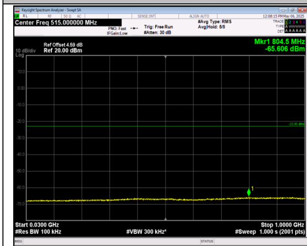
2-2-5MHz-20MHz-16QAM-16QAM-18808-18925-1RB#0-0 0RB#0-30~1000MHz-PASS
