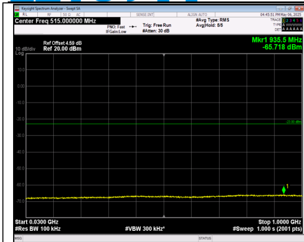
2-2-20MHz-20MHz-16QAM-16QAM-18902-19100-100RB #0-100RB#0-30~1000MHz-PASS
