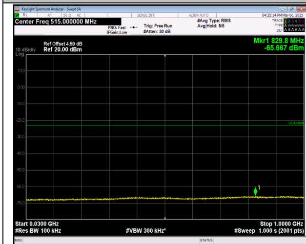
2-2-20MHz-20MHz-16QAM-16QAM-18700-18898-100RB #0-100RB#0-30~1000MHz-PASS
