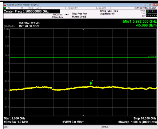
5-5-3MHz-5MHz-16QAM-16QAM-20416-20455-1RB#0-0R B#0-1000~10000MHz-PASS
