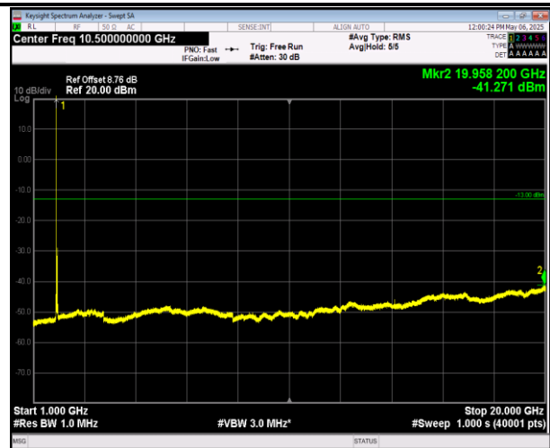
2-2-5MHz-20MHz-16QAM-16QAM-18633-18750-1RB#0-1RB#99-1000~20000MHz-PASS
