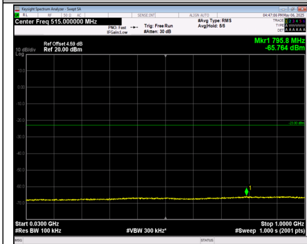
2-2-20MHz-20MHz-16QAM-16QAM-18902-19100-1RB#99 9-ORB#0-30~1000MHz-PASS
