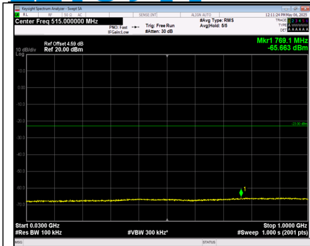
2-2-5MHz-20MHz-16QAM-16QAM-18983-19100-25RB#0 -100RB#0-30~1000MHz-PASS
