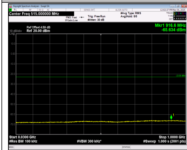
2-2-5MHz-20MHz-16QAM-16QAM-18633-18750-1RB#24-0-0RB#0-30~1000MHz-PASS
