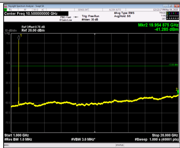
2-2-5MHz-20MHz-QPSK-QPSK-18983-19100-1RB#24-0RB #0-1000~20000MHz-PASS
