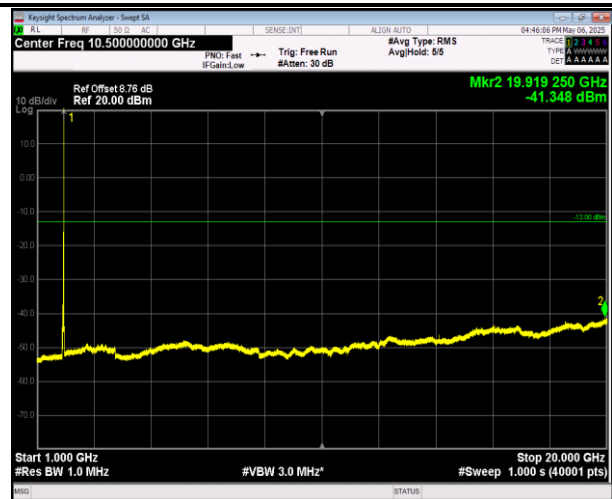
2-2-20MHz-20MHz-16QAM-16QAM-18902-19100-100RB#0 -100RB#0-1000~20000MHz-PASS
