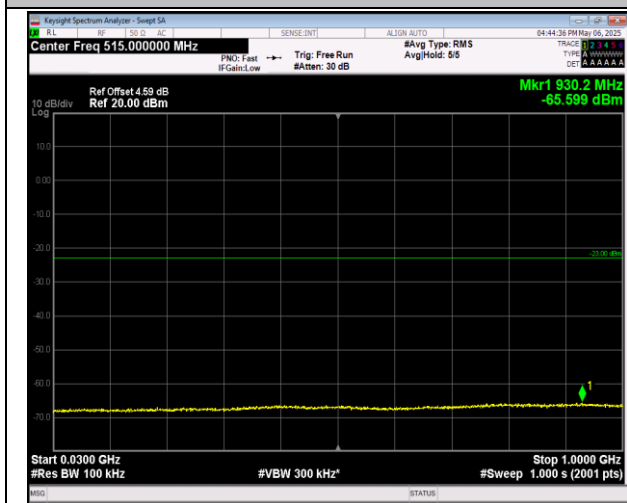
2-2-20MHz-20MHz-16QAM-16QAM-18902-19100-1RB#0 -1RB#99-30~1000MHz-PASS
