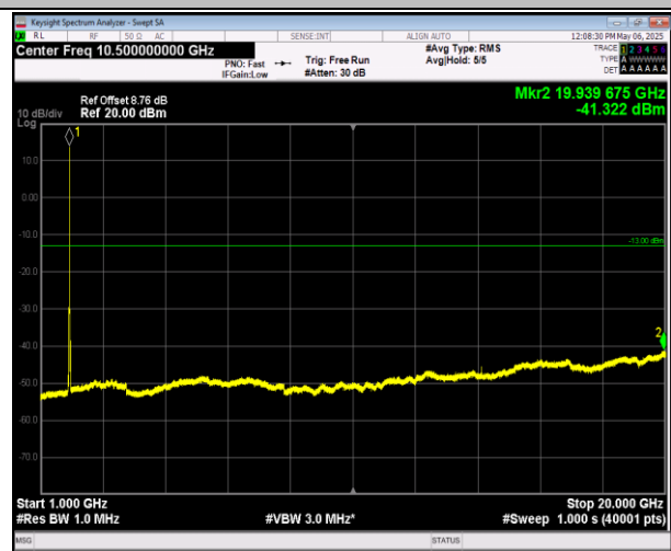
2-2-5MHz-20MHz-16QAM-16QAM-18808-18925-1RB#0-0R B#0-1000~20000MHz-PASS
