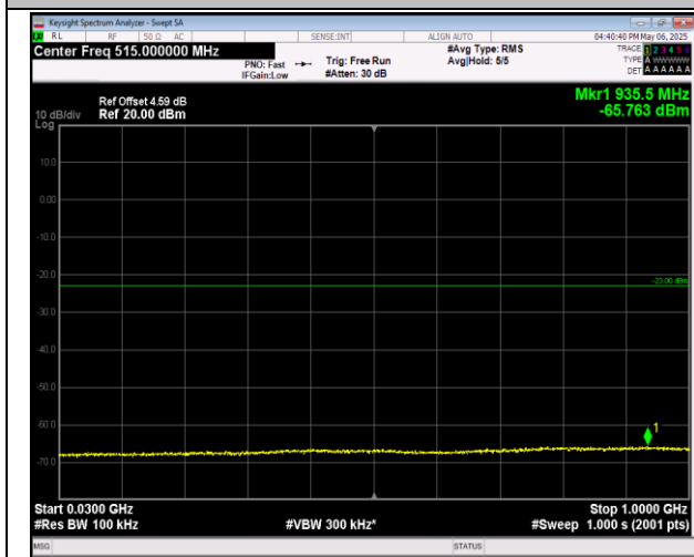
2-2-20MHz-20MHz-16QAM-16QAM-18801-18999-100RB #0-100RB#0-30~1000MHz-PASS
