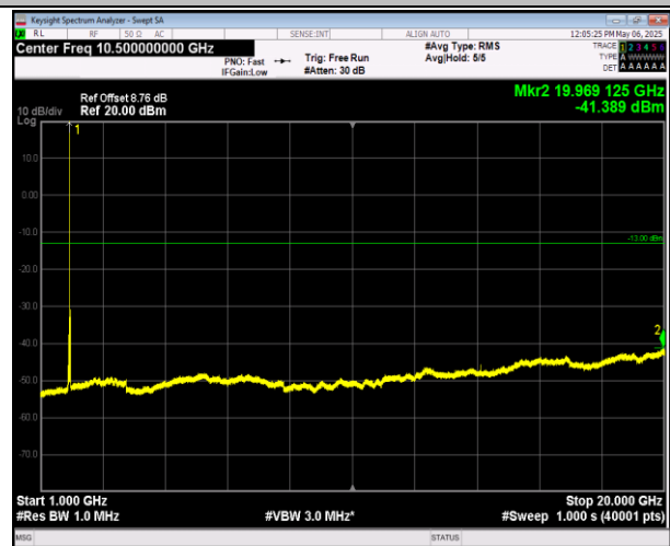
2-2-5MHz-20MHz-16QAM-16QAM-18808-18925-1RB#0-1R B#99-1000~20000MHz-PASS
