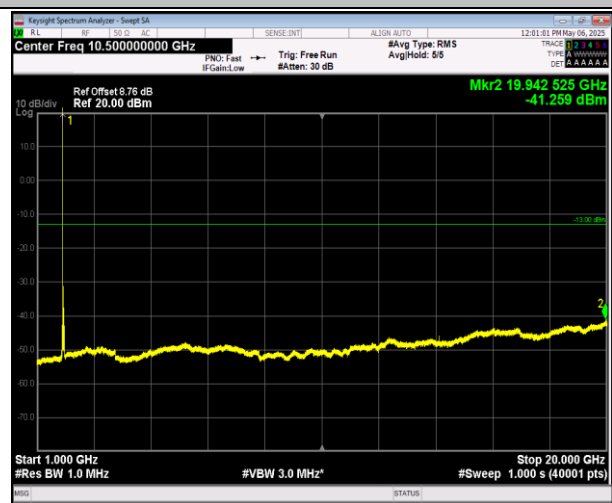
2-2-5MHz-20MHz-QPSK-QPSK-18633-18750-25RB#0-100 RB#0-1000~20000MHz-PASS
