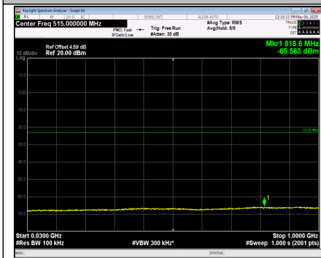
2-2-5MHz-20MHz-16QAM-16QAM-18983-19100-1RB#0-1RB#99-30~1000MHz-PASS
