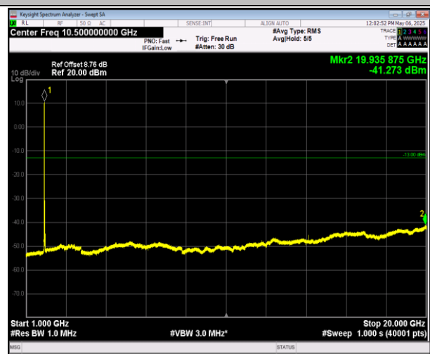
2-2-5MHz-20MHz-16QAM-16QAM-18633-18750-1RB#24-0RB#0-1000~20000MHz-PASS
