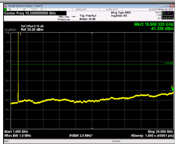
2-2-5MHz-20MHz-16QAM-16QAM-18983-19100-1RB#0-1RB#99-1000~20000MHz-PASS
