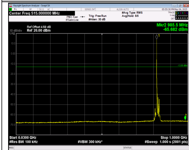
5-5-3MHz-5MHz-QPSK-QPSK-20416-20455-1RB#0-1RB #24-30~1000MHz-PASS
