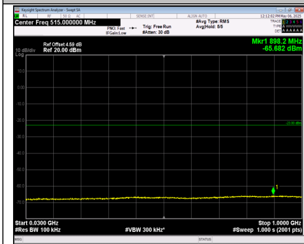
2-2-5MHz-20MHz-QPSK-QPSK-18983-19100-1RB#24-0 RB#0-30~1000MHz-PASS
