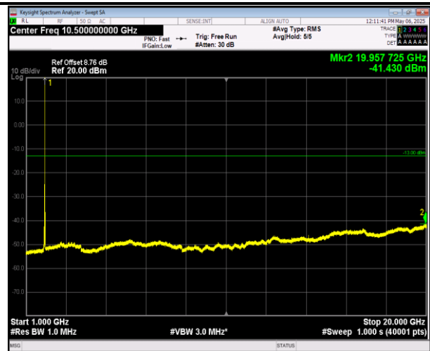
2-2-5MHz-20MHz-16QAM-16QAM-18983-19100-25RB#0-1 00RB#0-1000~20000MHz-PASS
