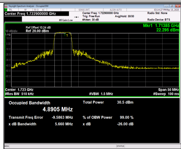
66-66-5MHz-20MHz-16QAM-16QAM-132330-132447-25R B#0-100RB#0-PASS
