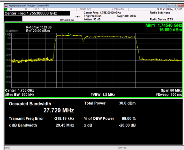
66-66-10MHz-20MHz-16QAM-16QAM-132428-132572-50R B#0-100RB#0-PASS
