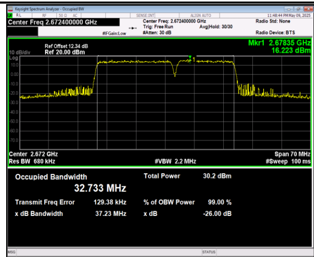
41-41-20MHz-20MHz-16QAM-16QAM-39750-39948-100RB B#0-100RB#0-PASS
