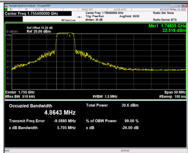
66-66-5MHz-20MHz-16QAM-16QAM-132455-132572-25R B#0-100RB#0-PASS
