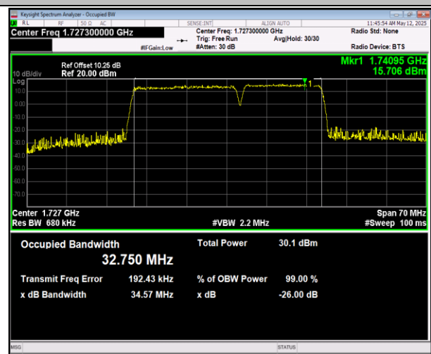
66-66-20MHz-15MHz-16QAM-16QAM-132348-132519-100 RB#0-75RB#0-PASS
