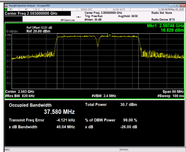
41-41-20MHz-20MHz-16QAM-16QAM-41292-41490-100RB B#0-100RB#0-PASS
