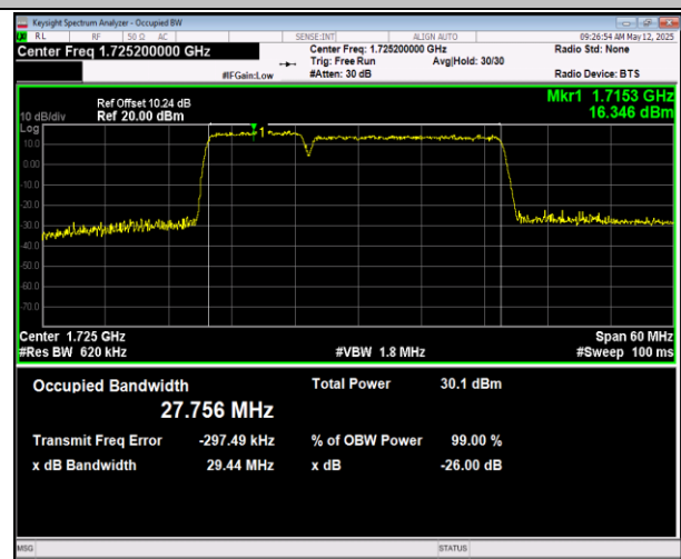
66-66-10MHz-20MHz-16QAM-16QAM-132328-132472-50R B#0-100RB#0-PASS
