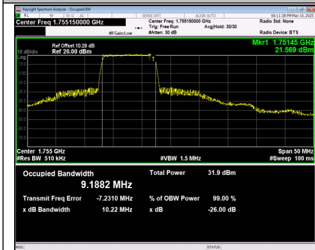
66-66-10MHz-15MHz-QPSK-QPSK-132477-132597-50R B#0-75RB#0-PASS
