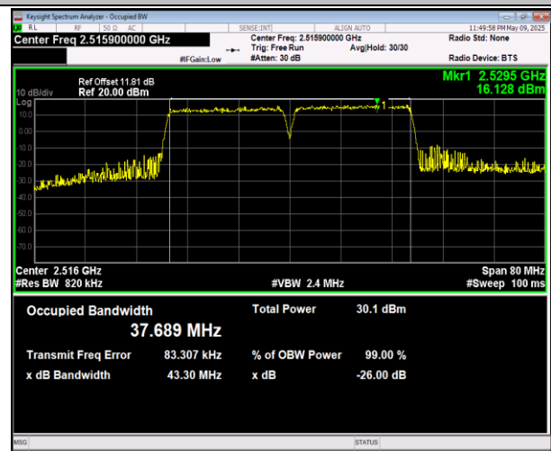
41-41-20MHz-20MHz-16QAM-16QAM-40521-40719-100RB B#0-100RB#0-PASS
