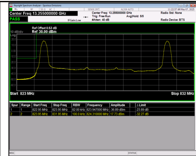
5-5-5MHz-3MHz-QPSK@QPSK-QPSK@QPSK-20425-20 464-25RB#0@25RB#0-15RB#0@15RB#0-PASS
