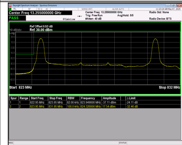
5-5-5MHz-3MHz-16QAM@16QAM-16QAM@16QAM-2042 5-20464-25RB#0@25RB#0-15RB#0@15RB#0-PASS
