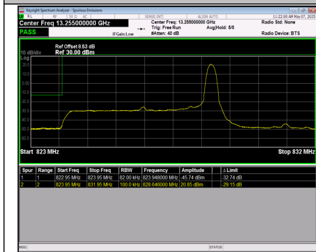
5-5-5MHz-3MHz-16QAM@16QAM-16QAM@16QAM-2042 5-20464- 1RB#0@25RB#0-ORB#0@15RB#0-PASS
