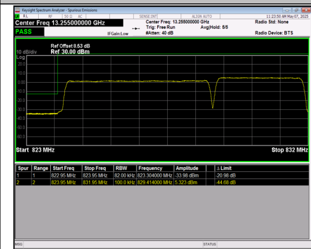
5-5-5MHz-3MHz-16QAM@16QAM-16QAM@16QAM-2042 5-20464-1RB#0@25RB#0-1RB#15@15RB#0-PASS
