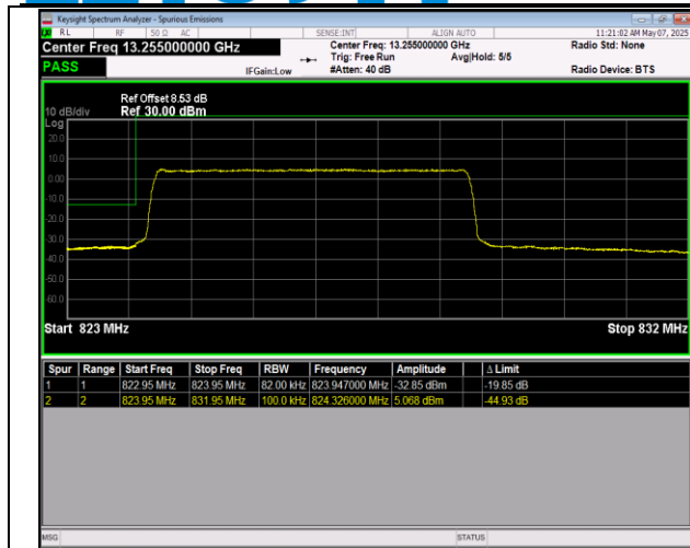
5-5-5MHz-3MHz-QPSK@QPSK-QPSK@QPSK-20425-20 464-1RB#24@25RB#0-ORB#0@15RB#0-PASS
