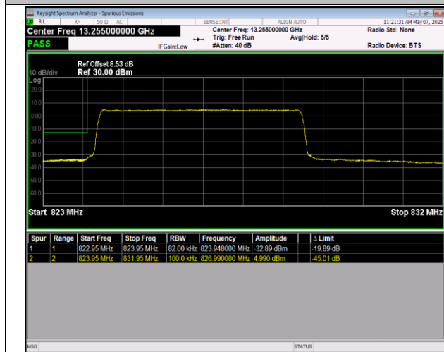
5-5-5MHz-3MHz-16QAM@16QAM-16QAM@16QAM-2042 5-20464-1RB#24@25RB#0-ORB#0@15RB#0-PASS
