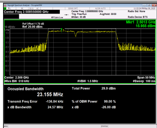
41-41-10MHz-15MHz-16QAM-16QAM-40549-40669-50RB #0-75RB#0-PASS
