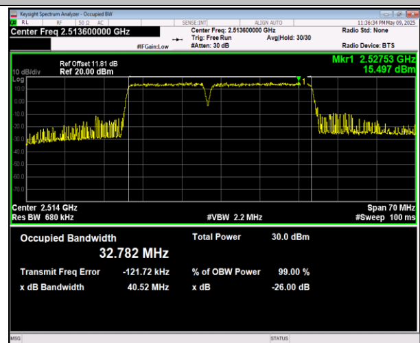
41-41-15MHz-20MHz-16QAM-16QAM-40523-40694-75RB #0-100RB#0-PASS
