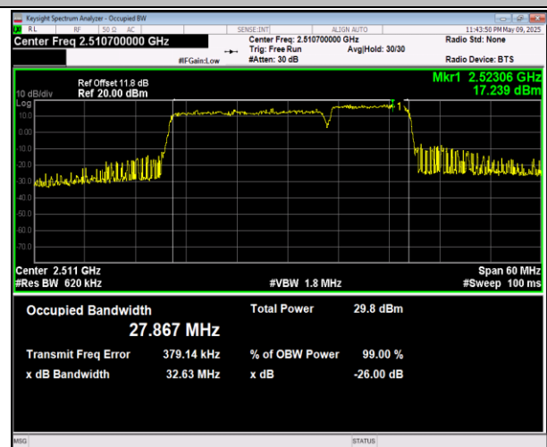
41-41-20MHz-10MHz-16QAM-16QAM-40571-40715-100R B#0-50RB#0-PASS
