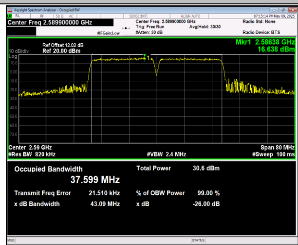
38-38-20MHz-20MHz-16QAM-16QAM-37901-38099-100RB B#0-100RB#0-PASS
