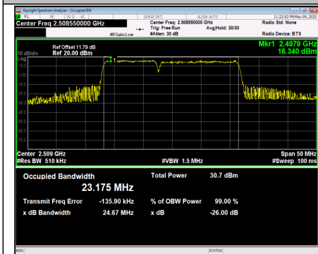
41-41-10MHz-15MHz-QPSK-QPSK-40549-40669-50RB# 0-75RB#0-PASS
