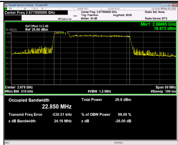
41-41-10MHz-15MHz-16QAM-16QAM-39703-39823-50RB #0-75RB#0-PASS
