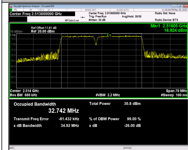
41-41-15MHz-20MHz-QPSK-QPSK-40523-40694-75RB# 0-100RB#0-PASS
