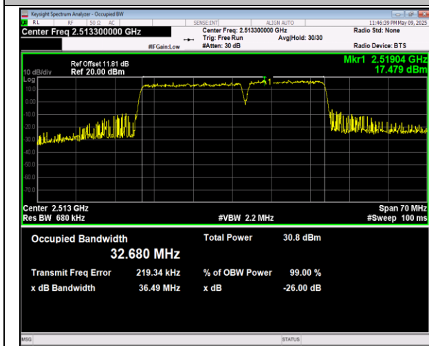
41-41-20MHz-15MHz-QPSK-QPSK-40546-40717-100RB #0-75RB#0-PASS
