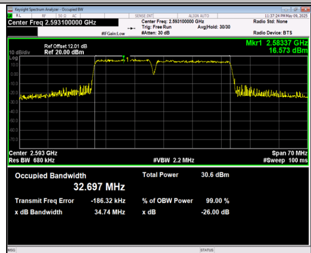
41-41-15MHz-20MHz-16QAM-16QAM-41319-41490-75RB #0-100RB#0-PASS
