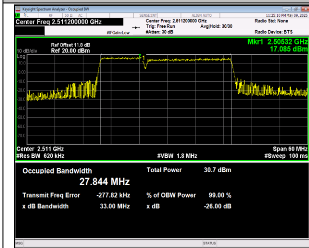
41-41-10MHz-20MHz-QPSK-QPSK-40526-40670-50RB# 0-100RB#0-PASS
