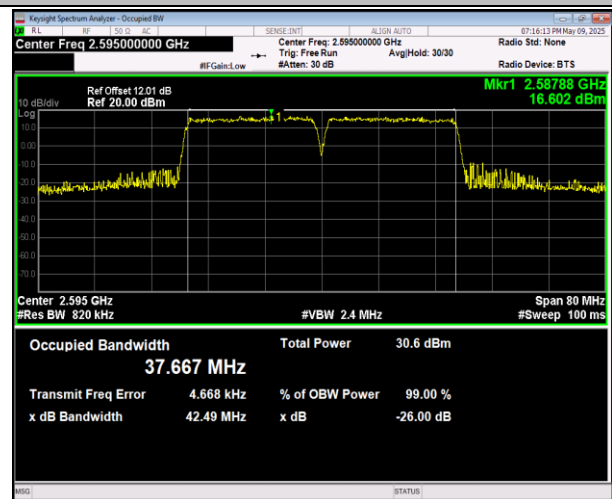
38-38-20MHz-20MHz-16QAM-16QAM-37952-38150-100RB B#0-100RB#0-PASS
