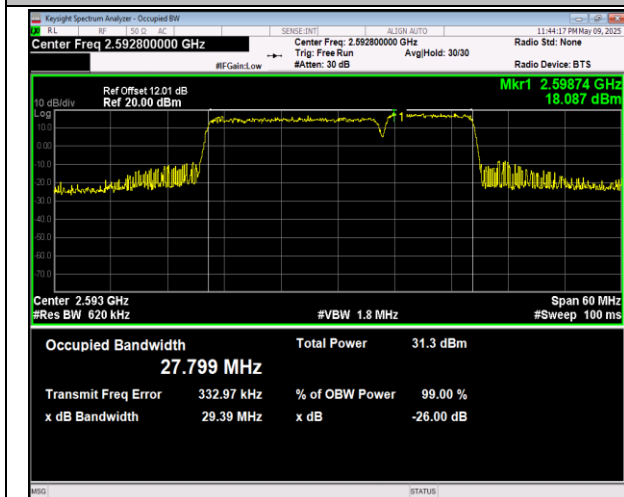
41-41-20MHz-10MHz-QPSK-QPSK-41391-41535-100RB #0-50RB#0-PASS
