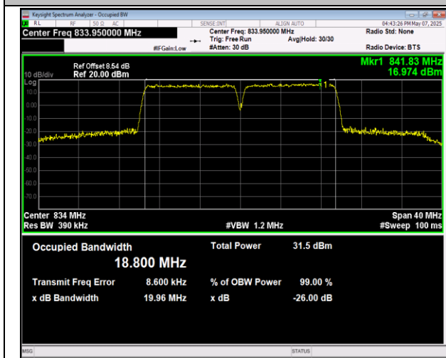
5-5-10MHz-10MHz-QPSK-QPSK-20476-20575-50RB#0-50RB#0-PASS
