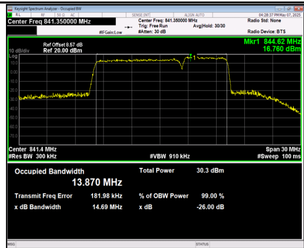
5-5-10MHz-10MHz-16QAM-16QAM-20450-20549-50RB#0-50RB#0-PASS
