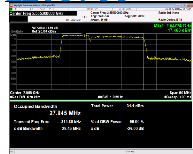
7-7-15MHz-10MHz-QPSK-QPSK-20825-20945-75RB#0-50RB#0-PASS
