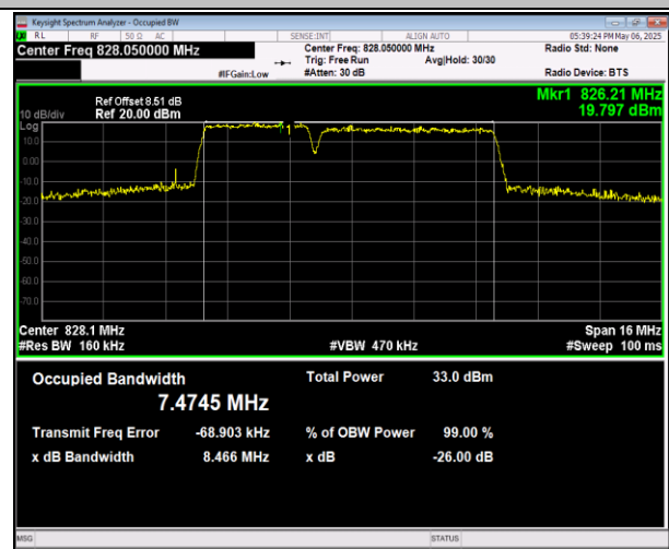
5-5-3MHz-5MHz-16QAM-16QAM-20501-20540-15RB#0-25 RB#0-PASS
