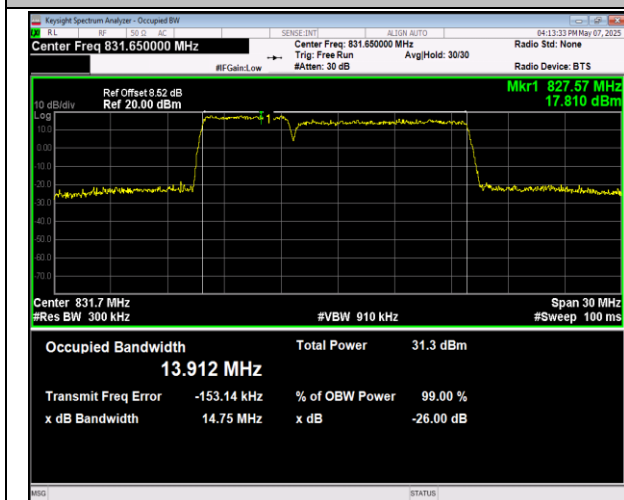
5-5-5MHz-10MHz-QPSK-QPSK-20478-20550-25RB#0-5 ORB#0-PASS
