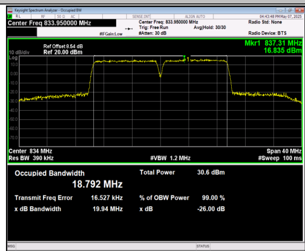
5-5-10MHz-10MHz-16QAM-16QAM-20476-20575-50RB#0-50RB#0-PASS
