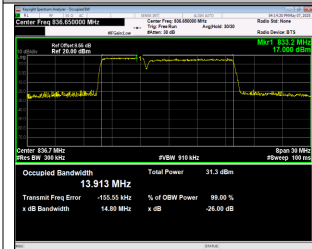
5-5-5MHz-10MHz-QPSK-QPSK-20528-20600-25RB#0-5 ORB#0-PASS
