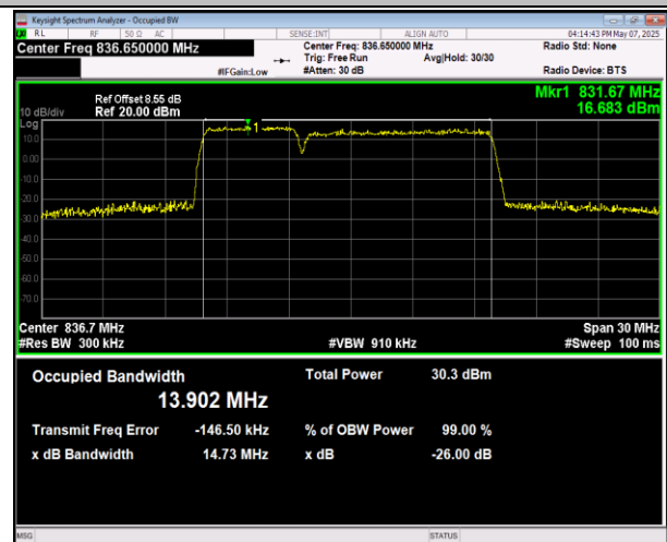
5-5-5MHz-10MHz-16QAM-16QAM-20528-20600-25RB#0-5 ORB#0-PASS
