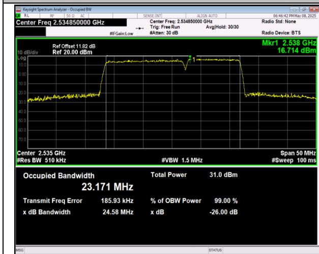
7-7-15MHz-10MHz-QPSK-QPSK-21277-21397-75RB#0-50RB#0-PASS
