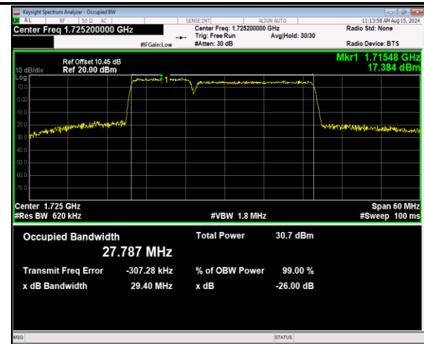
66-66-10MHz-20MHz-16QAM-16QAM-132027-132171-50RB #0-100RB#0-PASS
