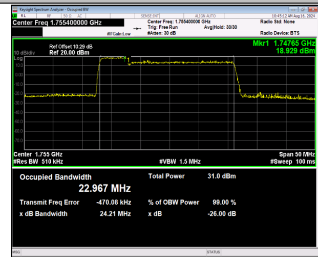
66-66-5MHz-20MHz-QPSK-QPSK-132330-132447-25RB# 0-100RB#0-PASS
