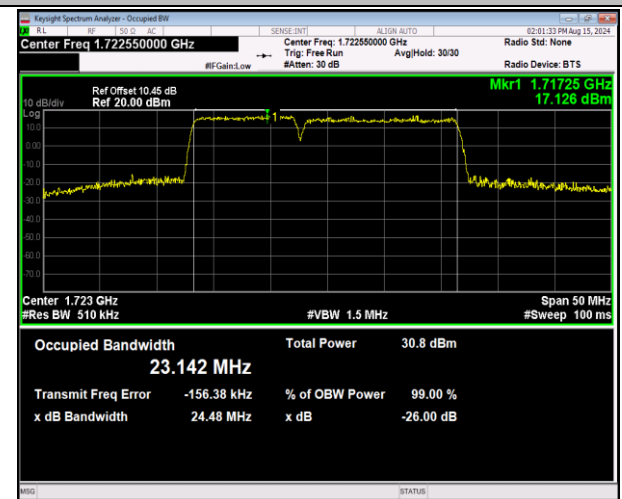
66-66-10MHz-15MHz-64QAM-64QAM-132025-132145-50RB#0-75RB#0-PASS
