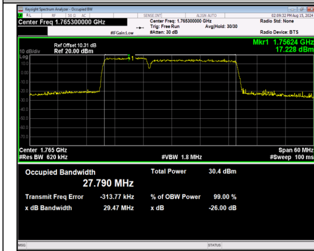
66-66-10MHz-20MHz-64QAM-64QAM-132428-132572-50RB #0-100RB#0-PASS
