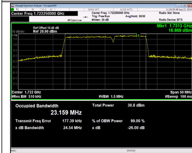
66-66-15MHz-10MHz-16QAM-16QAM-132047-132167-75RB #0-50RB#0-PASS
