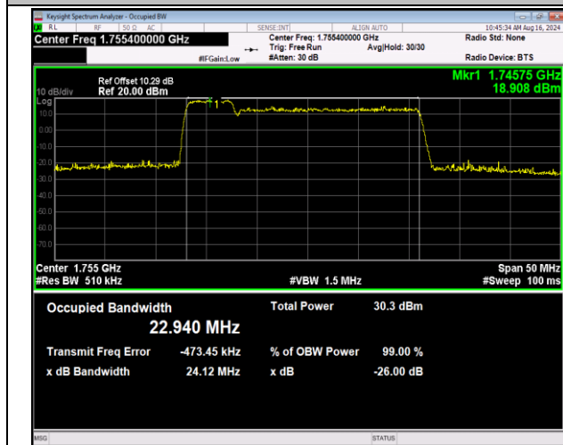
66-66-5MHz-20MHz-16QAM-16QAM-132330-132447-25R B#0-100RB#0-PASS
