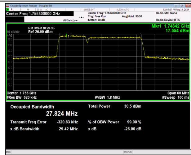
66-66-10MHz-20MHz-64QAM-64QAM-132328-132472-50RB #0-100RB#0-PASS
