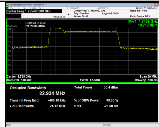
66-66-5MHz-20MHz-64QAM-64QAM-132330-132447-25R B#0-100RB#0-PASS
