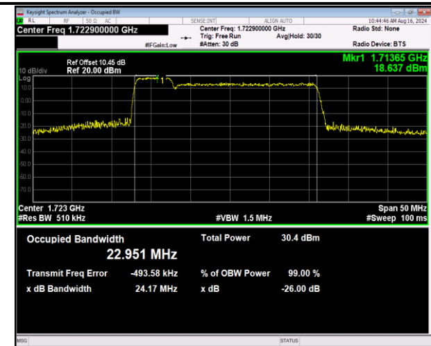
66-66-5MHz-20MHz-16QAM-16QAM-132005-132122-25R B#0-100RB#0-PASS
