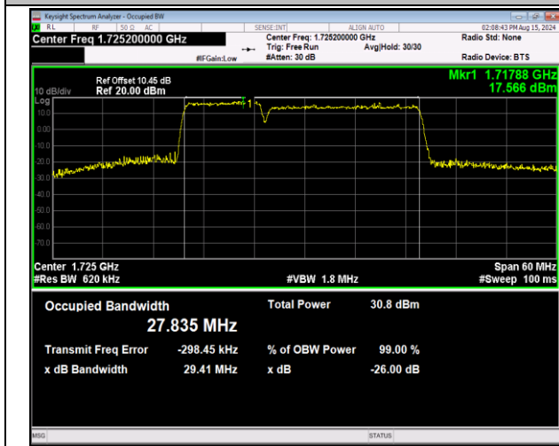
66-66-10MHz-20MHz-64QAM-64QAM-132027-132171-50RB #0-100RB#0-PASS
