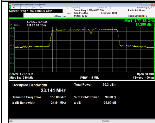
66-66-15MHz-10MHz-16QAM-16QAM-132499-132619-75RB #0-50RB#0-PASS
