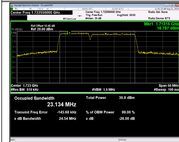
66-66-10MHz-15MHz-16QAM-16QAM-132025-132145-50RB#0-75RB#0-PASS
