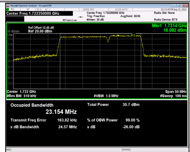
66-66-15MHz-10MHz-64QAM-64QAM-132047-132167-75RB #0-50RB#0-PASS
