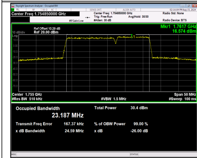
66-66-15MHz-10MHz-64QAM-64QAM-132373-132493-75RB #0-50RB#0-PASS
