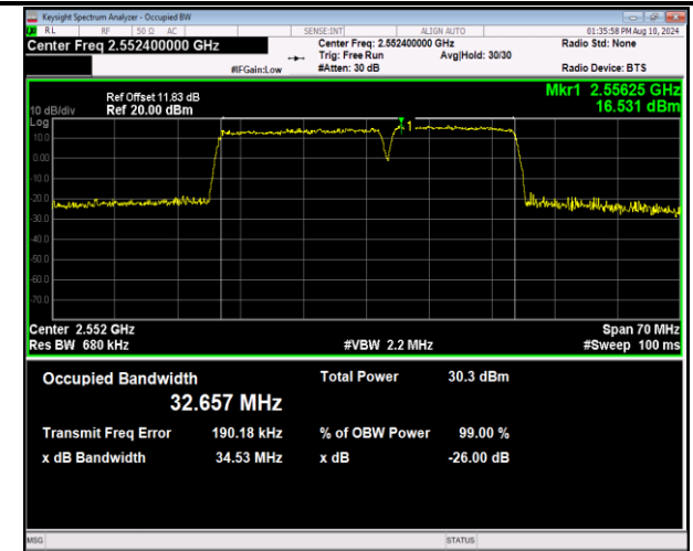
7-7-20MHz-15MHz-16QAM-16QAM-21201-21372-100RB#0-75RB#0-PASS
