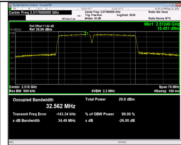
7-7-15MHz-20MHz-16QAM-16QAM-20828-20999-75RB#0 -100RB#0-PASS
