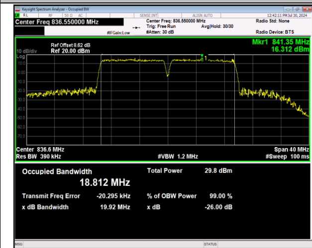
5-5-10MHz-10MHz-64QAM-64QAM-20476-20575-50RB#0-5 -50RB#0-PASS
