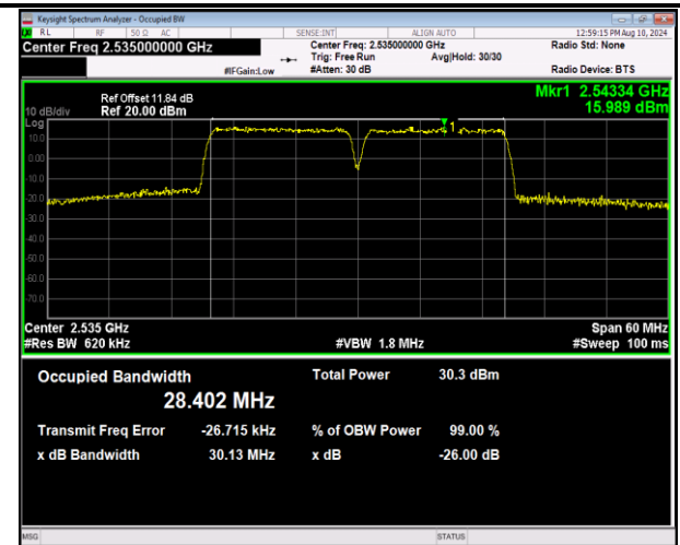
7-7-15MHz-15MHz-16QAM-16QAM-21025-21175-75RB#0-7 -75RB#0-PASS
