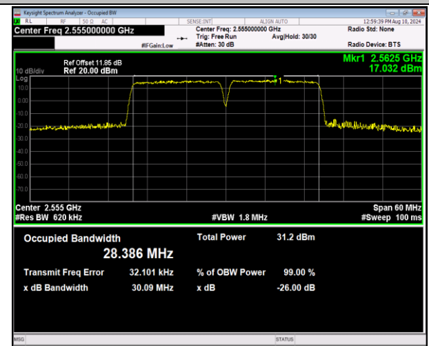
7-7-15MHz-15MHz-QPSK-QPSK-21225-21375-75RB#0-7 5RB#0-PASS
