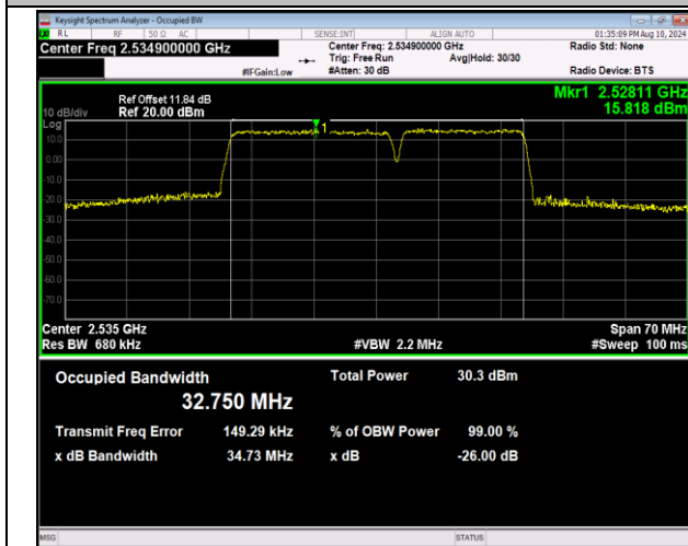
7-7-20MHz-15MHz-16QAM-16QAM-21026-21197-100RB#0-75RB#0-PASS
