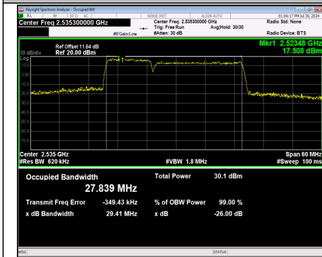
7-7-10MHz-20MHz-64QAM-64QAM-21006-21150-50RB#0-100RB#0-PASS
