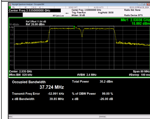
7-7-20MHz-20MHz-64QAM-64QAM-21001-21199-100RB#0-100RB#0-PASS
