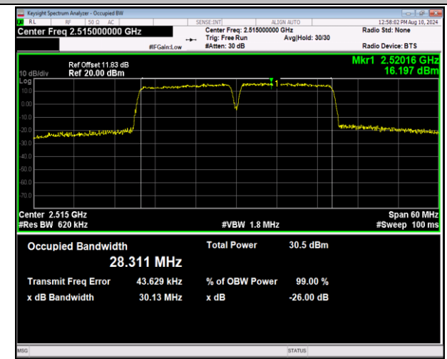
7-7-15MHz-15MHz-QPSK-QPSK-20825-20975-75RB#0-7 5RB#0-PASS
