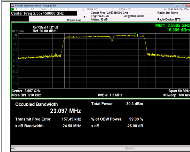
7-7-15MHz-10MHz-64QAM-64QAM-21277-21397-75RB#0-5 -50RB#0-PASS
