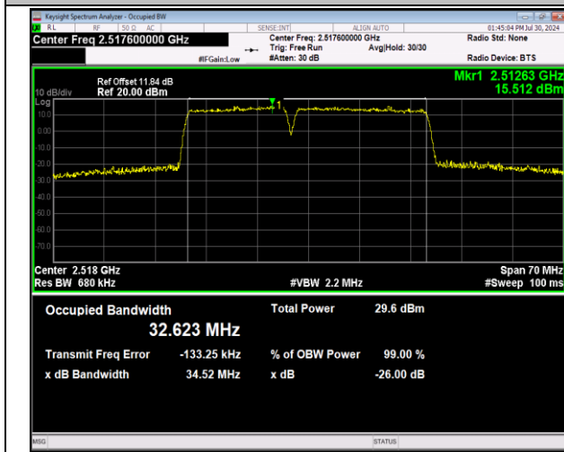
7-7-15MHz-20MHz-64QAM-64QAM-20828-20999-75RB#0 -100RB#0-PASS
