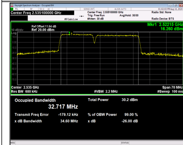
7-7-15MHz-20MHz-16QAM-16QAM-21003-21174-75RB#0 -100RB#0-PASS
