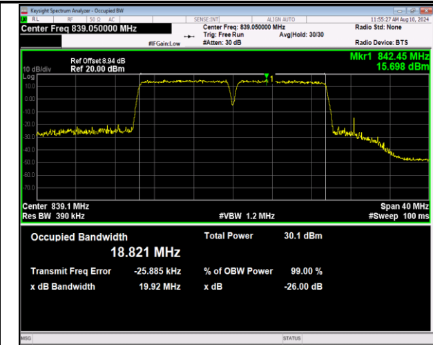
5-5-10MHz-10MHz-16QAM-16QAM-20501-20600-50RB#0-5 -50RB#0-PASS
