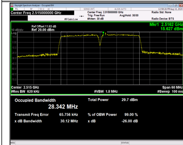
7-7-15MHz-15MHz-16QAM-16QAM-20825-20975-75RB#0-7 -75RB#0-PASS
