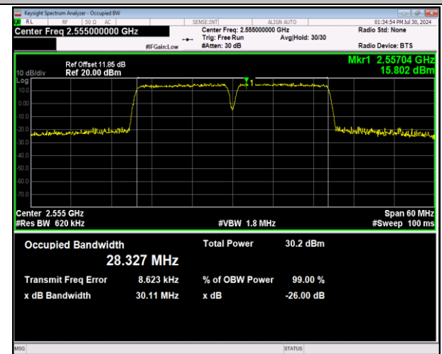
7-7-15MHz-15MHz-64QAM-64QAM-21225-21375-75RB#0-7 -75RB#0-PASS
