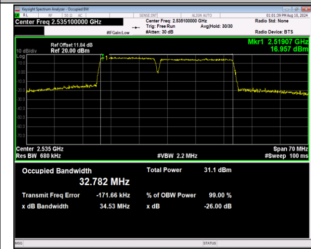
7-7-15MHz-20MHz-QPSK-QPSK-21003-21174-75RB#0-1 00RB#0-PASS
