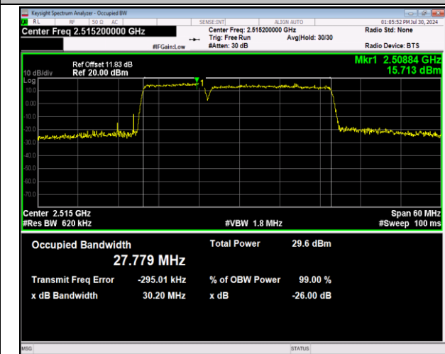
7-7-10MHz-20MHz-64QAM-64QAM-20805-20949-50RB#0-1 -100RB#0-PASS
