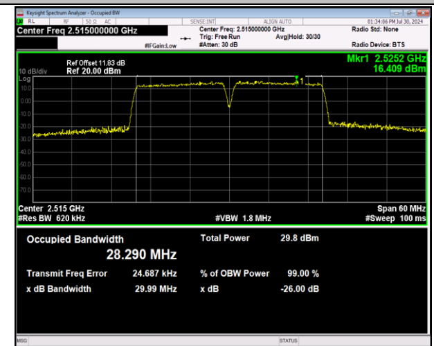
7-7-15MHz-15MHz-64QAM-64QAM-20825-20975-75RB#0-7 -75RB#0-PASS
