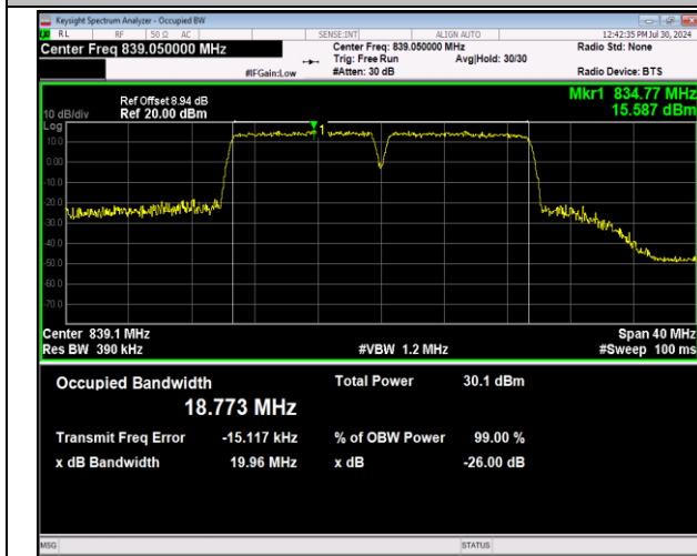
5-5-10MHz-10MHz-64QAM-64QAM-20501-20600-50RB#0-5 -50RB#0-PASS
