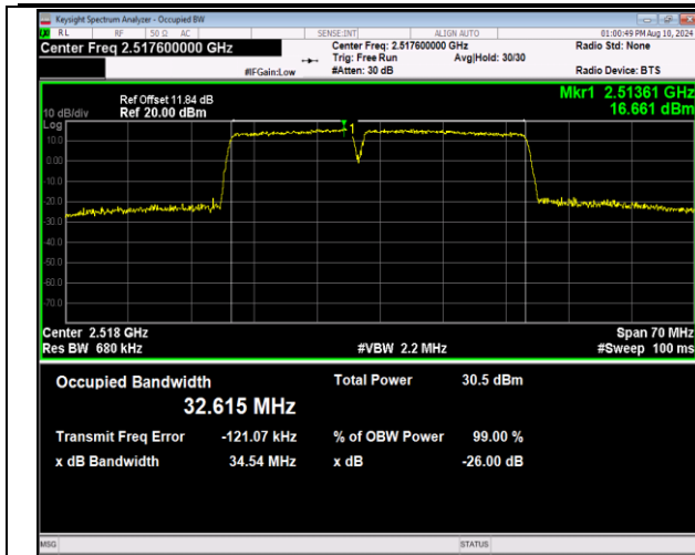
7-7-15MHz-20MHz-QPSK-QPSK-20828-20999-75RB#0-1 00RB#0-PASS
