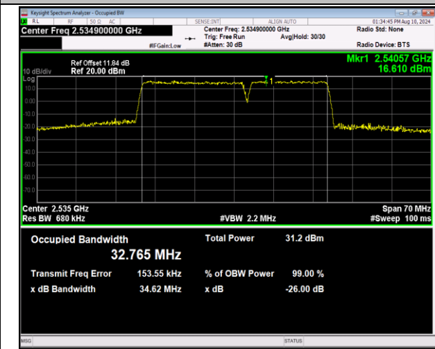
7-7-20MHz-15MHz-QPSK-QPSK-21026-21197-100RB#0-75RB#0-PASS
