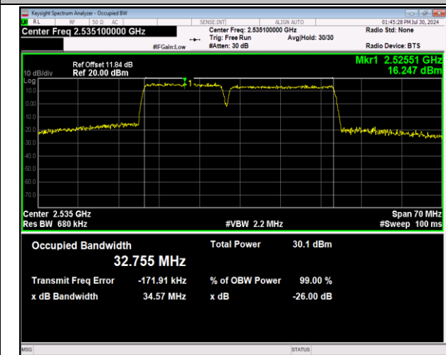
7-7-15MHz-20MHz-64QAM-64QAM-21003-21174-75RB#0 -100RB#0-PASS
