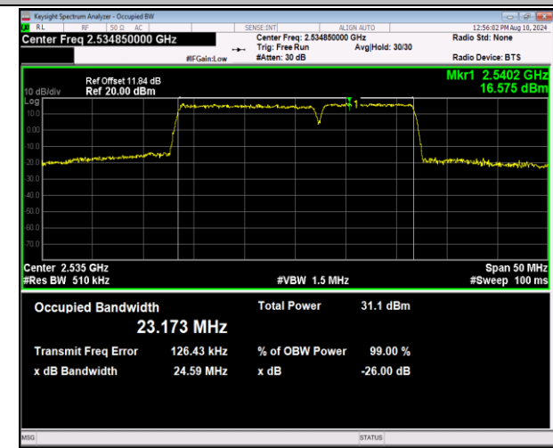
7-7-15MHz-10MHz-QPSK-QPSK-21051-21171-75RB#0-5 ORB#0-PASS
