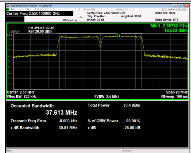
7-7-20MHz-20MHz-64QAM-64QAM-21152-21350-100RB#0-100RB#0-PASS
