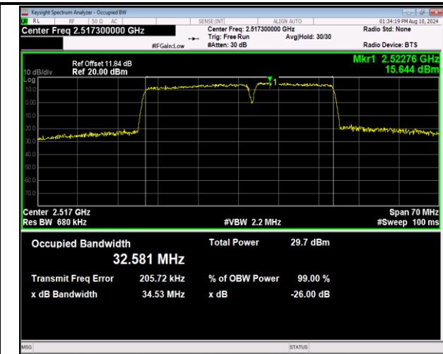
7-7-20MHz-15MHz-16QAM-16QAM-20850-21021-100RB#0-75RB#0-PASS
