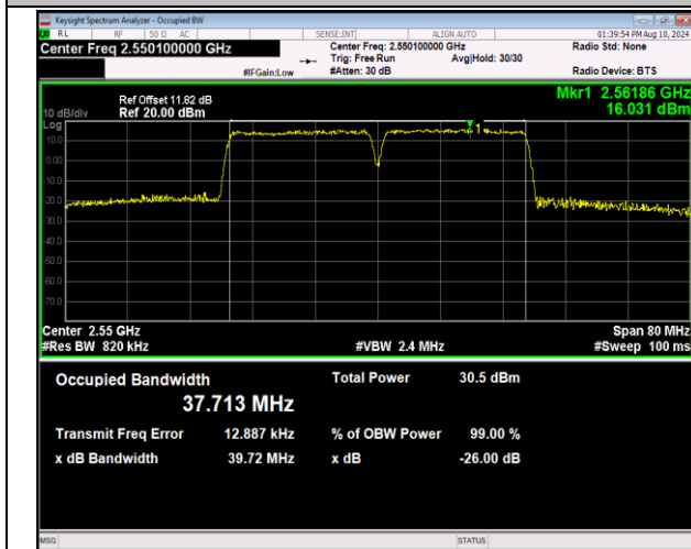
7-7-20MHz-20MHz-16QAM-16QAM-21152-21350-100RB#0-100RB#0-PASS
