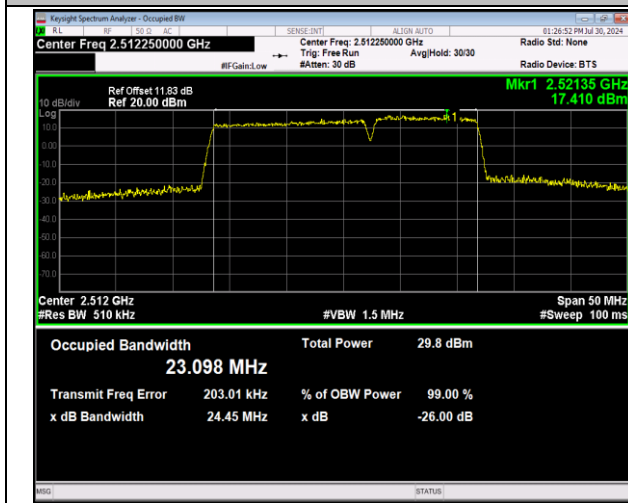
7-7-15MHz-10MHz-64QAM-64QAM-20825-20945-75RB#0-5 -50RB#0-PASS
