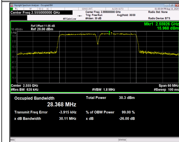
7-7-15MHz-15MHz-16QAM-16QAM-21225-21375-75RB#0-7 -75RB#0-PASS
