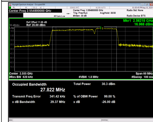
7-7-20MHz-10MHz-16QAM-16QAM-21251-21395-100RB#0-50RB#0-PASS
