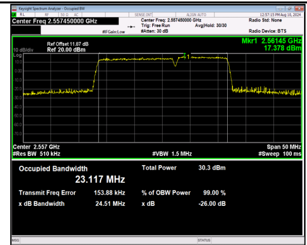
7-7-15MHz-10MHz-16QAM-16QAM-21277-21397-75RB#0-5 -50RB#0-PASS
