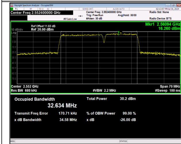
7-7-20MHz-15MHz-64QAM-64QAM-21201-21372-100RB#0-75RB#0-PASS
