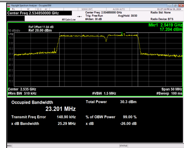
7-7-15MHz-10MHz-64QAM-64QAM-21051-21171-75RB#0-5 -50RB#0-PASS
