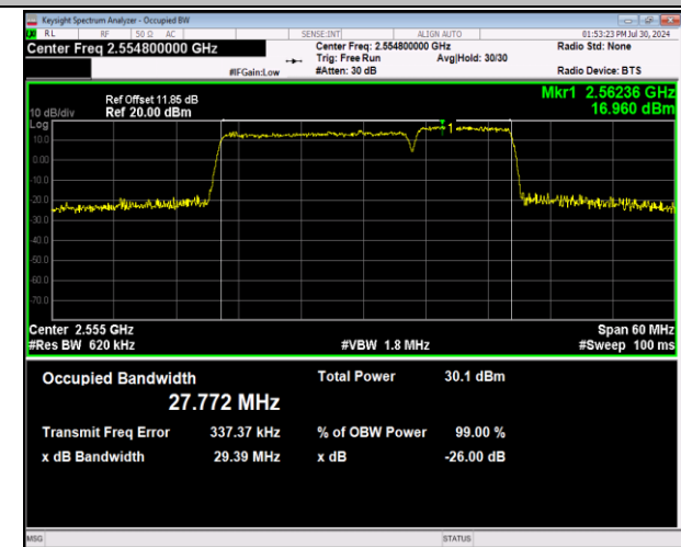
7-7-20MHz-10MHz-64QAM-64QAM-21251-21395-100RB#0-50RB#0-PASS
