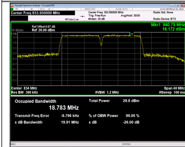
5-5-10MHz-10MHz-64QAM-64QAM-20450-20549-50RB#0-5 -50RB#0-PASS
