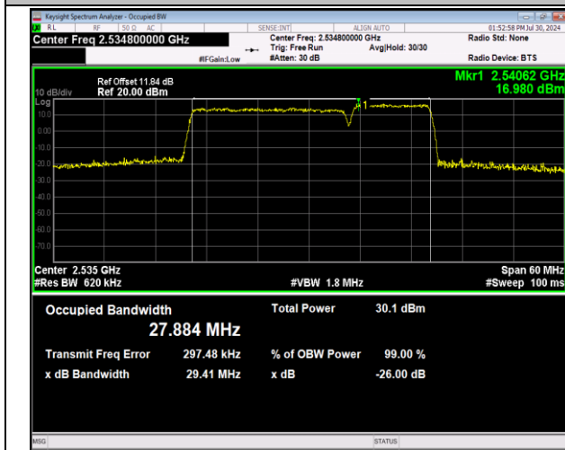
7-7-20MHz-10MHz-64QAM-64QAM-21051-21195-100RB#0-50RB#0-PASS
