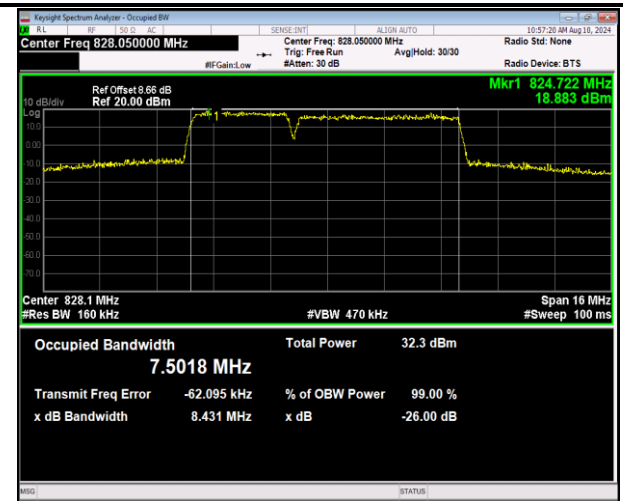
5-5-3MHz-5MHz-16QAM-16QAM-20416-20455-15RB#0-2 5RB#0-PASS
