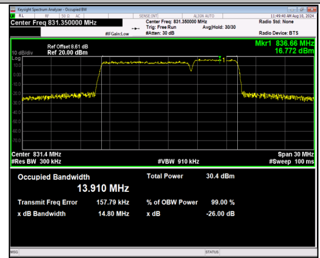
5-5-10MHz-5MHz-QPSK-QPSK-20450-20522-50RB#0-25 RB#0-PASS
