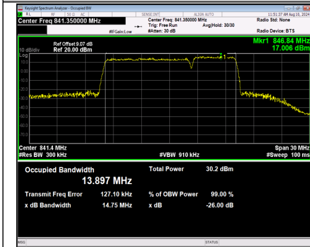
5-5-10MHz-5MHz-16QAM-16QAM-20550-20622-50RB#0-25RB#0-PASS
