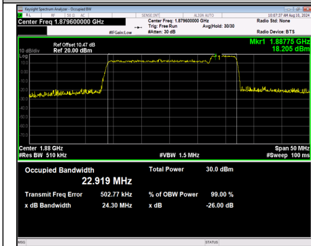
2-2-20MHz-5MHz-16QAM-16QAM-18875-18992-100RB#0-2 -25RB#0-PASS
