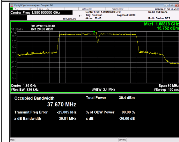
2-2-20MHz-20MHz-16QAM-16QAM-18902-19100-100RB#0-100RB#0-PASS
