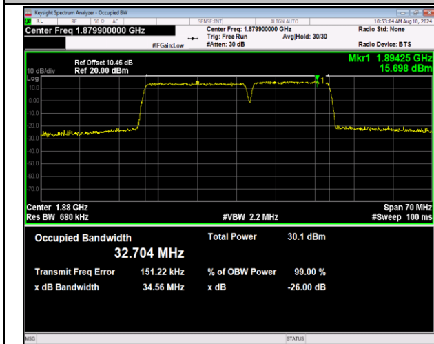
2-2-20MHz-15MHz-16QAM-16QAM-18826-18997-100RB#0-75RB#0-PASS
