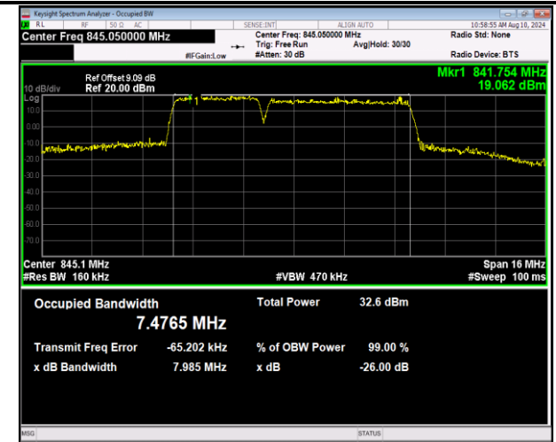
5-5-3MHz-5MHz-16QAM-16QAM-20586-20625-15RB#0-2 5RB#0-PASS
