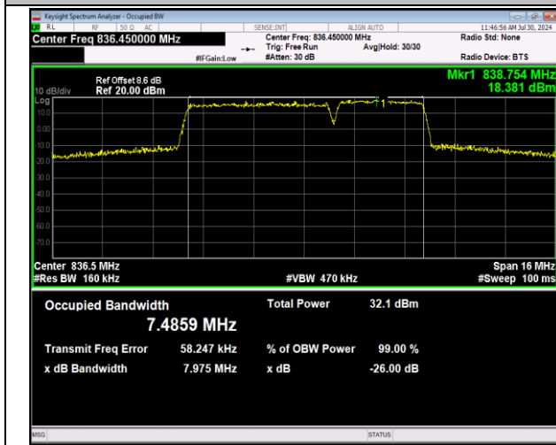
5-5-5MHz-3MHz-64QAM-64QAM-20510-20549-25RB#0-1 5RB#0-PASS
