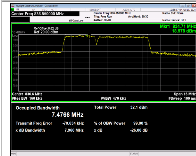
5-5-3MHz-5MHz-16QAM-16QAM-20501-20540-15RB#0-2 5RB#0-PASS
