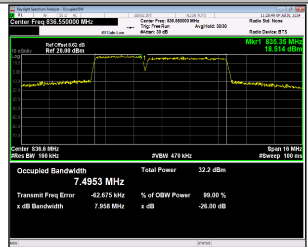
5-5-3MHz-5MHz-64QAM-64QAM-20501-20540-15RB#0-2 5RB#0-PASS
