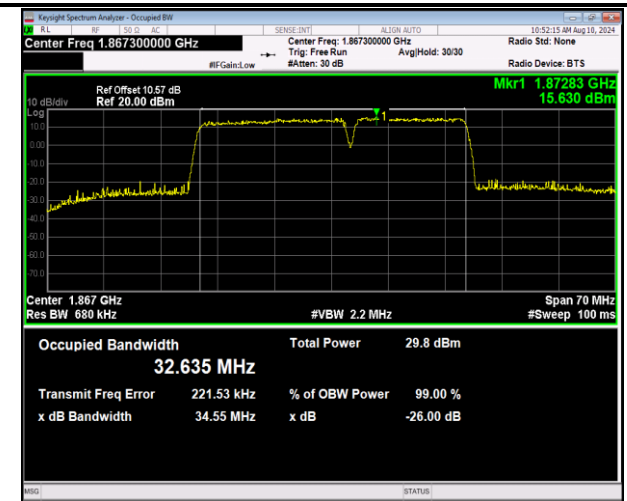
2-2-20MHz-15MHz-16QAM-16QAM-18700-18871-100RB#0-75RB#0-PASS
