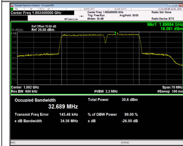
2-2-20MHz-15MHz-64QAM-64QAM-18951-19122-100RB#0-75RB#0-PASS
