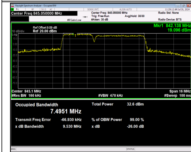
5-5-3MHz-5MHz-64QAM-64QAM-20586-20625-15RB#0-2 5RB#0-PASS
