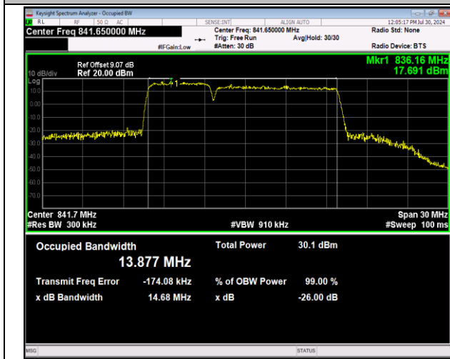
5-5-5MHz-10MHz-64QAM-64QAM-20528-20600-25RB#0-50RB#0-PASS
