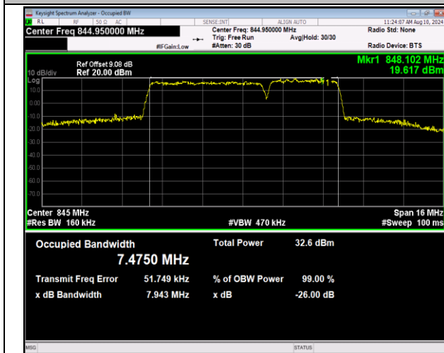
5-5-5MHz-3MHz-16QAM-16QAM-20595-20634-25RB#0-1 5RB#0-PASS
