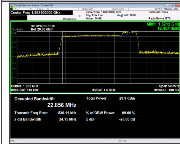
2-2-20MHz-5MHz-64QAM-64QAM-18700-18817-100RB#0-2 -25RB#0-PASS
