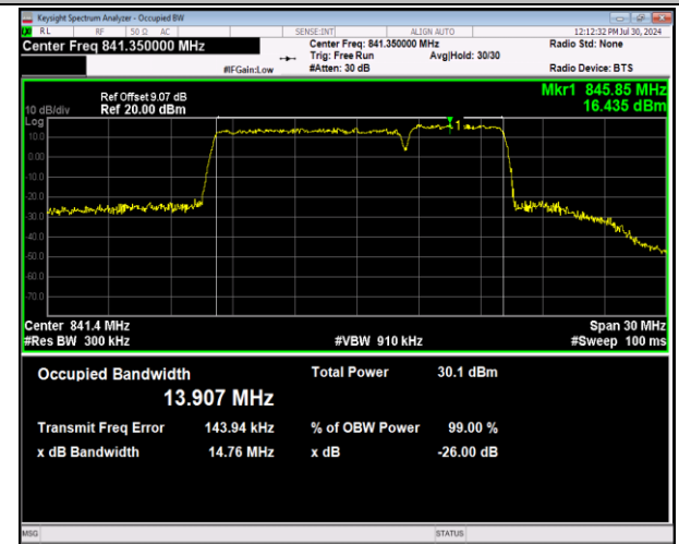
5-5-10MHz-5MHz-64QAM-64QAM-20550-20622-50RB#0-25RB#0-PASS
