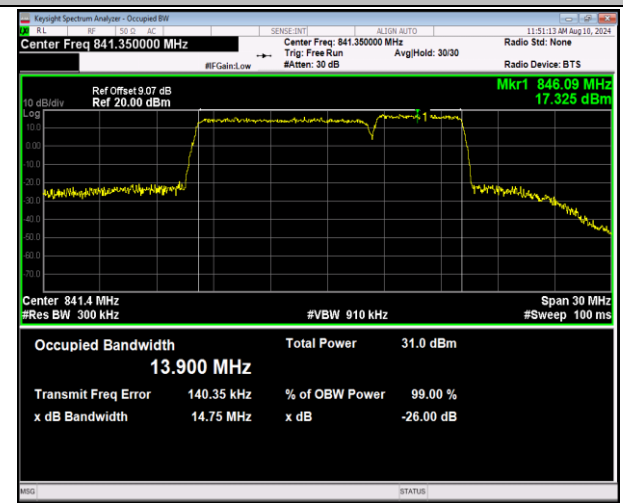
5-5-10MHz-5MHz-QPSK-QPSK-20550-20622-50RB#0-25 RB#0-PASS
