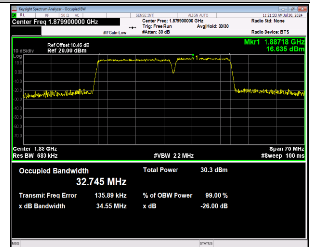
2-2-20MHz-15MHz-64QAM-64QAM-18826-18997-100RB#0-75RB#0-PASS
