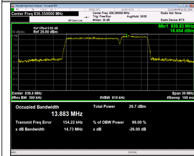
5-5-10MHz-5MHz-64QAM-64QAM-20500-20572-50RB#0-25RB#0-PASS
