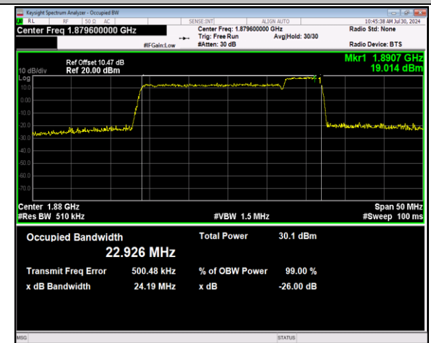
2-2-20MHz-5MHz-64QAM-64QAM-18875-18992-100RB#0-2 -25RB#0-PASS
