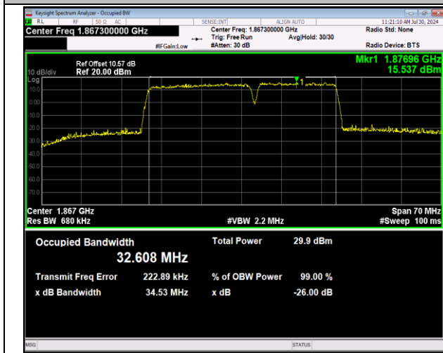
2-2-20MHz-15MHz-64QAM-64QAM-18700-18871-100RB#0-75RB#0-PASS
