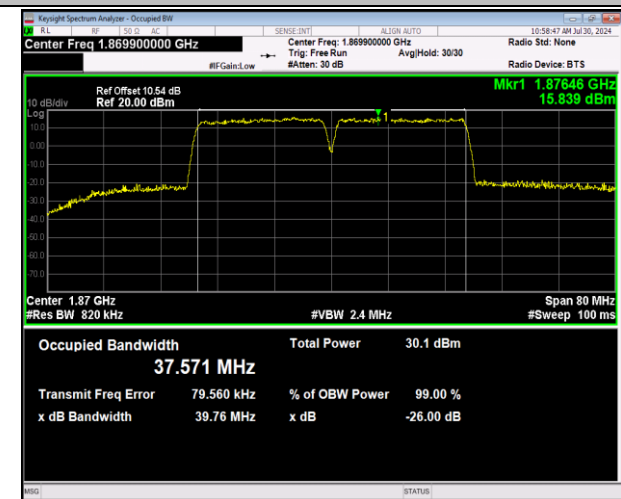
2-2-20MHz-20MHz-64QAM-64QAM-18700-18898-100RB#0-100RB#0-PASS
