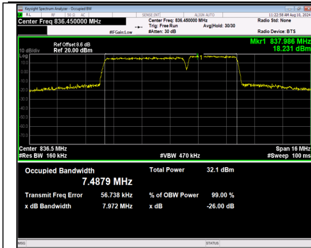
5-5-5MHz-3MHz-QPSK-QPSK-20510-20549-25RB#0-15R B#0-PASS
