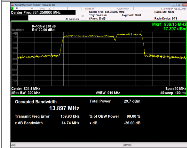
5-5-10MHz-5MHz-16QAM-16QAM-20450-20522-50RB#0-25RB#0-PASS
