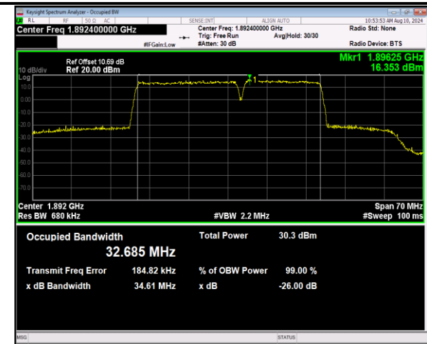
2-2-20MHz-15MHz-16QAM-16QAM-18951-19122-100RB#0-75RB#0-PASS
