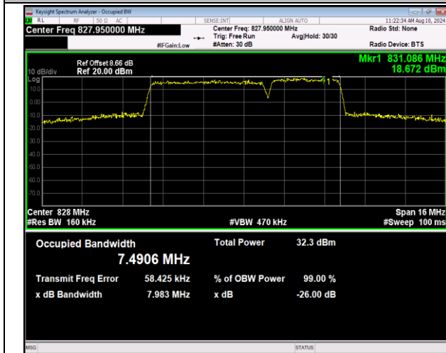
5-5-5MHz-3MHz-16QAM-16QAM-20425-20464-25RB#0-1 5RB#0-PASS
