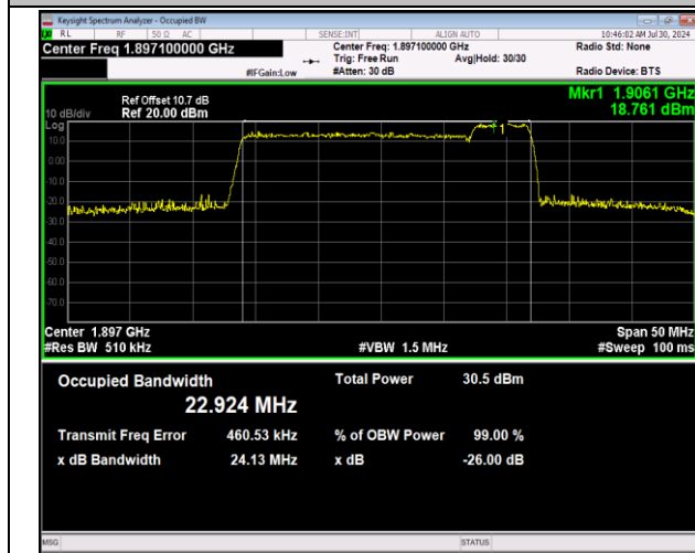
2-2-20MHz-5MHz-64QAM-64QAM-19050-19167-100RB#0 -25RB#0-PASS
