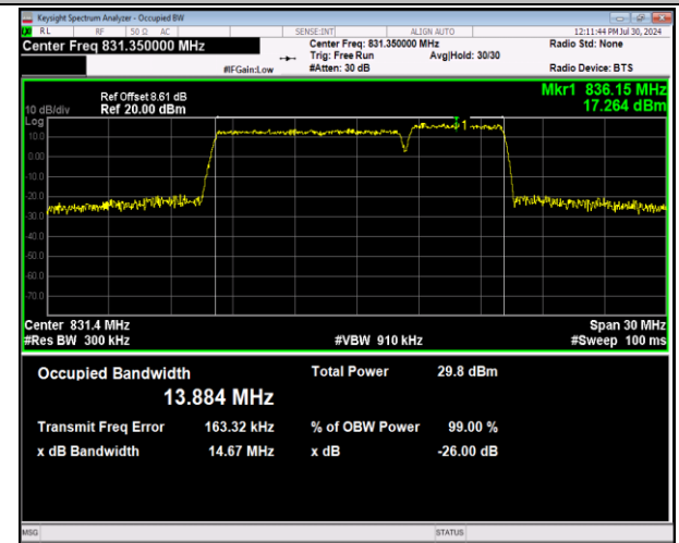
5-5-10MHz-5MHz-64QAM-64QAM-20450-20522-50RB#0-25RB#0-PASS
