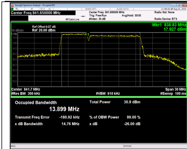
5-5-5MHz-10MHz-QPSK-QPSK-20528-20600-25RB#0-50 RB#0-PASS
