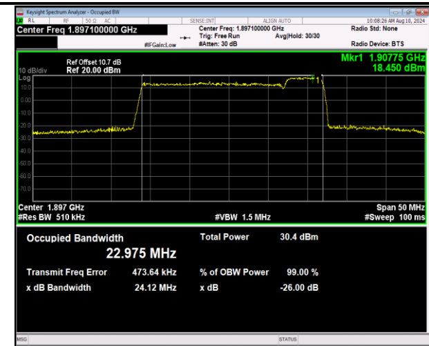
2-2-20MHz-5MHz-16QAM-16QAM-19050-19167-100RB#0 -25RB#0-PASS
