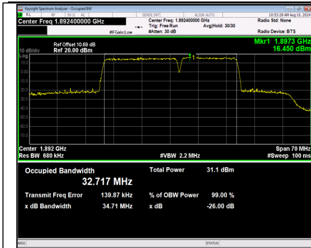
2-2-20MHz-15MHz-QPSK-QPSK-18951-19122-100RB#0-75RB#0-PASS
