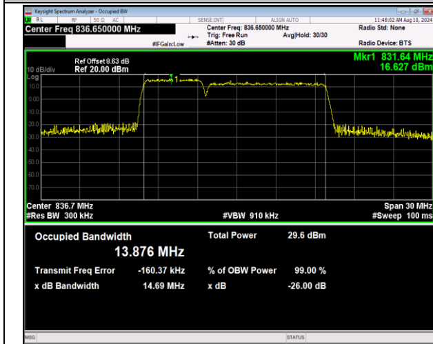
5-5-5MHz-10MHz-16QAM-16QAM-20478-20550-25RB#0-50RB#0-PASS
