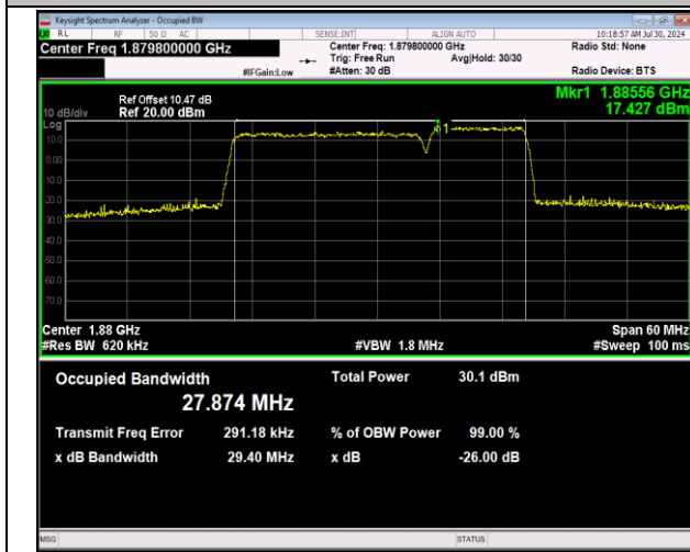
2-2-20MHz-10MHz-64QAM-64QAM-18851-18995-100RB#0-50RB#0-PASS
