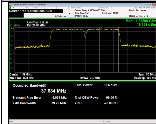
2-2-20MHz-20MHz-64QAM-64QAM-18801-18999-100RB#0-100RB#0-PASS
