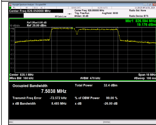
5-5-3MHz-5MHz-64QAM-64QAM-20416-20455-15RB#0-2 5RB#0-PASS
