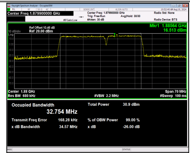
2-2-20MHz-15MHz-QPSK-QPSK-18826-18997-100RB#0-75RB#0-PASS
