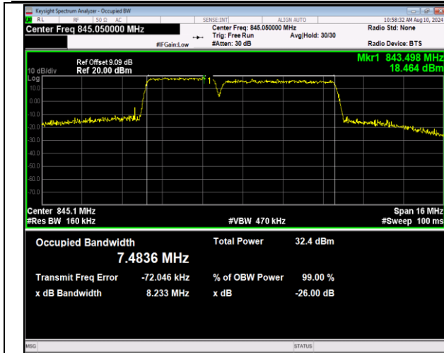
5-5-3MHz-5MHz-QPSK-QPSK-20586-20625-15RB#0-25R B#0-PASS
