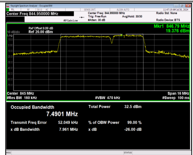
5-5-5MHz-3MHz-64QAM-64QAM-20595-20634-25RB#0-1 5RB#0-PASS
