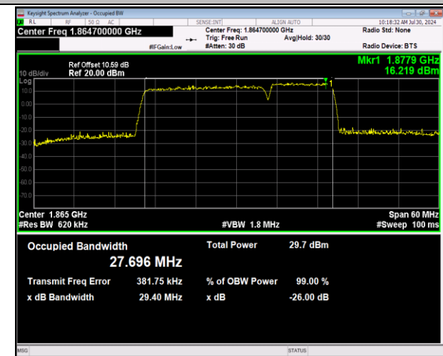
2-2-20MHz-10MHz-64QAM-64QAM-18700-18844-100RB# 0-50RB#0-PASS
