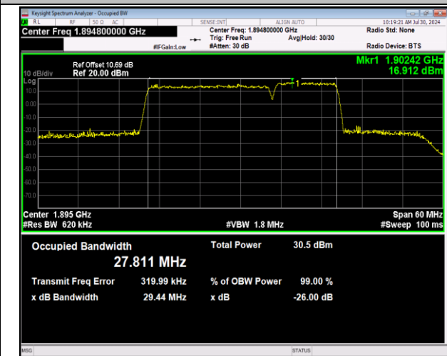
2-2-20MHz-10MHz-64QAM-64QAM-19001-19145-100RB#0-50RB#0-PASS
