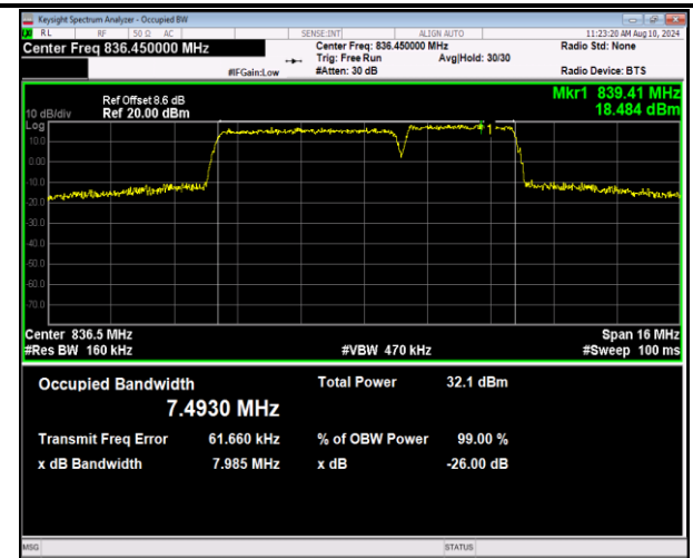
5-5-5MHz-3MHz-16QAM-16QAM-20510-20549-25RB#0-1 5RB#0-PASS
