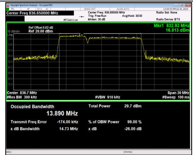
5-5-5MHz-10MHz-64QAM-64QAM-20478-20550-25RB#0-50RB#0-PASS
