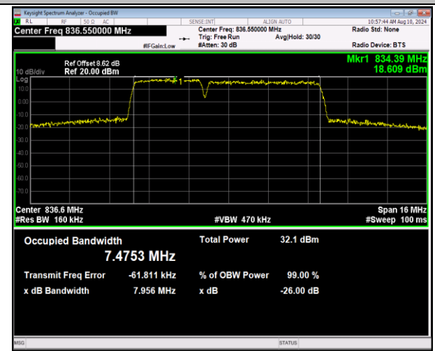
5-5-3MHz-5MHz-QPSK-QPSK-20501-20540-15RB#0-25R B#0-PASS
