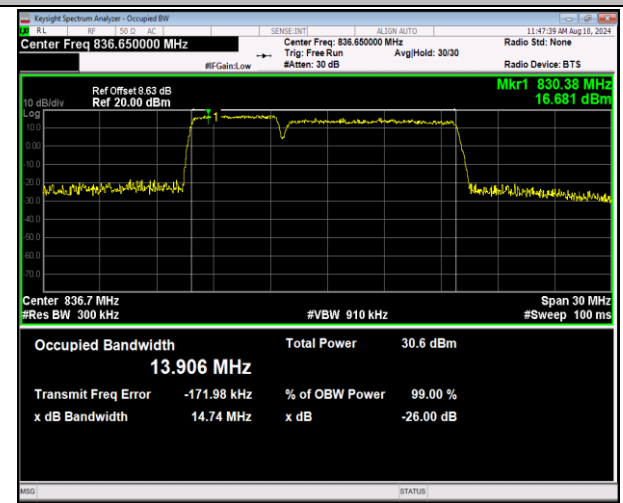
5-5-5MHz-10MHz-QPSK-QPSK-20478-20550-25RB#0-50 RB#0-PASS
