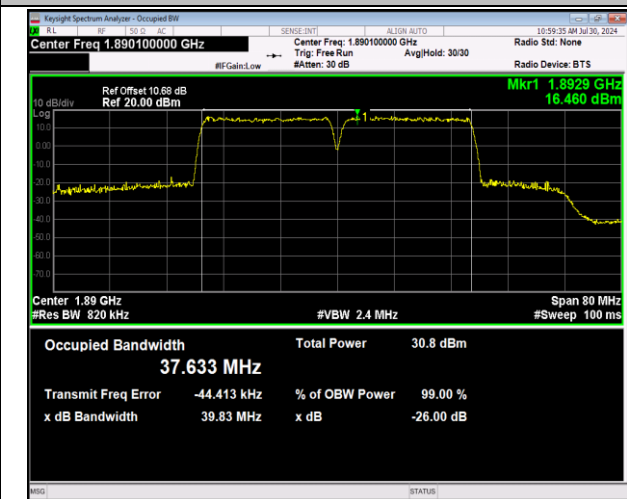
2-2-20MHz-20MHz-64QAM-64QAM-18902-19100-100RB#0-100RB#0-PASS
