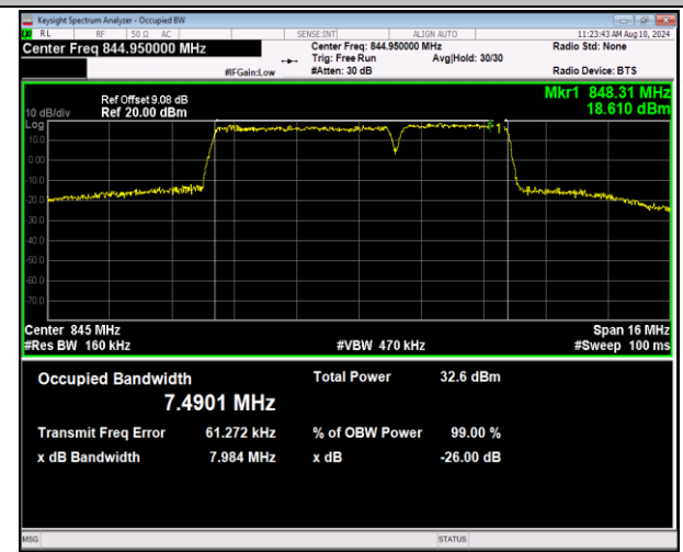
5-5-5MHz-3MHz-QPSK-QPSK-20595-20634-25RB#0-15R B#0-PASS
