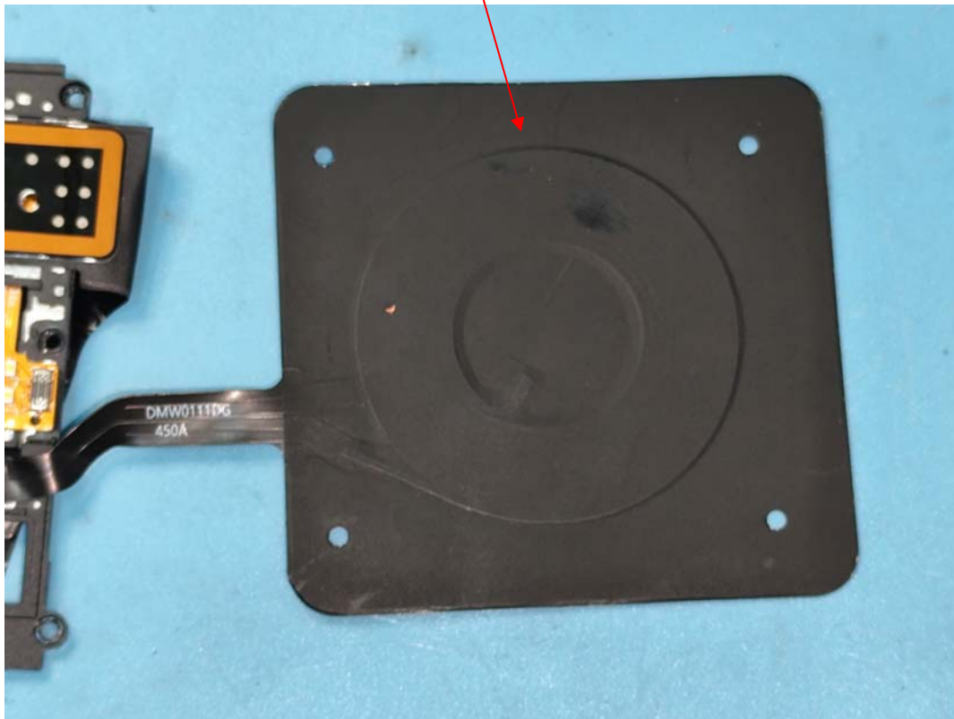
WPT Antenna
