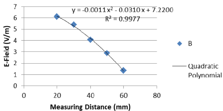
Position B E-Field
