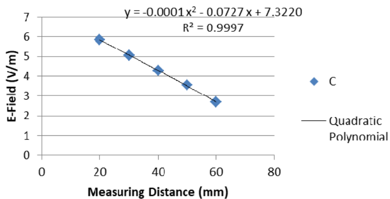
Position C E-Field
