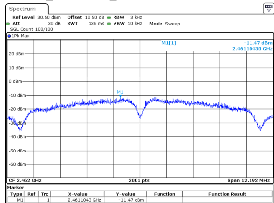
802.11b_2462MHz_Main ANT -11.47dBm/3kHz
