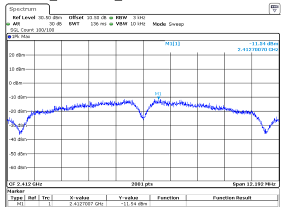
802.11b_2412MHz_Aux ANT -11.54dBm/3kHz
