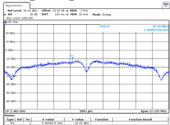
802.11b_2462MHz_Aux ANT -10.43dBm/3kHz
