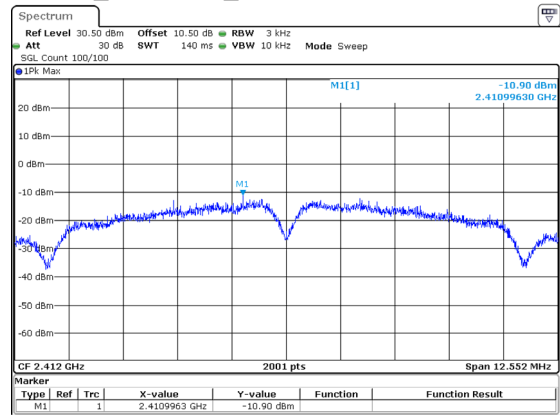
802.11b_2412MHz_Main ANT -10.90dBm/3kHz
