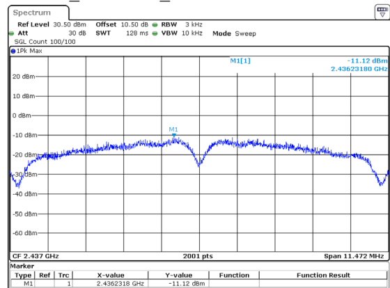
802.11b_2437MHz_Aux ANT -11.12dBm/3kHz
