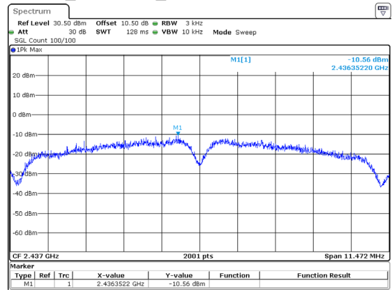
802.11b_2437MHz_Main ANT -10.56dBm/3kHz
