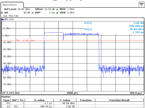
2DH1_Hopping 0.388ms
