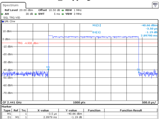
2DH5_Hopping 2.898ms
