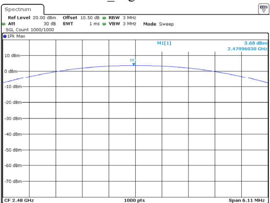
3DH1_High 3.68dBm
