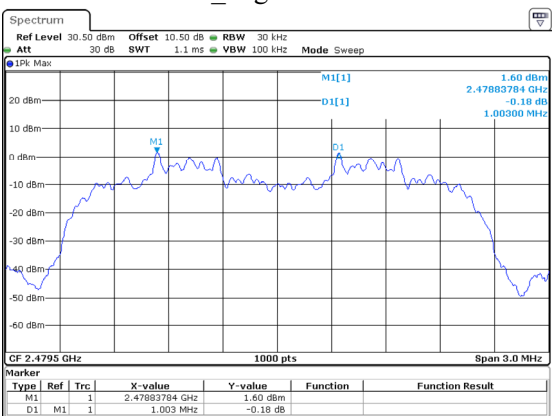
2DH1_High 1.003MHz
