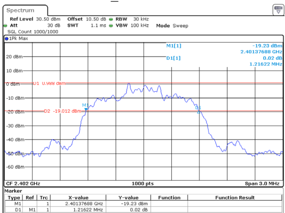
2DH1_Low 1.216MHz
