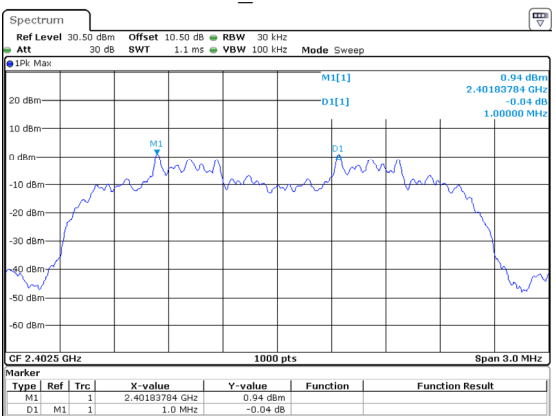
2DH1_Low 1MHz
