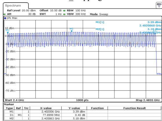
DH1_Hopping 79
