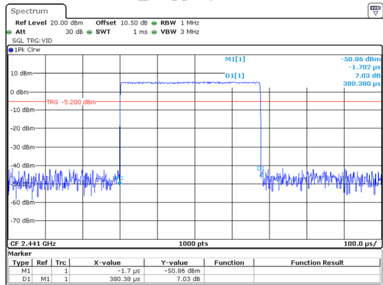
DH1_Hopping 0.380ms
