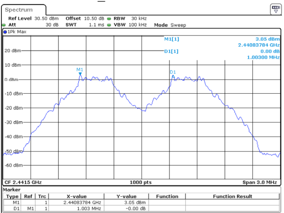
DH1_Middle 1.003MHz
