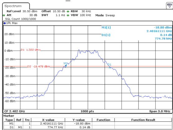
DH1_Low 0.775MHz
