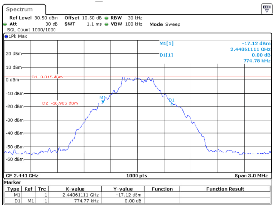
DH1_Middle 0.775MHz
