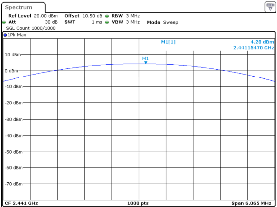
2DH1_Middle 4.28dBm
