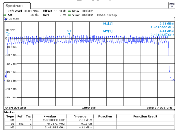
3DH1_Hopping 79
