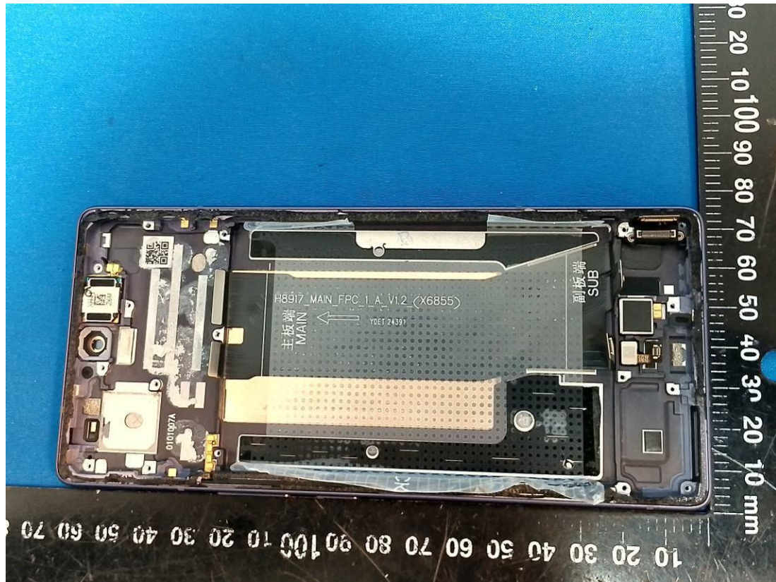
Bluetooth&2.4G Wifi(Chain 1)&5G Wifi Antenna(ANT 13)
