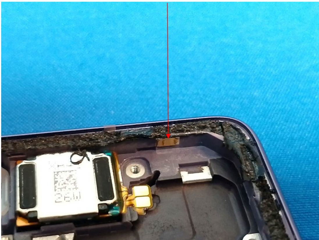
WWAN Antenna(ANT 3)
