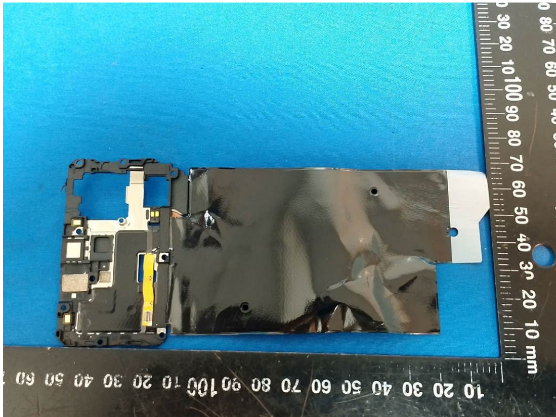
Wireless Charging Antenna
