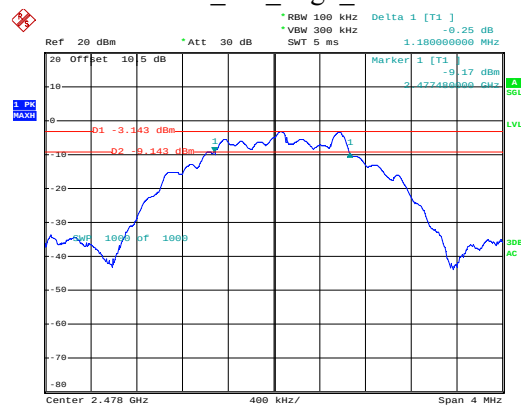
BLE_2M_High_Channel
