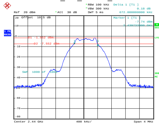
BLE_1M_Middle_Channel
