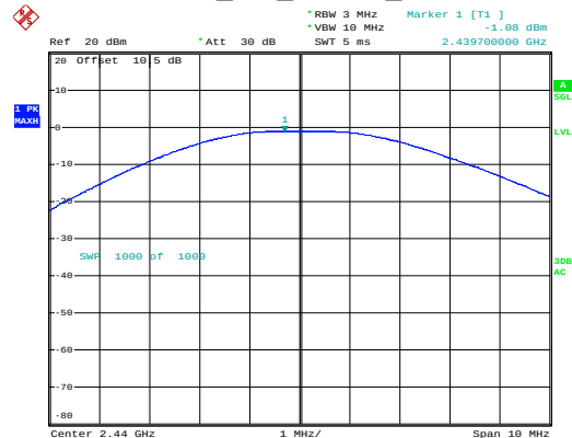
BLE_2M_Middle_Channel
