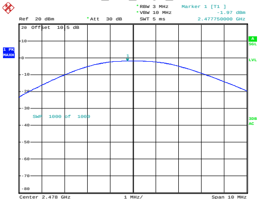
BLE_2M_High_Channel
