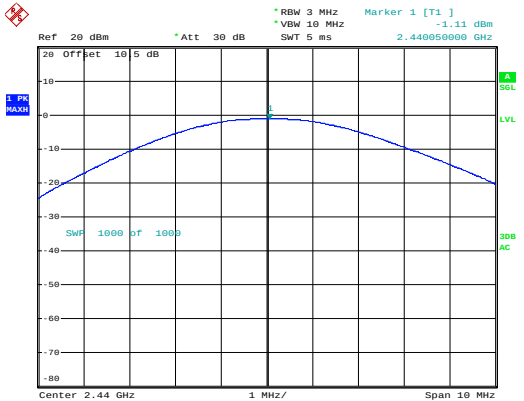
BLE_1M_Middle_Channel
