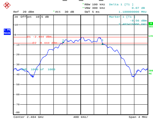
BLE_2M_Low_Channel
