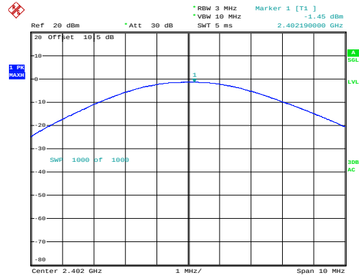
BLE_1M_Low_Channel
