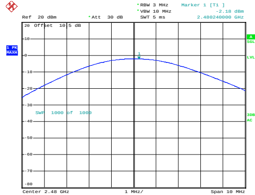
BLE_1M_High_Channel
