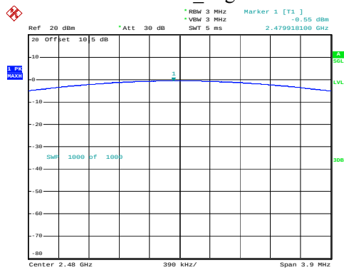
DH1_High
