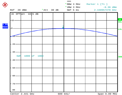
2DH1_Middle
