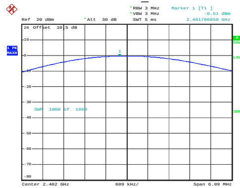
2DH1_Low
