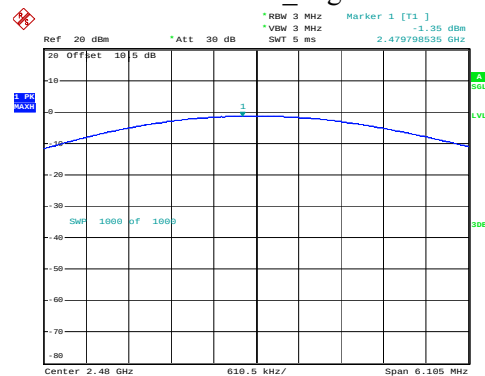
2DH1_High
