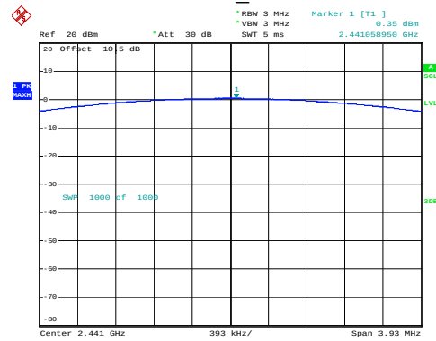
DH1_Middle
