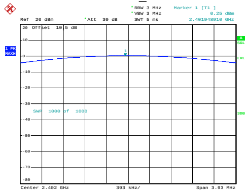
DH1_Low
