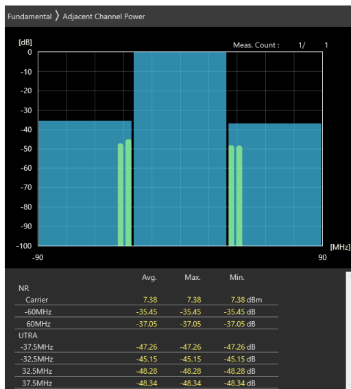
60MHz_30kHz_3580MHz_CP-OFDM 16 QAM_RB1@0 -35.45 dB,-37.05 dB
