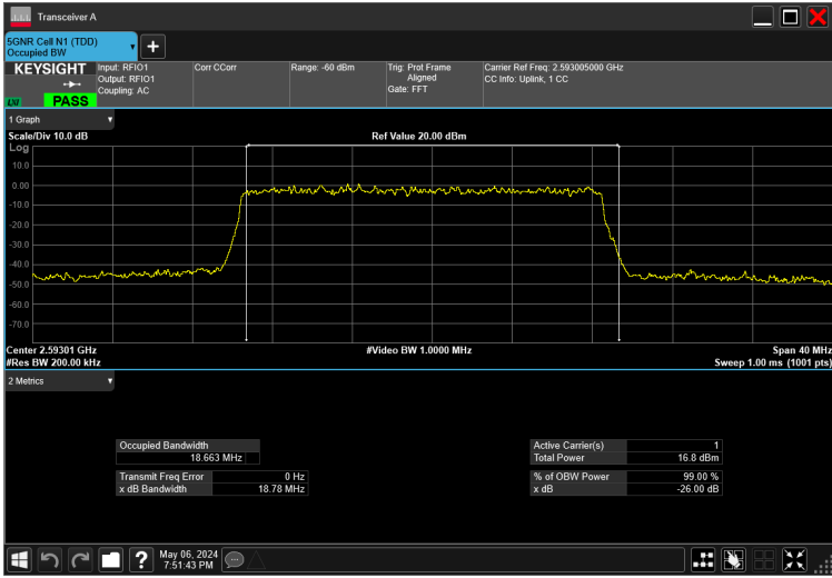
20MHz_15kHz_2593.005MHz_DFT-s-OFDM 256 QAM_RB100@0 18.663 MHz
