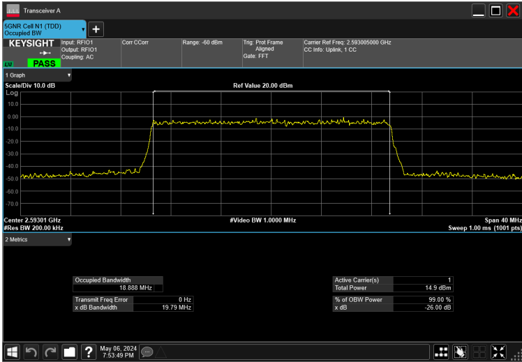
20MHz_15kHz_2593.005MHz_CP-OFDM 256 QAM_RB106@0 18.888 MHz
