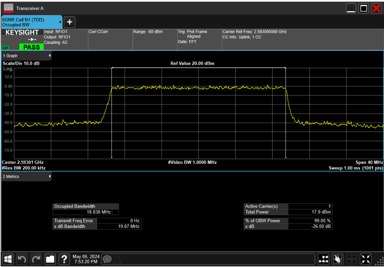
20MHz_15kHz_2593.005MHz_CP-OFDM 64 QAM_RB106@0 18.838 MHz
