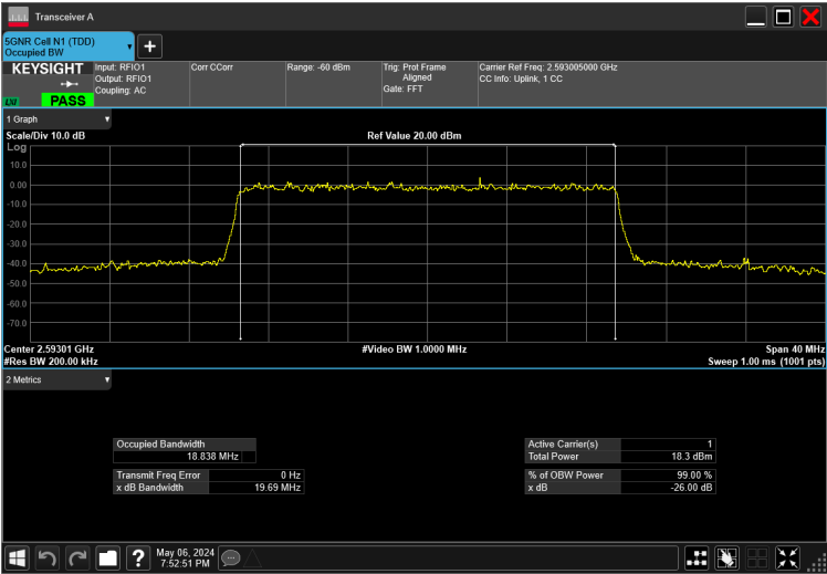
20MHz_15kHz_2593.005MHz_CP-OFDM 16 QAM_RB106@0 18.838 MHz
