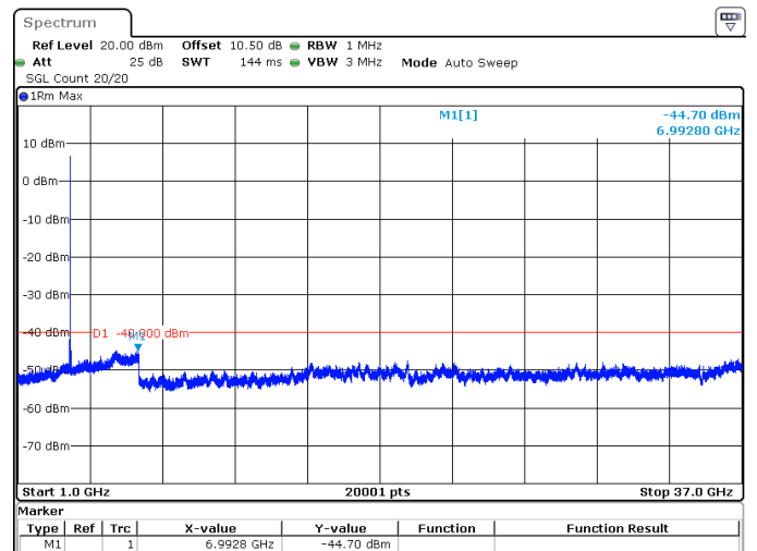
60MHz_30kHz_3580MHz_DFT-s-OFDM QPSK_RB1@161 -44.70 dBm
