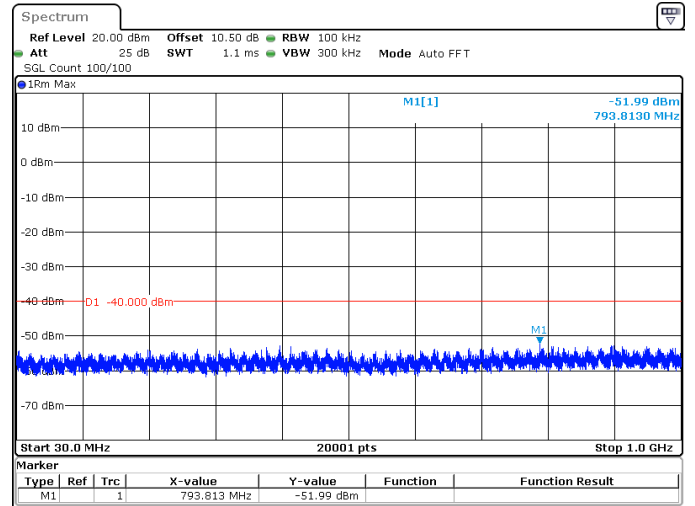
40MHz_30kHz_3570MHz_DFT-s-OFDM QPSK_RB1@0 -51.99 dBm
