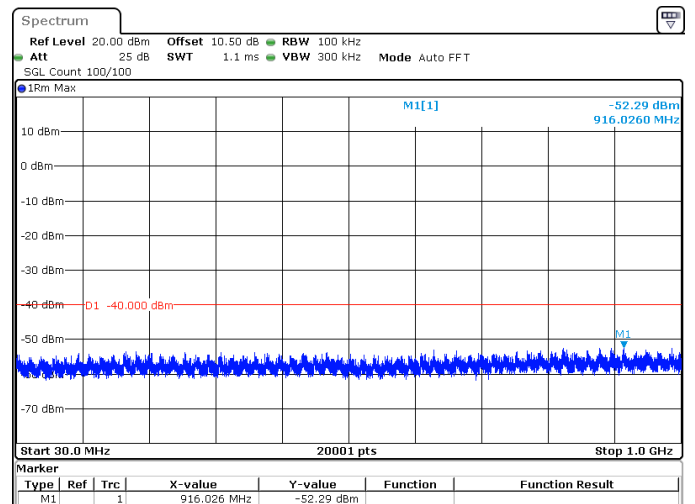
40MHz_30kHz_3570MHz_DFT-s-OFDM QPSK_RB100@0 -52.29 dBm
