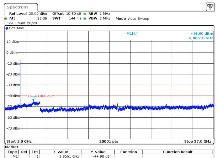
60MHz_30kHz_3580MHz_DFT-s-OFDM QPSK_RB162@0 -44.90 dBm
