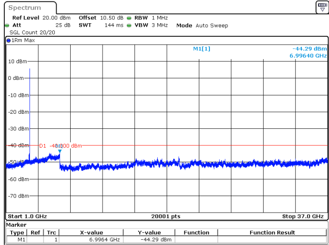
90MHz_30kHz_3595MHz_DFT-s-OFDM QPSK_RB1@244 -44.29 dBm
