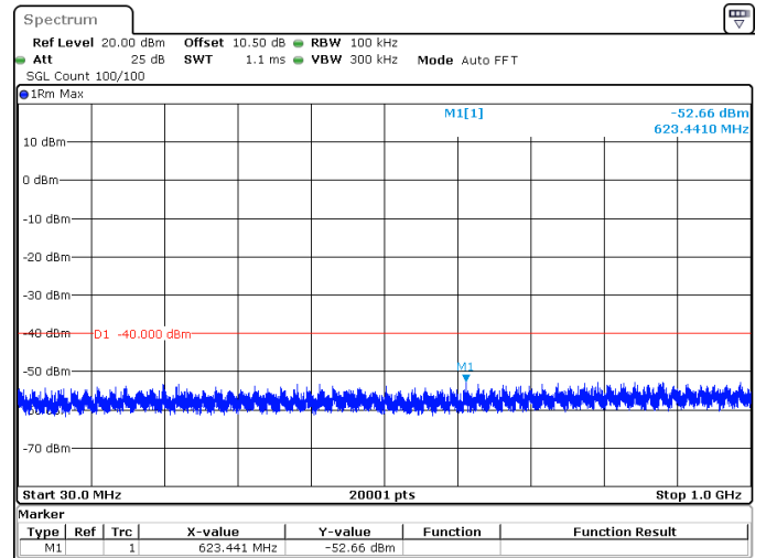
40MHz_30kHz_3570MHz_DFT-s-OFDM QPSK_RB1@105 -52.66 dBm
