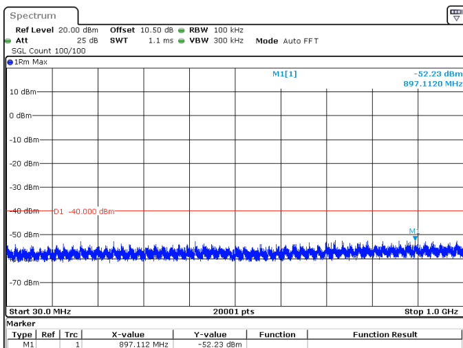
30MHz_30kHz_3565MHz_DFT-s-OFDM QPSK_RB1@77 -52.23 dBm
