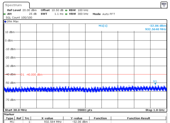
25MHz_15kHz_3562.5MHz_DFT-s-OFDM QPSK_RB128@0 -52.06 dBm
