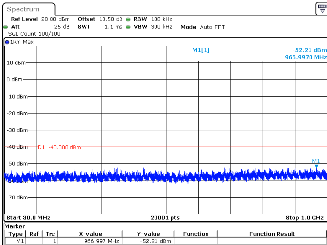
30MHz_15kHz_3565MHz_DFT-s-OFDM QPSK_RB160@0 -52.21 dBm
