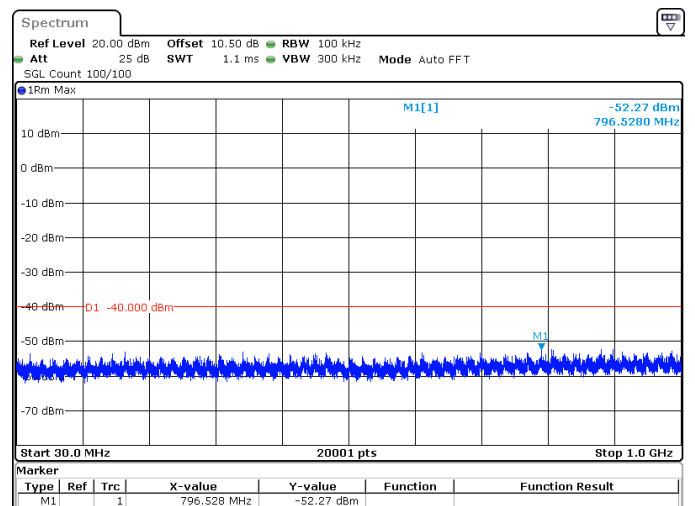
15MHz_15kHz_3557.5MHz_DFT-s-OFDM QPSK_RB75@0 -52.27 dBm
