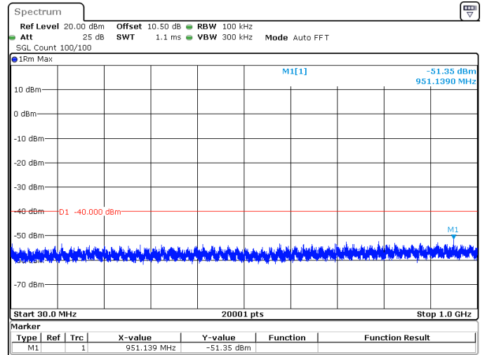
25MHz_30kHz_3562.5MHz_DFT-s-OFDM QPSK_RB1@0 -51.35 dBm
