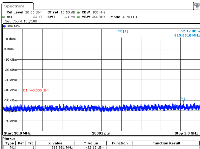
15MHz_30kHz_3692.5MHz_DFT-s-OFDM QPSK_RB1@37 -52.12 dBm
