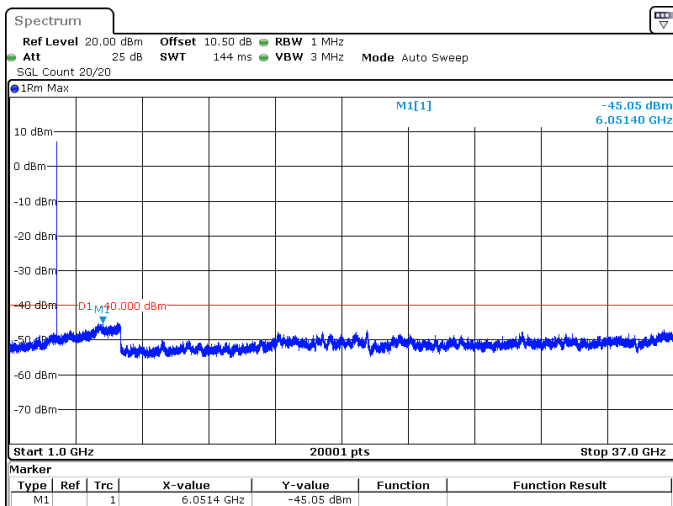
15MHz_15kHz_3557.5MHz_DFT-s-OFDM QPSK_RB1@0 -45.05 dBm
