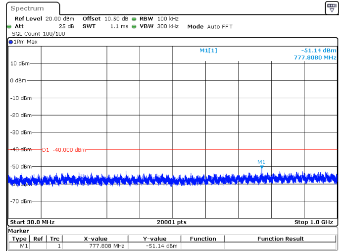
25MHz_15kHz_3562.5MHz_DFT-s-OFDM QPSK_RB1@0 -51.14 dBm
