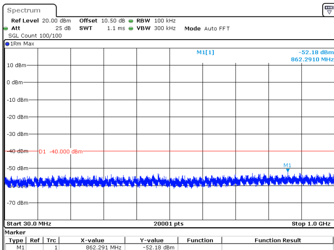
15MHz_30kHz_3557.5MHz_DFT-s-OFDM QPSK_RB1@37 -52.18 dBm
