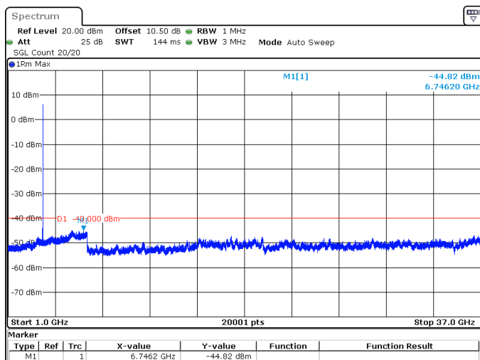
25MHz_15kHz_3625MHz_DFT-s-OFDM QPSK_RB1@132 -44.82 dBm
