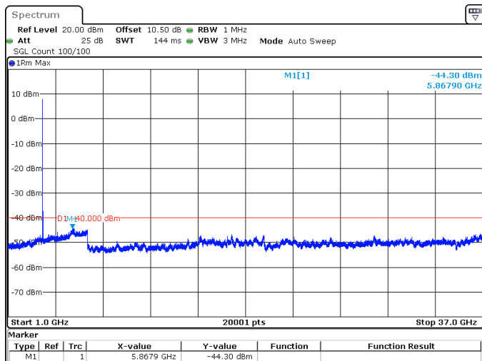
25MHz_15kHz_3625MHz_DFT-s-OFDM QPSK_RB1@0 -44.30 dBm
