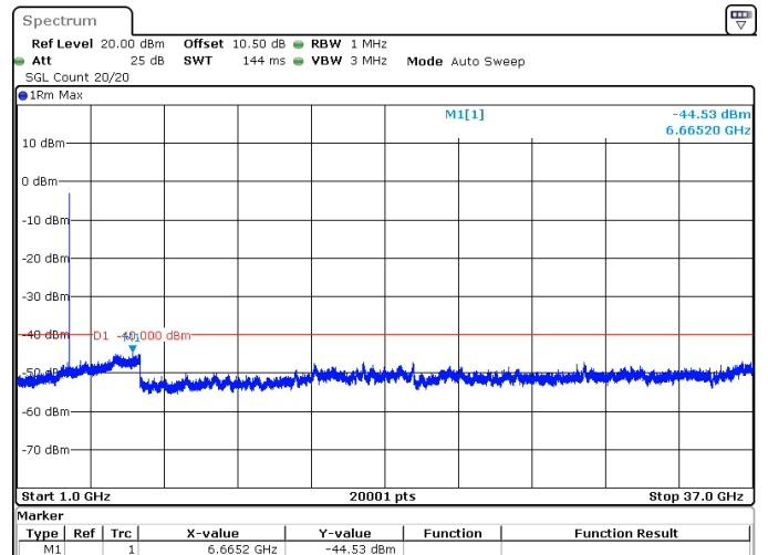
25MHz_30kHz_3562.5MHz_DFT-s-OFDM QPSK_RB64@0 -44.53 dBm
