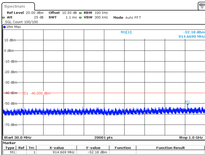
30MHz_30kHz_3565MHz_DFT-s-OFDM QPSK_RB1@0 -52.18 dBm
