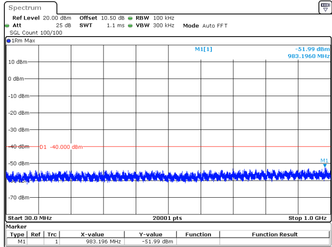
90MHz_30kHz_3595MHz_DFT-s-OFDM QPSK_RB1@244 -51.99 dBm
