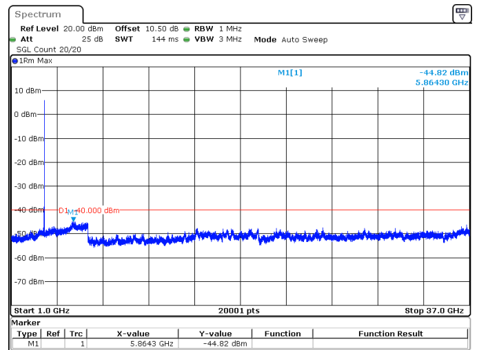
30MHz_30kHz_3565MHz_DFT-s-OFDM QPSK_RB1@77 -44.82 dBm
