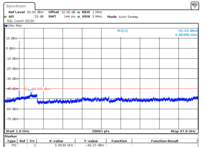
25MHz_15kHz_3687.5MHz_DFT-s-OFDM QPSK_RB1@132 -45.23 dBm
