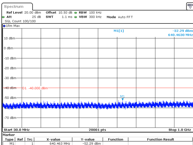
30MHz_15kHz_3625MHz_DFT-s-OFDM QPSK_RB1@159 -52.29 dBm
