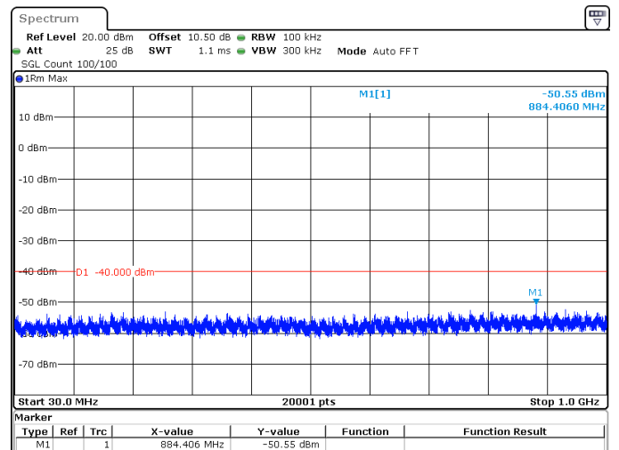
25MHz_15kHz_3625MHz_DFT-s-OFDM QPSK_RB1@132 -50.55 dBm
