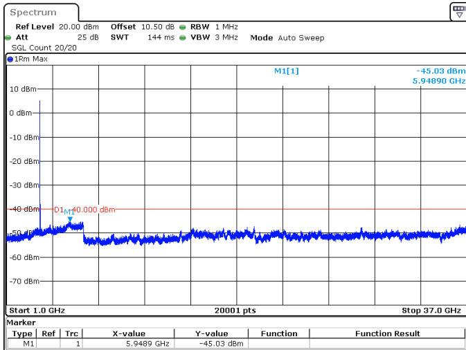
25MHz_30kHz_3625MHz_DFT-s-OFDM QPSK_RB1@0 -45.03 dBm
