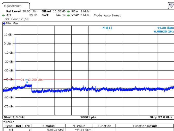
15MHz_15kHz_3692.5MHz_DFT-s-OFDM QPSK_RB1@78 -44.38 dBm
