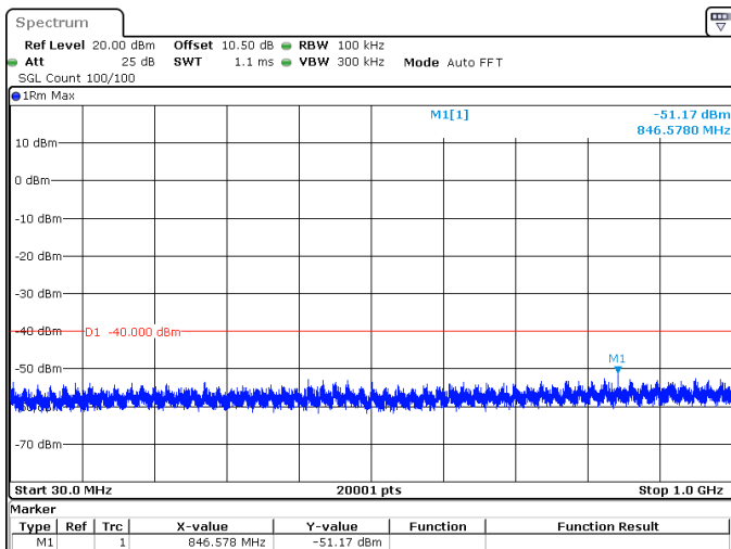
30MHz_15kHz_3625MHz_DFT-s-OFDM QPSK_RB1@0 -51.17 dBm
