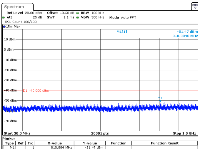
25MHz_15kHz_3687.5MHz_DFT-s-OFDM QPSK_RB1@132 -51.47 dBm
