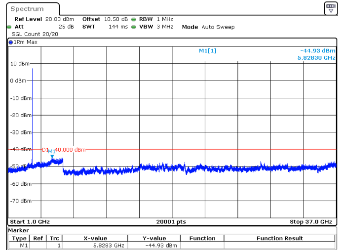
15MHz_15kHz_3625MHz_DFT-s-OFDM QPSK_RB1@78 -44.93 dBm
