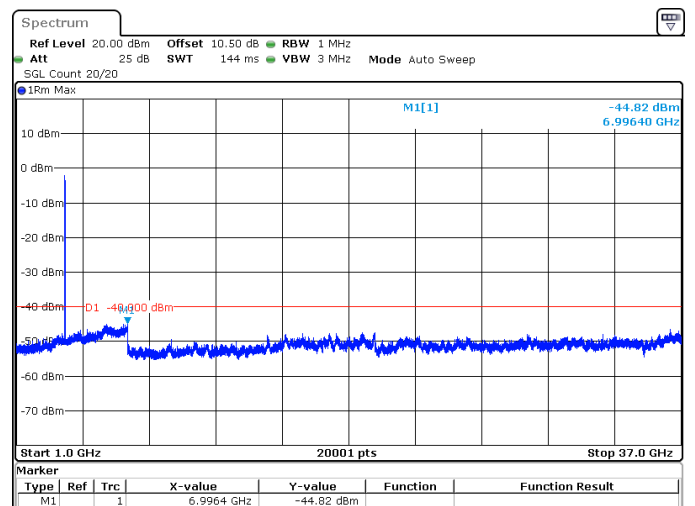
25MHz_15kHz_3625MHz_DFT-s-OFDM QPSK_RB128@0 -44.82 dBm
