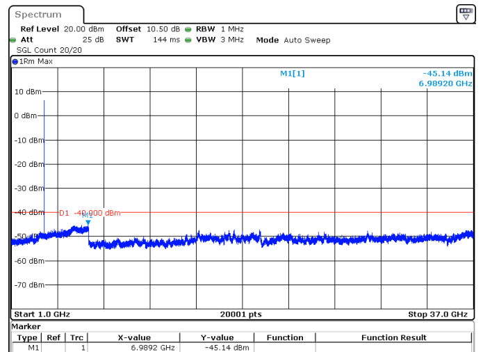
15MHz_15kHz_3557.5MHz_DFT-s-OFDM QPSK_RB1@78 -45.14 dBm
