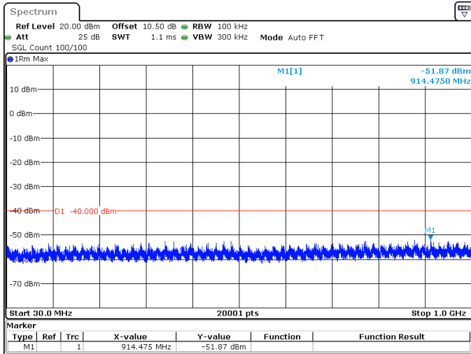
15MHz_30kHz_3557.5MHz_DFT-s-OFDM QPSK_RB36@0 -51.87 dBm
