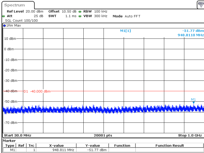
25MHz_30kHz_3687.5MHz_DFT-s-OFDM QPSK_RB64@0 -51.77 dBm
