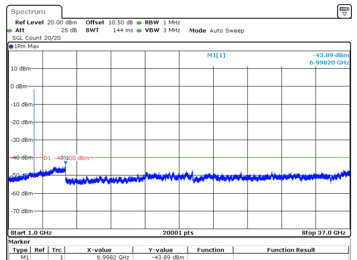
25MHz_15kHz_3687.5MHz_DFT-s-OFDM QPSK_RB128@0 -43.89 dBm
