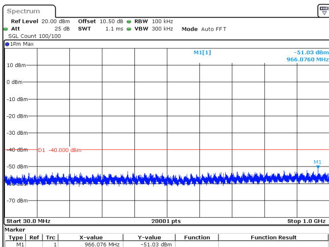
15MHz_15kHz_3557.5MHz_DFT-s-OFDM QPSK_RB1@78 -51.03 dBm
