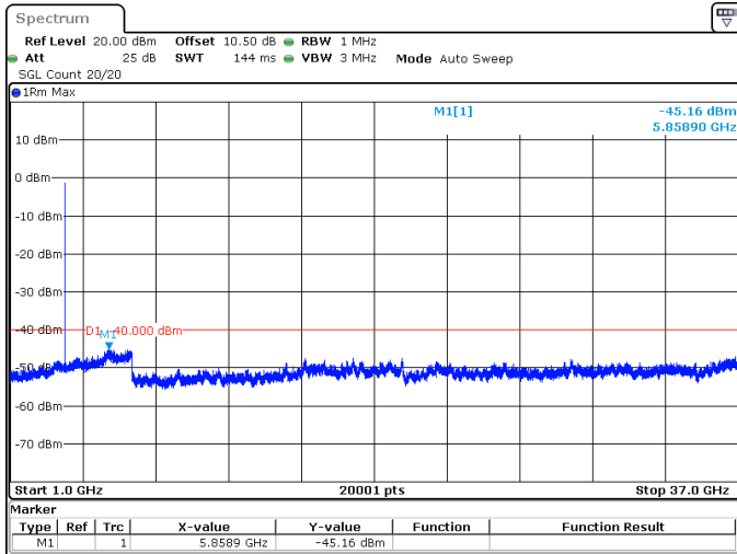
15MHz_15kHz_3692.5MHz_DFT-s-OFDM QPSK_RB75@0 -45.16 dBm
