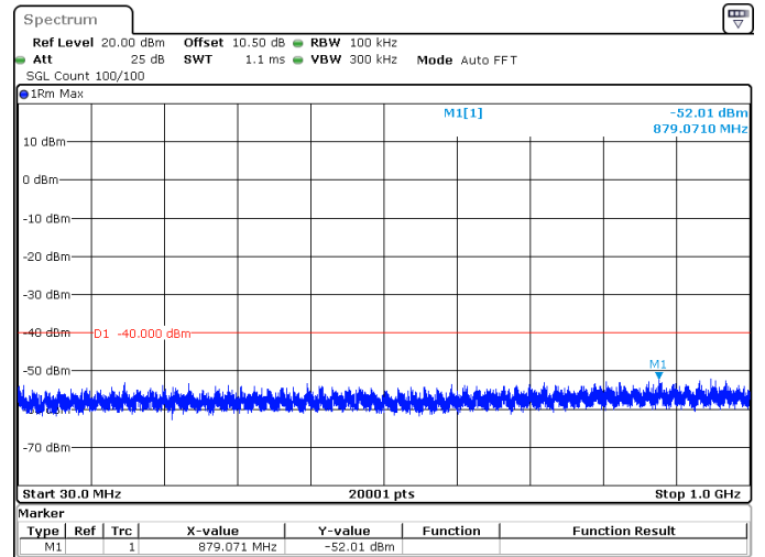
25MHz_15kHz_3562.5MHz_DFT-s-OFDM QPSK_RB1@132 -52.01 dBm
