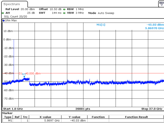
15MHz_15kHz_3557.5MHz_DFT-s-OFDM QPSK_RB75@0 -45.03 dBm
