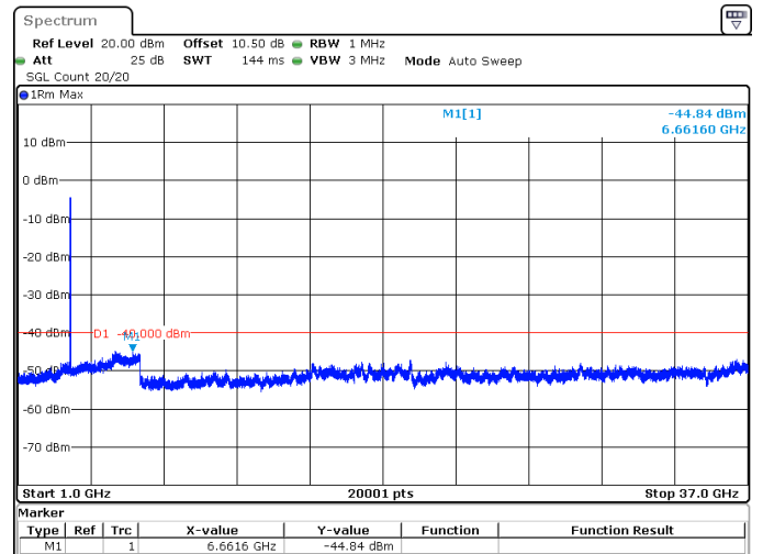
30MHz_15kHz_3565MHz_DFT-s-OFDM QPSK_RB160@0 -44.84 dBm
