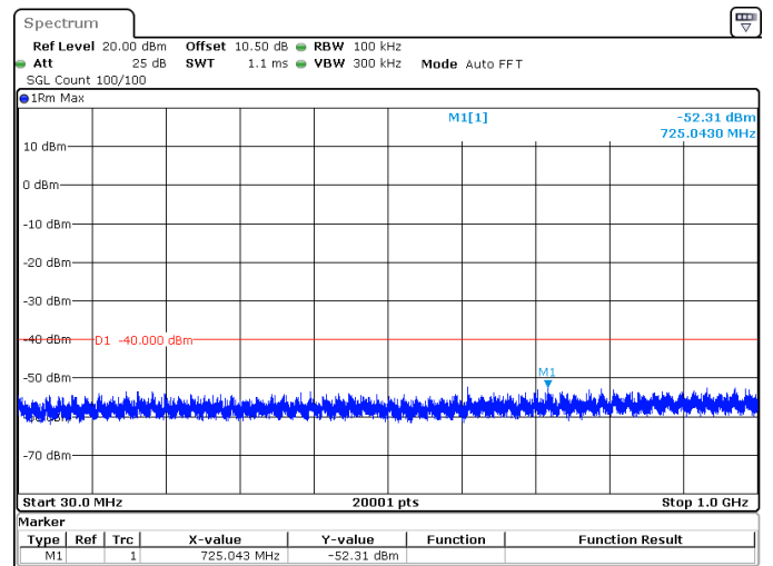
15MHz_15kHz_3692.5MHz_DFT-s-OFDM QPSK_RB1@78 -52.31 dBm
