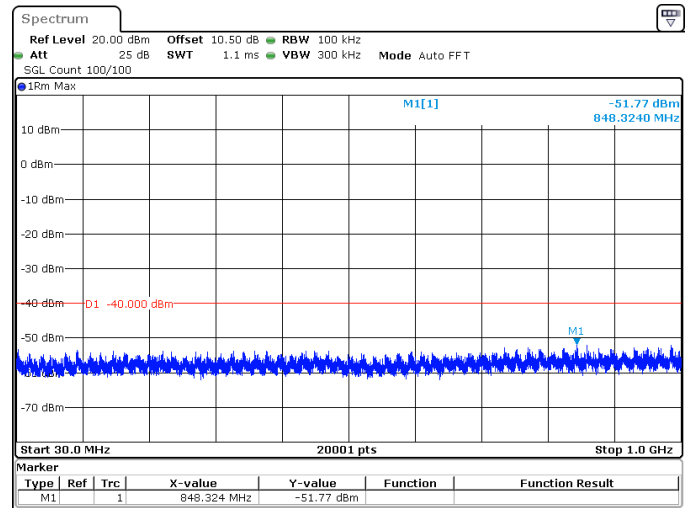
25MHz_30kHz_3687.5MHz_DFT-s-OFDM QPSK_RB1@0 -51.77 dBm
