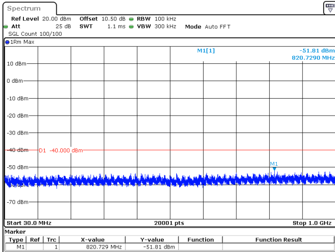
25MHz_15kHz_3687.5MHz_DFT-s-OFDM QPSK_RB128@0 -51.81 dBm
