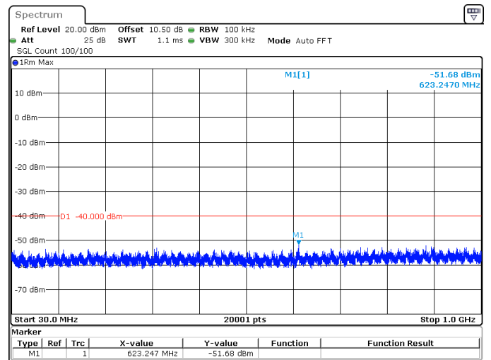
25MHz_30kHz_3687.5MHz_DFT-s-OFDM QPSK_RB1@64 -51.68 dBm
