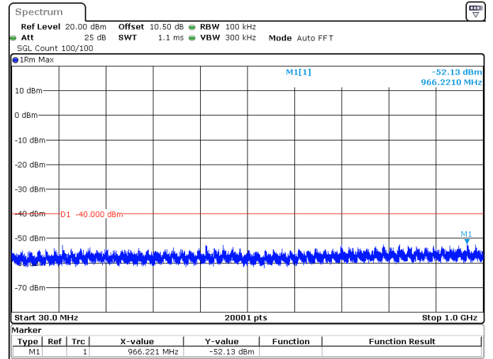
30MHz_15kHz_3565MHz_DFT-s-OFDM QPSK_RB1@0 -52.13 dBm
