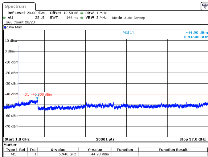
15MHz_15kHz_3692.5MHz_DFT-s-OFDM QPSK_RB1@0 -44.90 dBm
