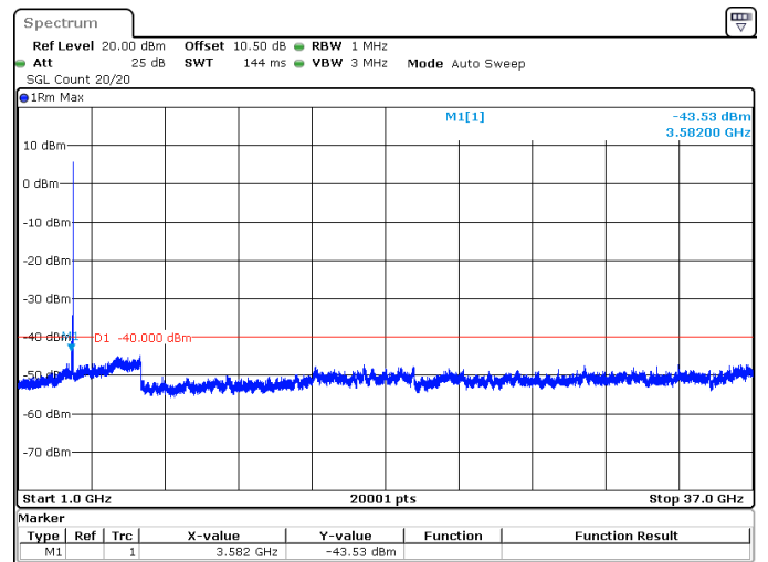
100MHz_30kHz_3625MHz_DFT-s-OFDM QPSK_RB1@272 -43.53 dBm
