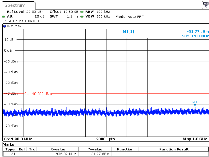
25MHz_30kHz_3562.5MHz_DFT-s-OFDM QPSK_RB64@0 -51.77 dBm
