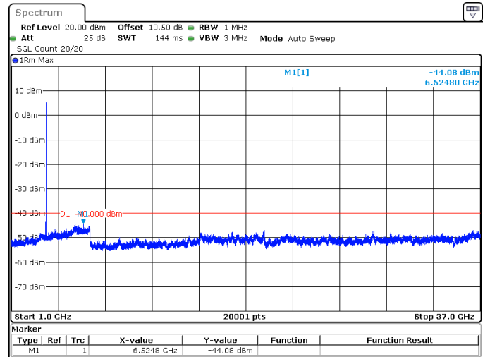
15MHz_30kHz_3625MHz_DFT-s-OFDM QPSK_RB1@37 -44.08 dBm
