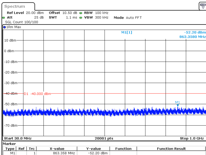
25MHz_15kHz_3687.5MHz_DFT-s-OFDM QPSK_RB1@0 -52.20 dBm
