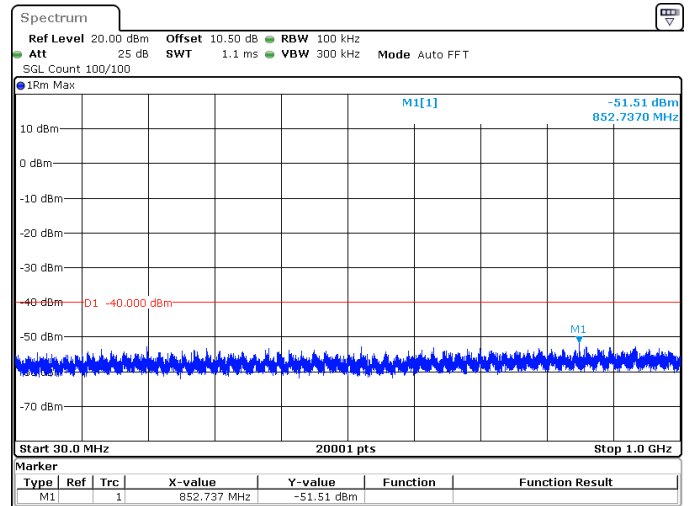
10MHz_15kHz_3625MHz_DFT-s-OFDM QPSK_RB1@51 -51.51 dBm
