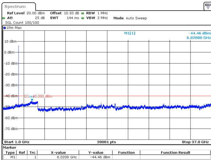
25MHz_30kHz_3687.5MHz_DFT-s-OFDM QPSK_RB1@0 -44.46 dBm
