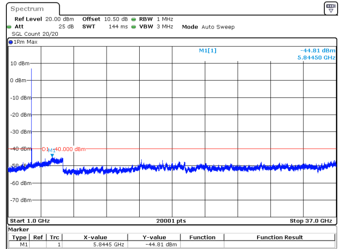
15MHz_30kHz_3557.5MHz_DFT-s-OFDM QPSK_RB1@37 -44.81 dBm
