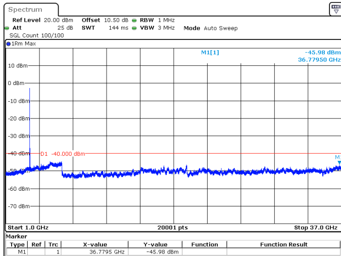
25MHz_15kHz_3562.5MHz_DFT-s-OFDM QPSK_RB128@0 -45.98 dBm
