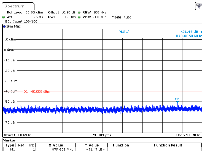
15MHz_30kHz_3625MHz_DFT-s-OFDM QPSK_RB1@37 -51.47 dBm
