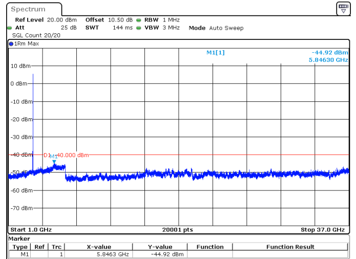
30MHz_15kHz_3565MHz_DFT-s-OFDM QPSK_RB1@159 -44.92 dBm
