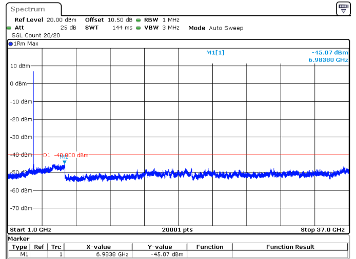
10MHz_15kHz_3695MHz_DFT-s-OFDM QPSK_RB1@51 -45.07 dBm
