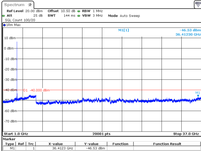
25MHz_30kHz_3562.5MHz_DFT-s-OFDM QPSK_RB1@0 -46.53 dBm
