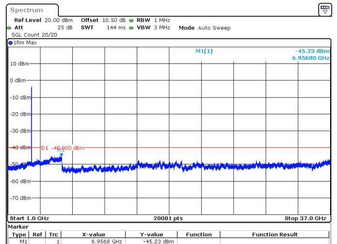
25MHz_30kHz_3625MHz_DFT-s-OFDM QPSK_RB64@0 -45.23 dBm
