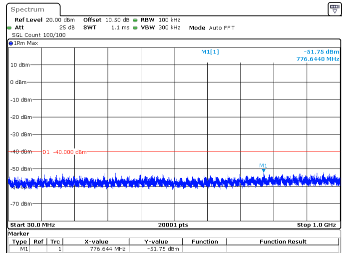
15MHz_15kHz_3557.5MHz_DFT-s-OFDM QPSK_RB1@0 -51.75 dBm
