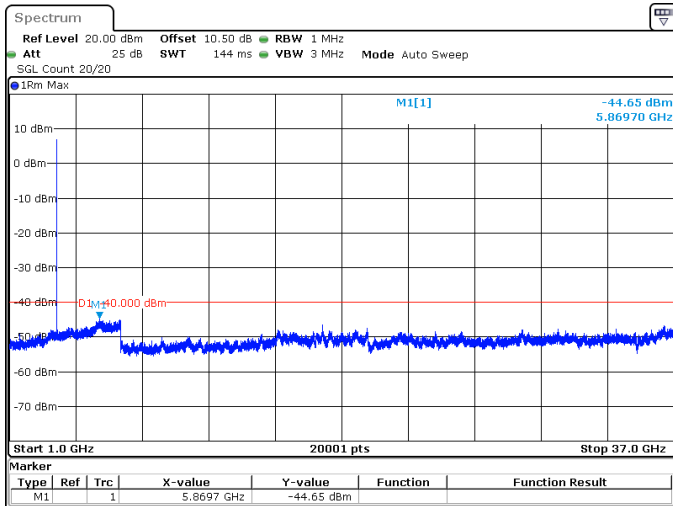
15MHz_30kHz_3557.5MHz_DFT-s-OFDM QPSK_RB1@0 -44.65 dBm
