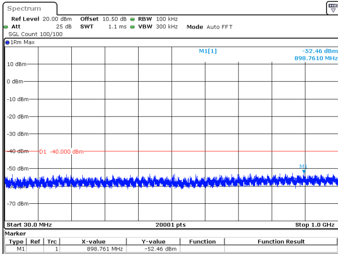
15MHz_30kHz_3625MHz_DFT-s-OFDM QPSK_RB36@0 -52.46 dBm
