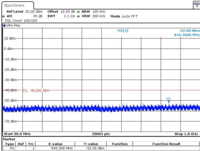
15MHz_30kHz_3692.5MHz_DFT-s-OFDM QPSK_RB1@0 -52.08 dBm
