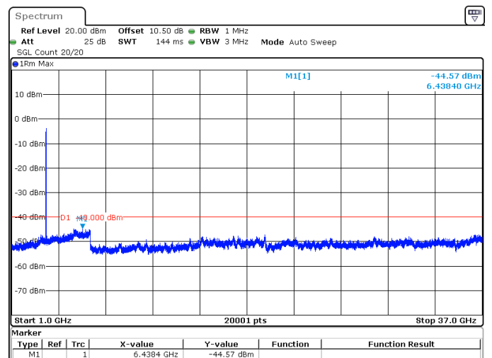
30MHz_15kHz_3625MHz_DFT-s-OFDM QPSK_RB160@0 -44.57 dBm
