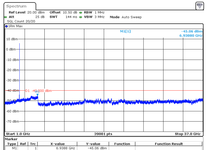
30MHz_15kHz_3625MHz_DFT-s-OFDM QPSK_RB1@159 -45.06 dBm
