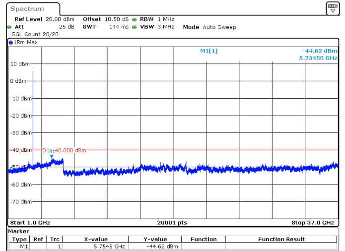
15MHz_30kHz_3692.5MHz_DFT-s-OFDM QPSK_RB1@37 -44.62 dBm
