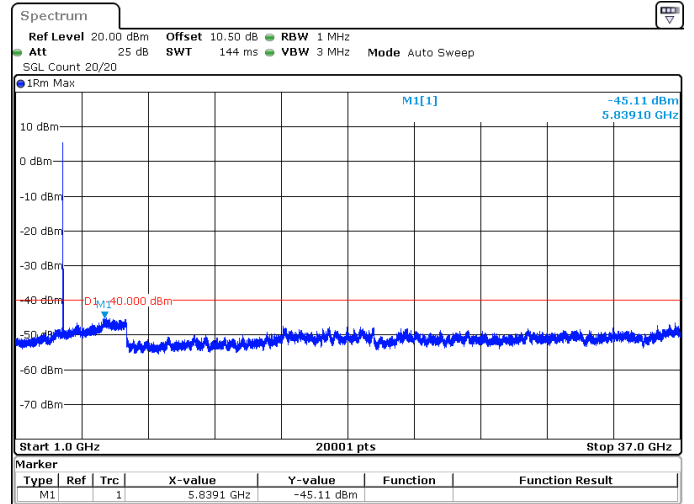
25MHz_30kHz_3562.5MHz_DFT-s-OFDM QPSK_RB1@64 -45.11 dBm
