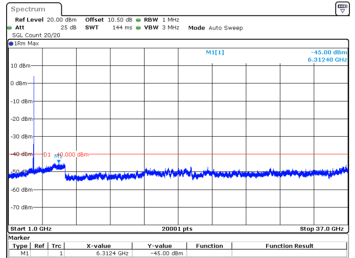
90MHz_30kHz_3625MHz_DFT-s-OFDM QPSK_RB1@244 -45.00 dBm
