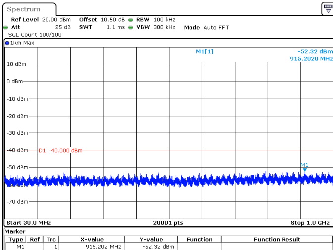
30MHz_15kHz_3565MHz_DFT-s-OFDM QPSK_RB1@159 -52.32 dBm
