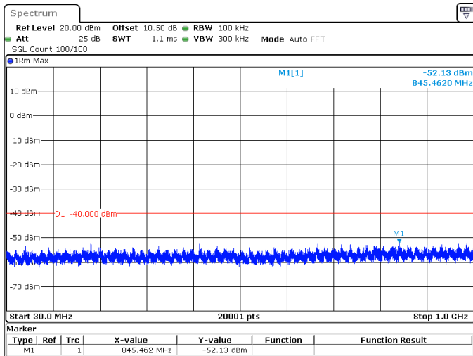
25MHz_15kHz_3625MHz_DFT-s-OFDM QPSK_RB128@0 -52.13 dBm
