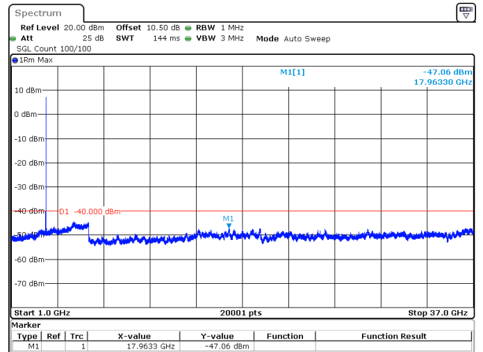
25MHz_15kHz_3687.5MHz_DFT-s-OFDM QPSK_RB1@0 -47.06 dBm
