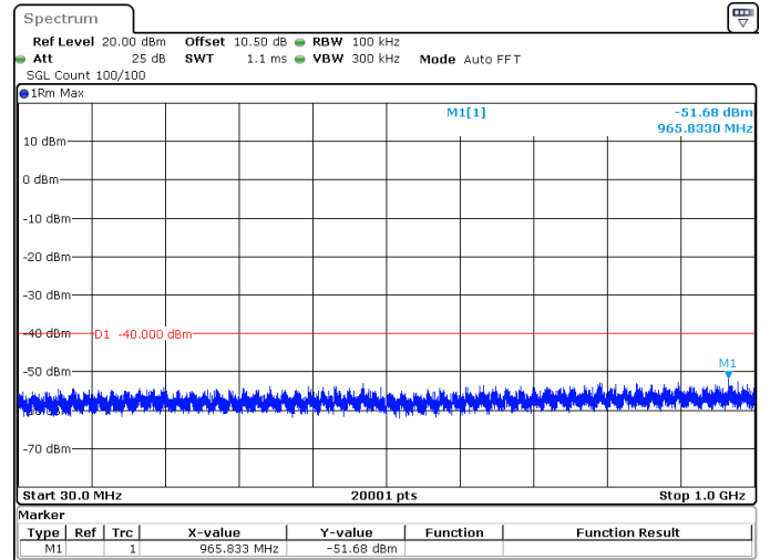
15MHz_30kHz_3557.5MHz_DFT-s-OFDM QPSK_RB1@0 -51.68 dBm
