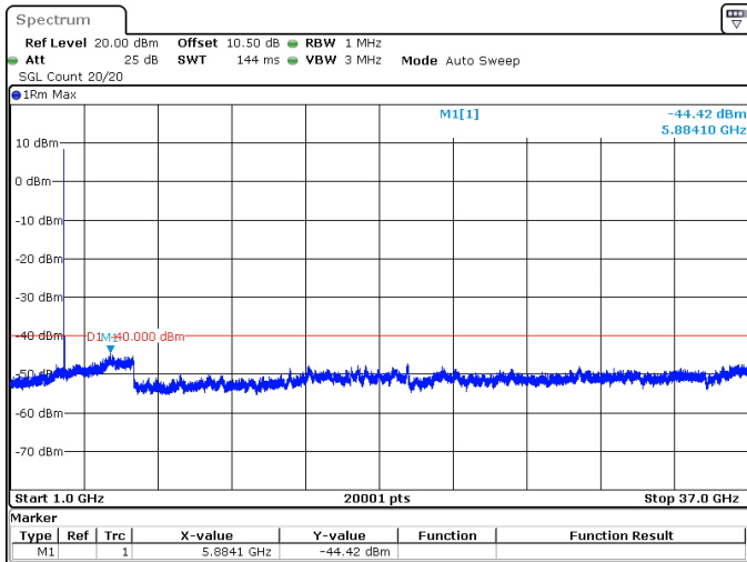
15MHz_15kHz_3625MHz_DFT-s-OFDM QPSK_RB1@0 -44.42 dBm
