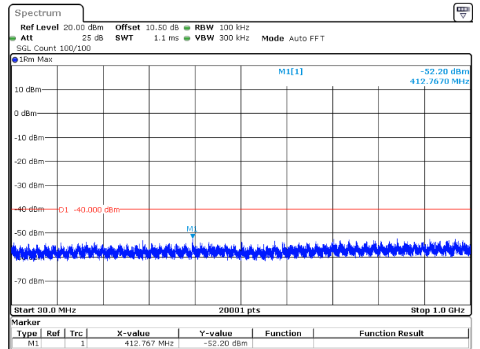
25MHz_15kHz_3625MHz_DFT-s-OFDM QPSK_RB1@0 -52.20 dBm
