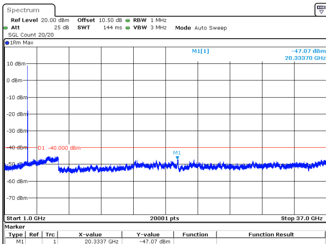
25MHz_15kHz_3562.5MHz_DFT-s-OFDM QPSK_RB1@132 -47.07 dBm
