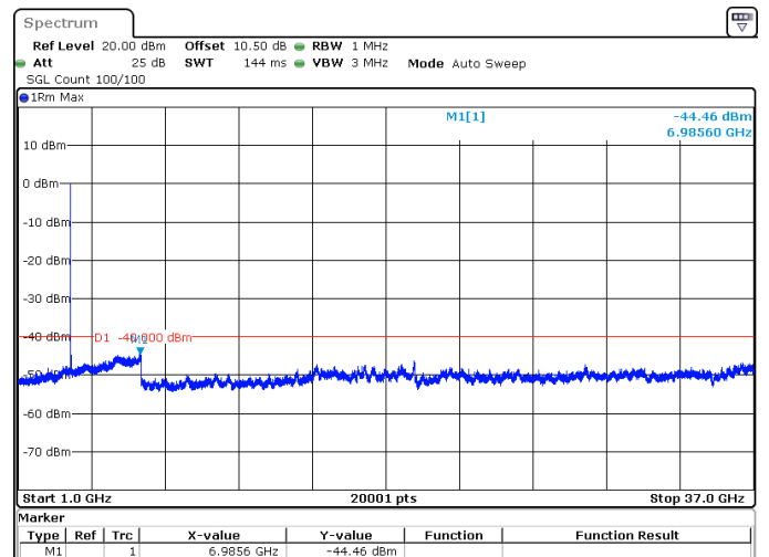
15MHz_30kHz_3557.5MHz_DFT-s-OFDM QPSK_RB36@0 -44.46 dBm
