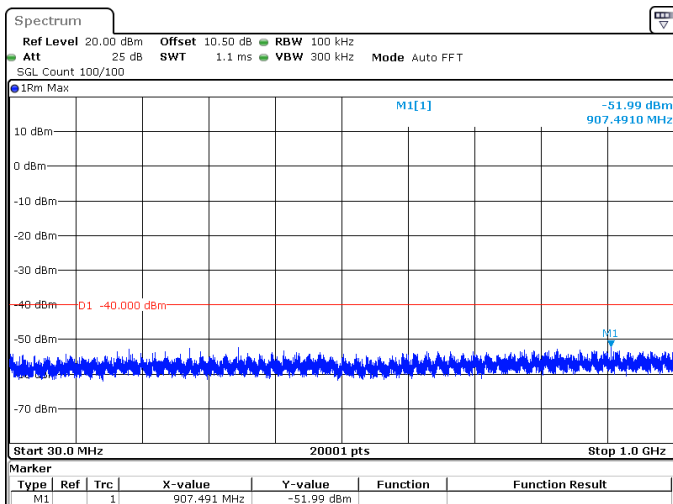
15MHz_15kHz_3625MHz_DFT-s-OFDM QPSK_RB1@78 -51.99 dBm
