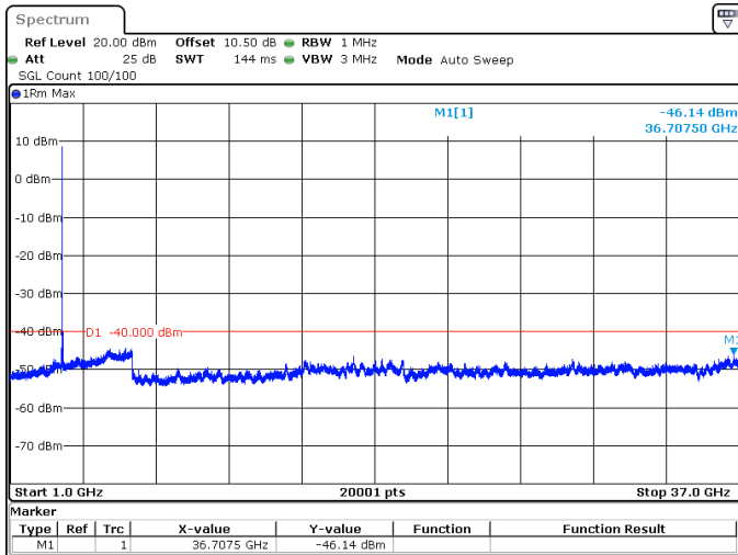
30MHz_15kHz_3565MHz_DFT-s-OFDM QPSK_RB1@0 -46.14 dBm
