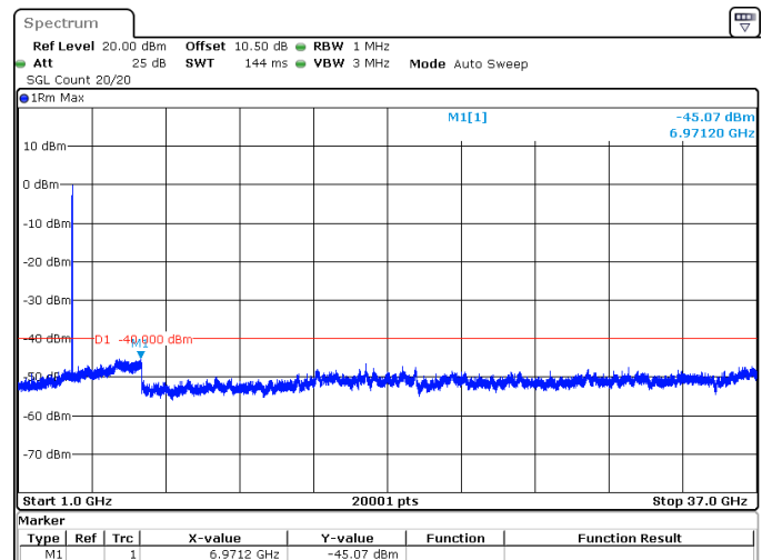
15MHz_30kHz_3625MHz_DFT-s-OFDM QPSK_RB36@0 -45.07 dBm
