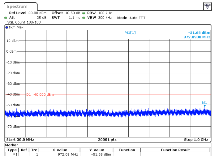
15MHz_30kHz_3692.5MHz_DFT-s-OFDM QPSK_RB36@0 -51.68 dBm
